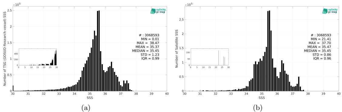
Figure 3: Histograms of SSS from TSG (GOSUD-Research-vessel) (a) and ISAS v7 - Monthly (Ifremer-LOPS-CMEMS) (b) considering all match-up pairs per bins of 0.1 over the North Atlantic Ocean Pi-MEP region and for the full satellite product period.
