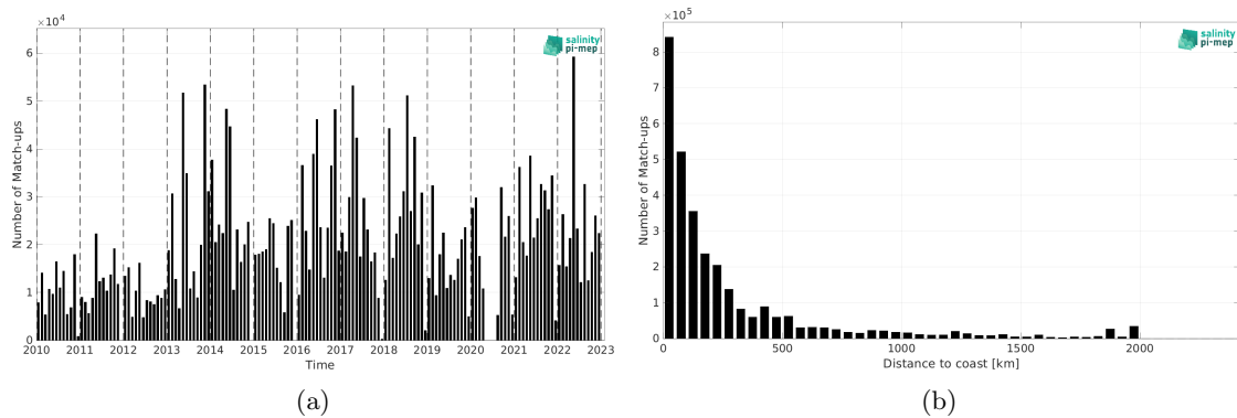
Figure 2: Number of match-ups between TSG (GOSUD-Research-vessel) and ISAS v7 - Monthly (Ifremer-LOPS-CMEMS) SSS as a function of time (a) and as function of the distance to coast (b) over the North Atlantic Ocean Pi-MEP region and for the full satellite product period.
