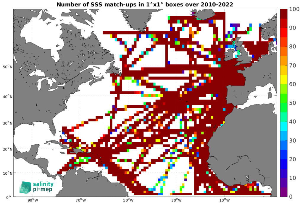
Figure 5: Number of SSS match-ups between TSG (GOSUD-Research-vessel) SSS and the ISAS v7 - Monthly (Ifremer-LOPS-CMEMS) SSS product for the North Atlantic Ocean Pi-MEP region over 1^{\circ} \times 1^{\circ} boxes and for the full satellite product period.
