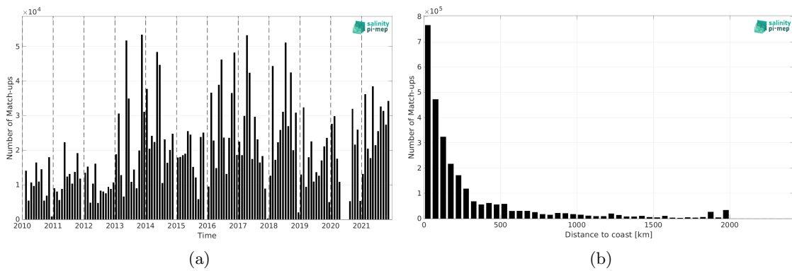
Figure 2: Number of match-ups between TSG (GOSUD-Research-vessel) and ISAS SSS as a function of time (a) and as function of the distance to coast (b) over the North Atlantic Ocean Pi-MEP region and for the full satellite product period.
