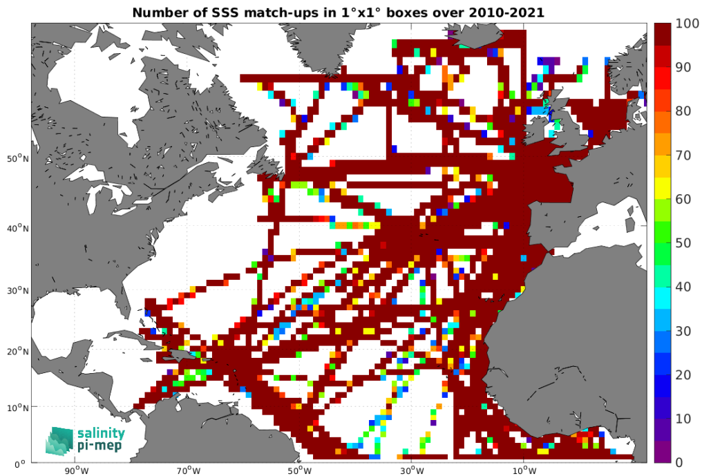
Figure 5: Number of SSS match-ups between TSG (GOSUD-Research-vessel) SSS and the ISAS SSS product for the North Atlantic Ocean Pi-MEP region over 1^{\circ} \times 1^{\circ} boxes and for the full satellite product period.
