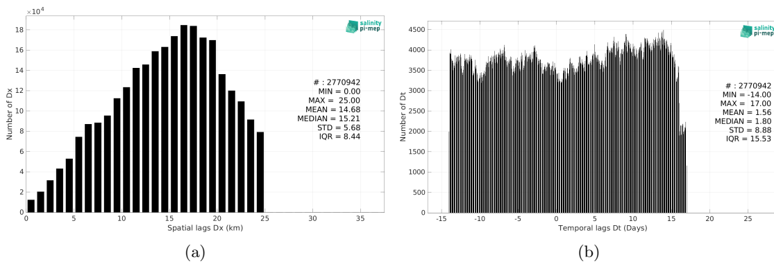
Figure 6: Histograms of the spatial (a) and temporal (b) lags between the location/time of the TSG (GOSUD-Research-vessel) measurement and the date of the corresponding ISAS SSS pixel.
