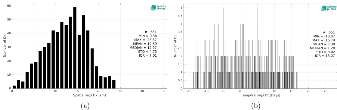
Figure 6: Histograms of the spatial (a) and temporal (b) lags between the location/time of the Marine mammals measurement and the date of the corresponding ISAS v7 - Monthly (Ifremer-LOPS-CMEMS) SSS pixel.
