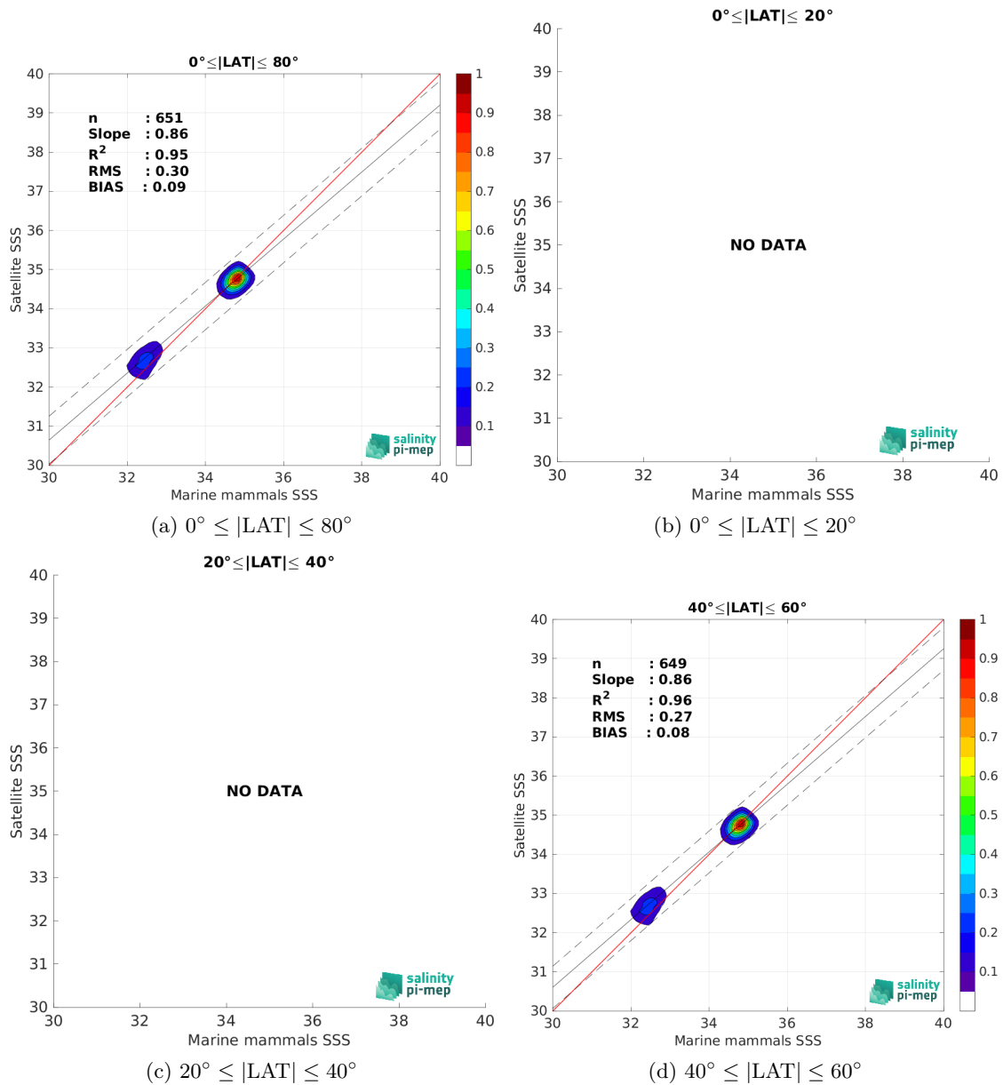
Figure 10: Contour maps of the concentration of ISAS v7 - Monthly (Ifremer-LOPS-CMEMS) SSS (y-axis) versus Marine mammals SSS (x-axis) at match-up pairs for different latitude bands. For each plot, the red line shows x=y . The black thin and dashed lines indicate a linear fit through the data cloud and the \pm 95\% confidence levels, respectively. The number match-up pairs n , the slope and R^2 coefficient of the linear fit, the root mean square (RMS) and the mean bias between satellite and in situ data are indicated for each latitude band in each plots.
