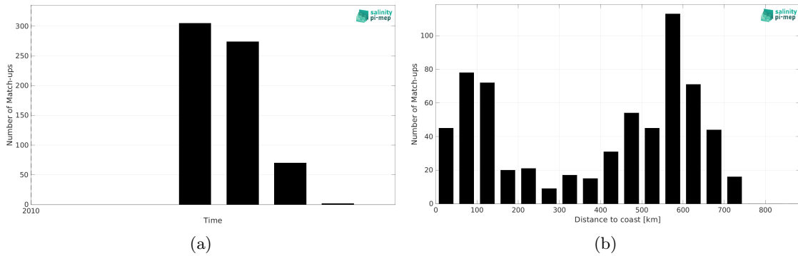
Figure 2: Number of match-ups between Marine mammals and ISAS v7 - Monthly (Ifremer-LOPS-CMEMS) SSS as a function of time (a) and as function of the distance to coast (b) over the North Atlantic Ocean Pi-MEP region and for the full satellite product period.
