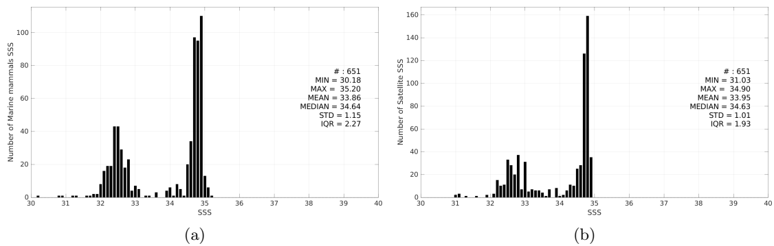
Figure 3: Histograms of SSS from Marine mammals (a) and ISAS v7 - Monthly (Ifremer-LOPS-CMEMS) (b) considering all match-up pairs per bins of 0.1 over the North Atlantic Ocean Pi-MEP region and for the full satellite product period.
