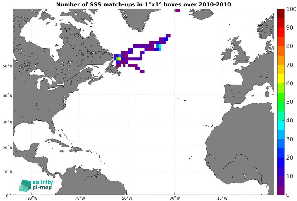
Figure 5: Number of SSS match-ups between Marine mammals SSS and the ISAS v7 - Monthly (Ifremer-LOPS-CMEMS) SSS product for the North Atlantic Ocean Pi-MEP region over 1^\circ \times 1^\circ boxes and for the full satellite product period.
