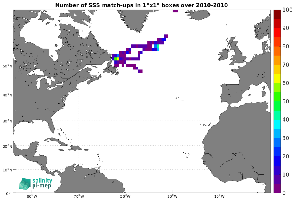
Figure 5: Number of SSS match-ups between Marine mammals SSS and the ISAS SSS product for the North Atlantic Ocean Pi-MEP region over 1^{\circ} \times 1^{\circ} boxes and for the full satellite product period.
