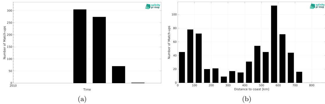
Figure 2: Number of match-ups between Marine mammals and ISAS SSS as a function of time (a) and as function of the distance to coast (b) over the North Atlantic Ocean Pi-MEP region and for the full satellite product period.
