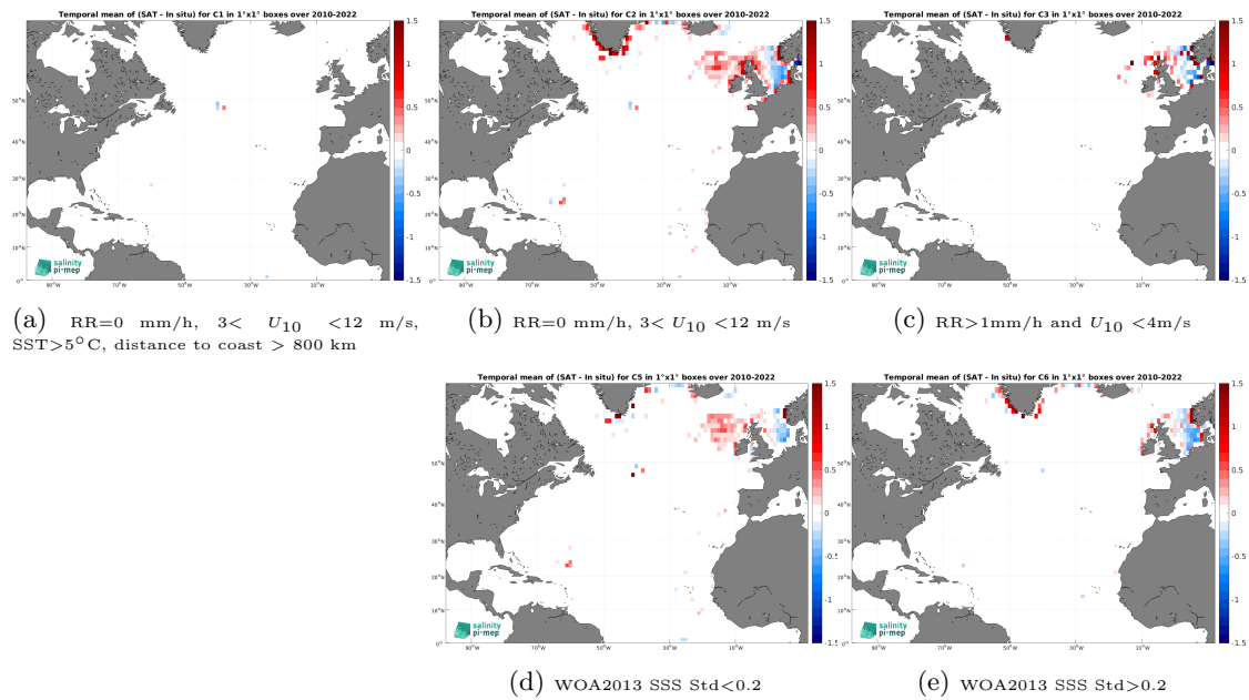
Figure 14: Temporal mean gridded over spatial boxes of size 1^\circ \times 1^\circ of \Delta\text{SSS} (ISAS v7 - Monthly (Ifremer-LOPS-CMEMS) - ICES) for 5 different subdatasets corresponding to:RR=0 mm/h, 3 < U_{10} < 12 m/s, SST > 5°C, distance to coast > 800 km (a), RR=0 mm/h, 3 < U_{10} < 12 m/s (b), RR > 1mm/h and U_{10} < 4 m/s (c), WOA2013 SSS Std < 0.2 (d), WOA2013 SSS Std > 0.2 (e).
