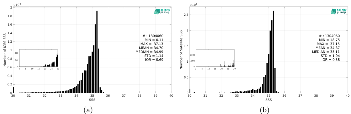
Figure 3: Histograms of SSS from ICES (a) and ISAS v7 - Monthly (Ifremer-LOPS-CMEMS) (b) considering all match-up pairs per bins of 0.1 over the North Atlantic Ocean Pi-MEP region and for the full satellite product period.
