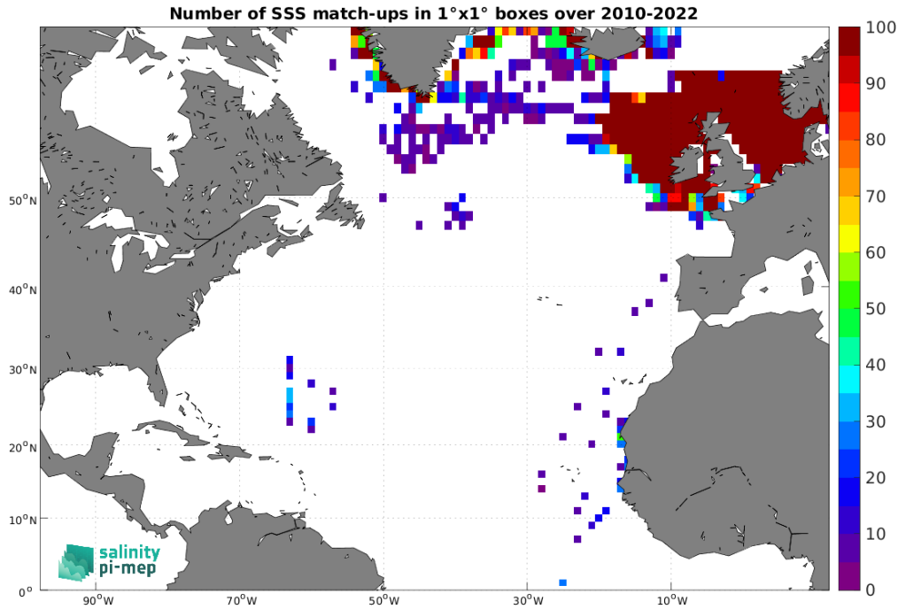
Figure 5: Number of SSS match-ups between ICES SSS and the ISAS v7 - Monthly (Ifremer-LOPS-CMEMS) SSS product for the North Atlantic Ocean Pi-MEP region over 1^\circ \times 1^\circ boxes and for the full satellite product period.
