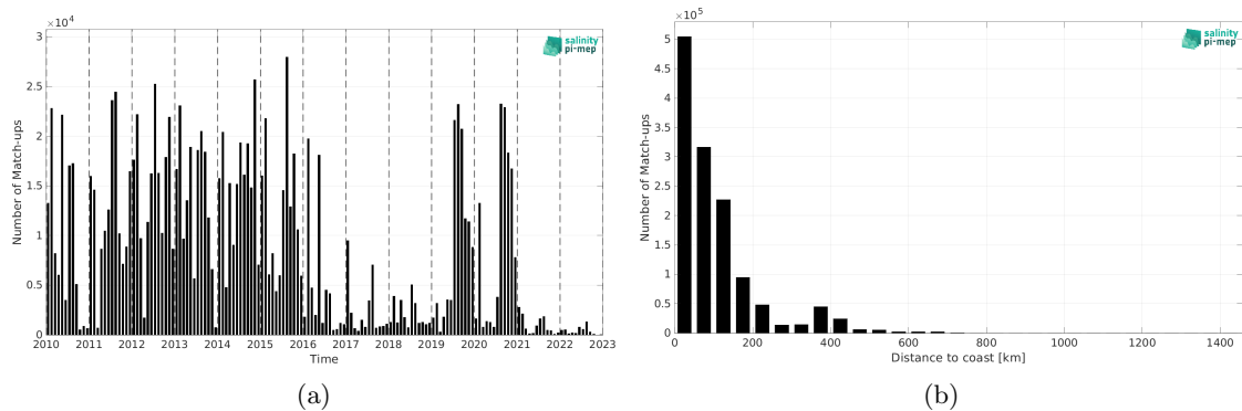
Figure 2: Number of match-ups between ICES and ISAS v7 - Monthly (Ifremer-LOPS-CMEMS) SSS as a function of time (a) and as function of the distance to coast (b) over the North Atlantic Ocean Pi-MEP region and for the full satellite product period.
