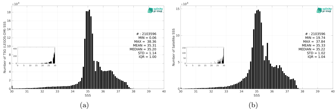
Figure 3: Histograms of SSS from TSG (LEGOS-DM) (a) and CCI SSS L4 Merged-OI v5.5 - 7-day running (ESA) (b) considering all match-up pairs per bins of 0.1 over the North Atlantic Ocean Pi-MEP region and for the full satellite product period.
