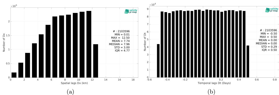
Figure 6: Histograms of the spatial (a) and temporal (b) lags between the location/time of the TSG (LEGOS-DM) measurement and the date of the corresponding CCI SSS L4 Merged-OI v5.5 - 7-day running (ESA) SSS pixel.
