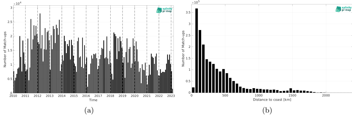
Figure 2: Number of match-ups between TSG (LEGOS-DM) and CCI SSS L4 Merged-OI v5.5 - 7-day running (ESA) SSS as a function of time (a) and as function of the distance to coast (b) over the North Atlantic Ocean Pi-MEP region and for the full satellite product period.
