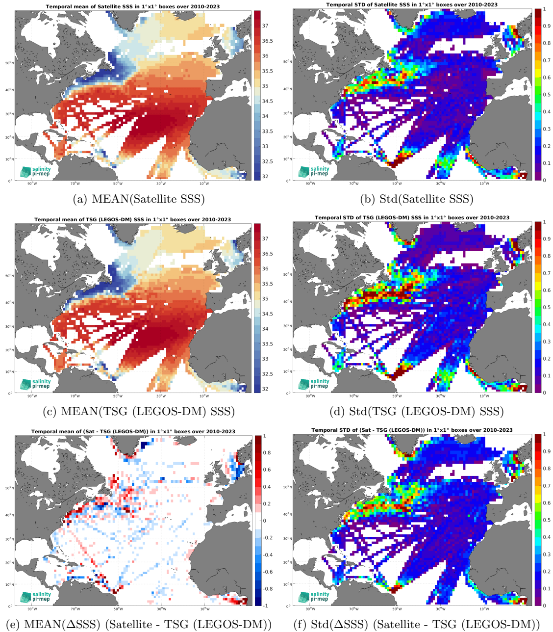
Figure 7: Temporal mean (left) and Std (right) of SSS from CCI SSS L4 Merged-OI v5.5 - 7-day running (ESA) (top), TSG (LEGOS-DM) (middle), and of \Delta SSS (Satellite - TSG (LEGOS-DM)). Only match-up pairs are used to generate these maps.
