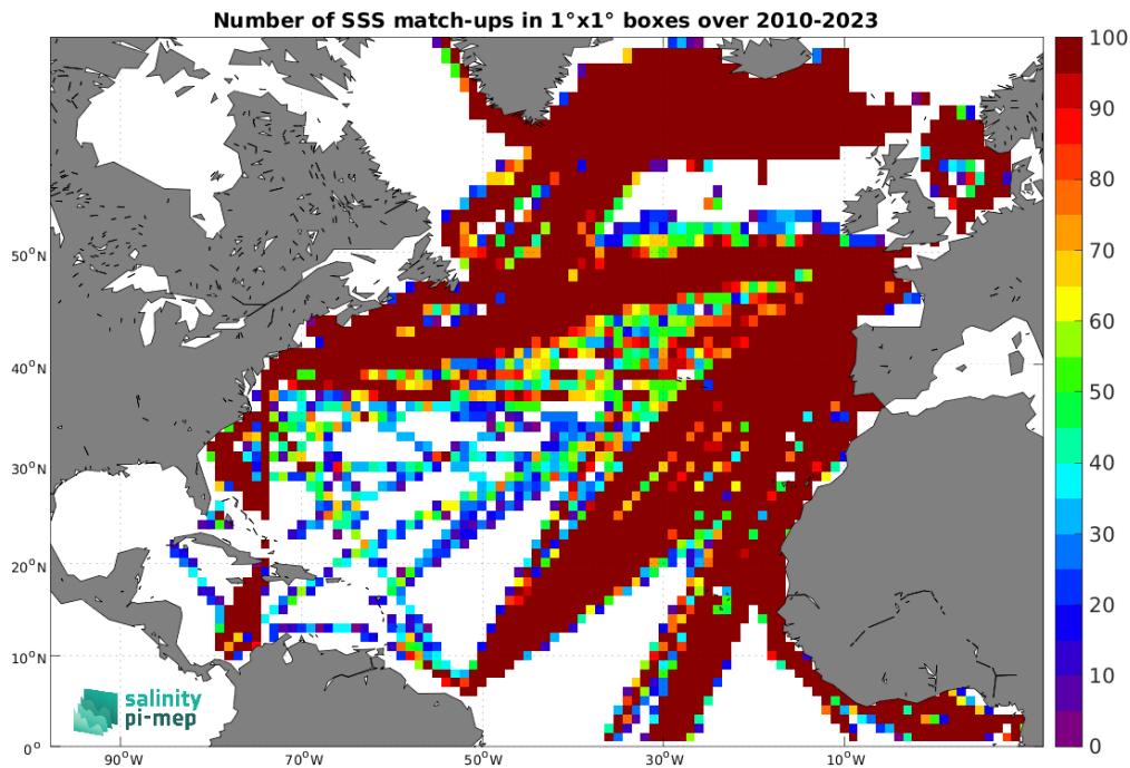
Figure 5: Number of SSS match-ups between TSG (LEGOS-DM) SSS and the CCI SSS L4 Merged-OI v5.5 - 7-day running (ESA) SSS product for the North Atlantic Ocean Pi-MEP region over 1^\circ \times 1^\circ boxes and for the full satellite product period.
