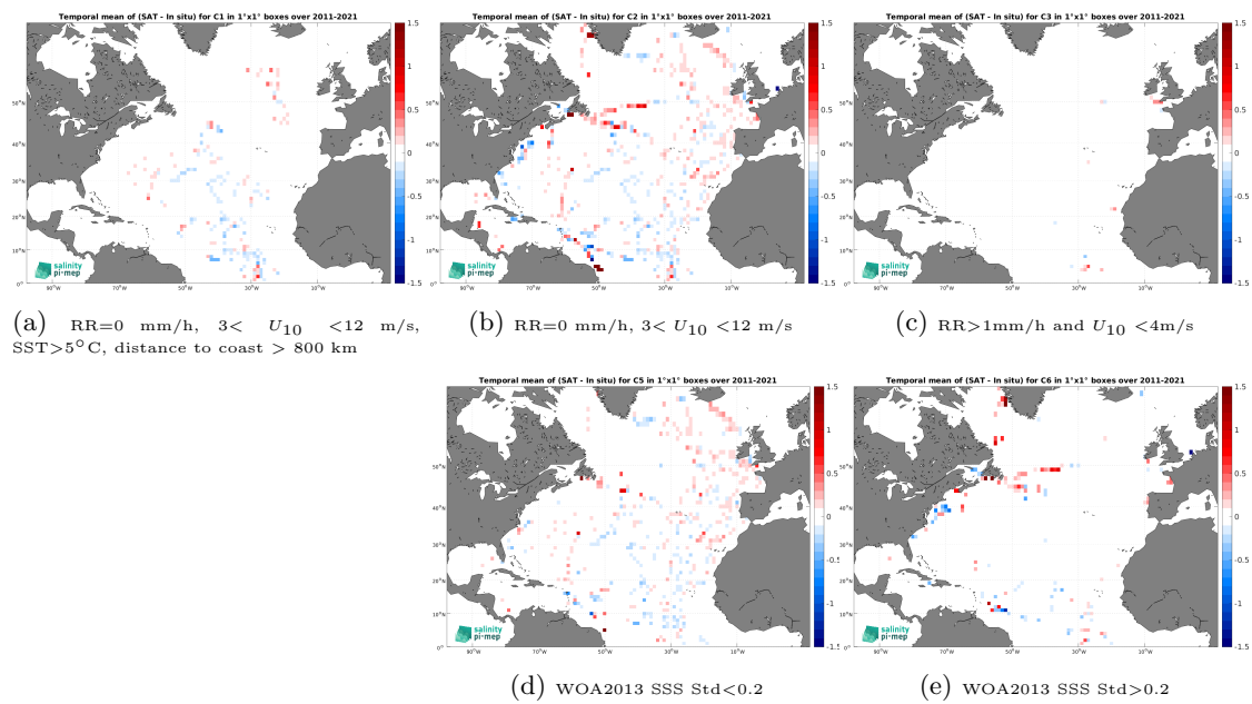
Figure 14: Temporal mean gridded over spatial boxes of size 1^\circ \times 1^\circ of \Delta\text{SSS} (CCI SSS L4 Merged-OI v5.5 - 7-day running (ESA) - TSG (GOSUD-Sailing-ship)) for 5 different subdatasets corresponding to:RR=0 mm/h, 3 < U_{10} < 12 m/s, SST >5^\circ\text{C} , distance to coast > 800 km (a), RR=0 mm/h, 3 < U_{10} < 12 m/s (b), RR >1 mm/h and U_{10} < 4 m/s (c), WOA2013 SSS Std <0.2 (d), WOA2013 SSS Std >0.2 (e).
