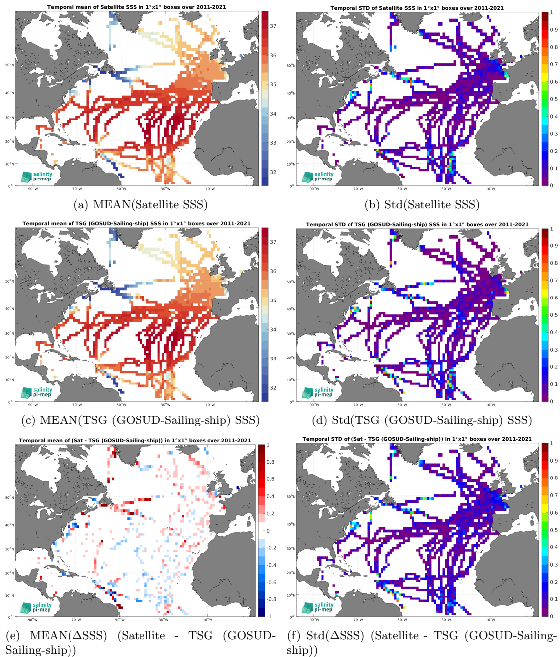
Figure 7: Temporal mean (left) and Std (right) of SSS from CCI SSS L4 Merged-OI v5.5 - 7-day running (ESA) (top), TSG (GOSUD-Sailing-ship) (middle), and of \Delta SSS (Satellite - TSG (GOSUD-Sailing-ship)). Only match-up pairs are used to generate these maps.
