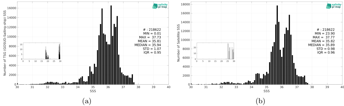
Figure 3: Histograms of SSS from TSG (GOSUD-Sailing-ship) (a) and CCI SSS L4 Merged-OI v5.5 - 7-day running (ESA) (b) considering all match-up pairs per bins of 0.1 over the North Atlantic Ocean Pi-MEP region and for the full satellite product period.
