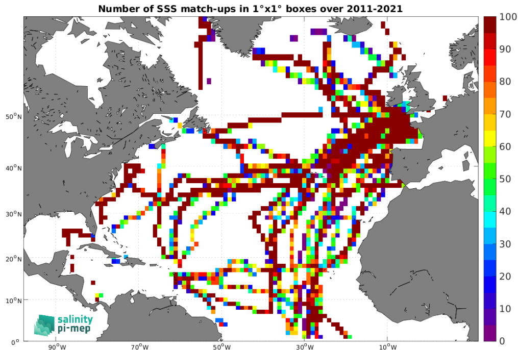
Figure 5: Number of SSS match-ups between TSG (GOSUD-Sailing-ship) SSS and the CCI SSS L4 Merged-OI v5.5 - 7-day running (ESA) SSS product for the North Atlantic Ocean Pi-MEP region over 1^\circ \times 1^\circ boxes and for the full satellite product period.
