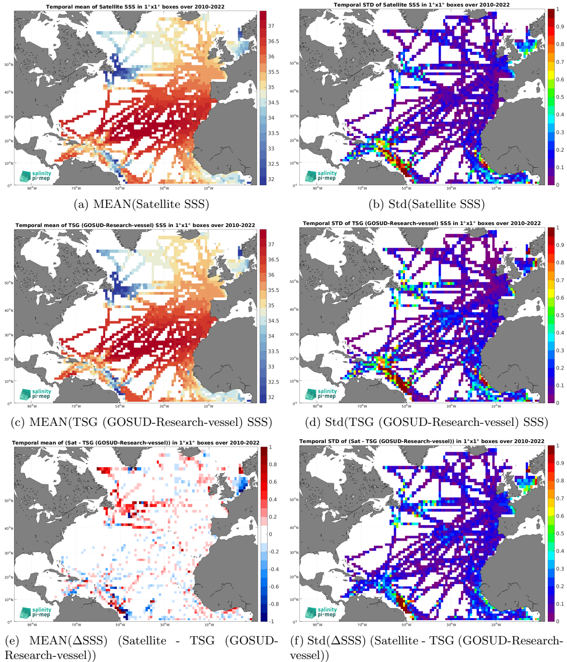
Figure 7: Temporal mean (left) and Std (right) of SSS from CCI SSS L4 Merged-OI v5.5 - 7-day running (ESA) (top), TSG (GOSUD-Research-vessel) (middle), and of \Delta SSS (Satellite - TSG (GOSUD-Research-vessel)). Only match-up pairs are used to generate these maps.
