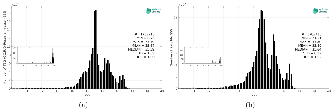
Figure 3: Histograms of SSS from TSG (GOSUD-Research-vessel) (a) and CCI SSS L4 Merged-OI v5.5 - 7-day running (ESA) (b) considering all match-up pairs per bins of 0.1 over the North Atlantic Ocean Pi-MEP region and for the full satellite product period.
