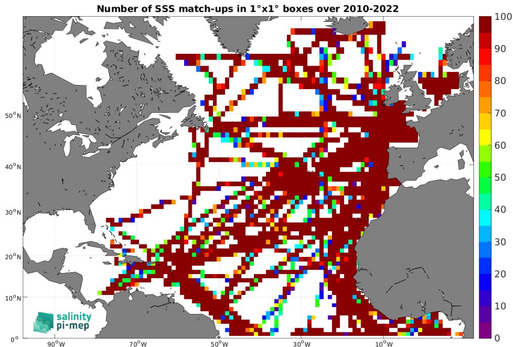
Figure 5: Number of SSS match-ups between TSG (GOSUD-Research-vessel) SSS and the CCI SSS L4 Merged-OI v5.5 - 7-day running (ESA) SSS product for the North Atlantic Ocean Pi-MEP region over 1^\circ \times 1^\circ boxes and for the full satellite product period.
