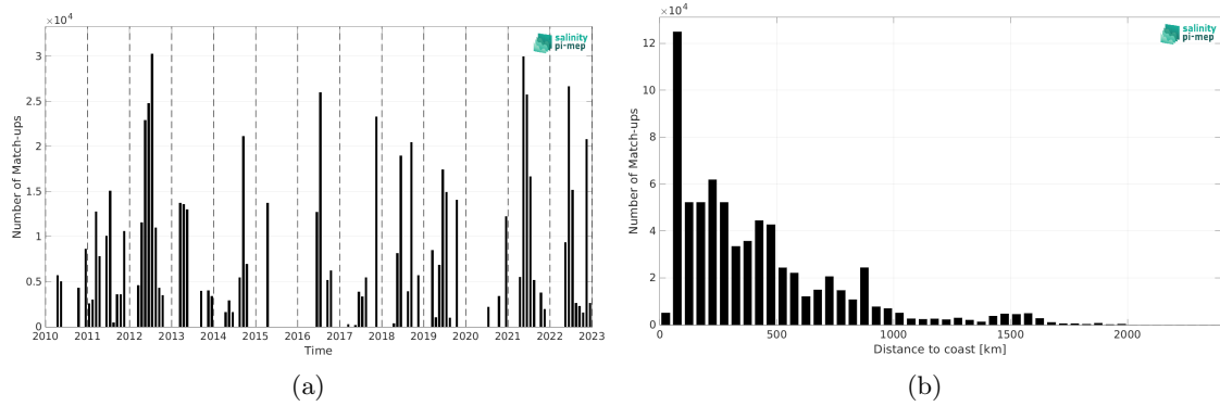
Figure 2: Number of match-ups between TSG (CSIC-UTM) and CCI SSS L4 Merged-OI v5.5 - 7-day running (ESA) SSS as a function of time (a) and as function of the distance to coast (b) over the North Atlantic Ocean Pi-MEP region and for the full satellite product period.
