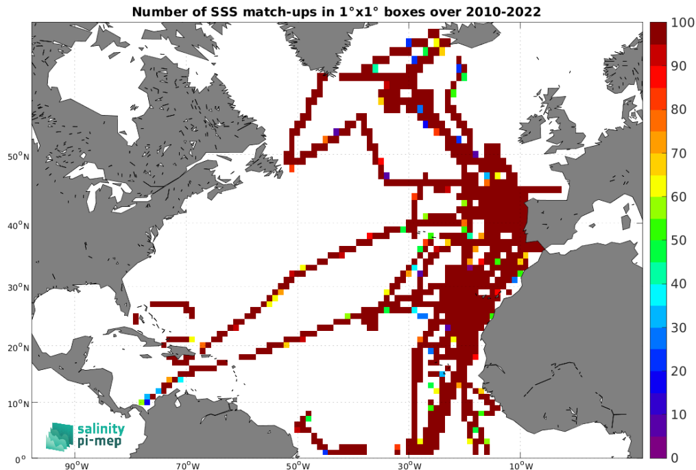
Figure 5: Number of SSS match-ups between TSG (CSIC-UTM) SSS and the CCI SSS L4 Merged-OI v5.5 - 7-day running (ESA) SSS product for the North Atlantic Ocean Pi-MEP region over 1^\circ \times 1^\circ boxes and for the full satellite product period.
