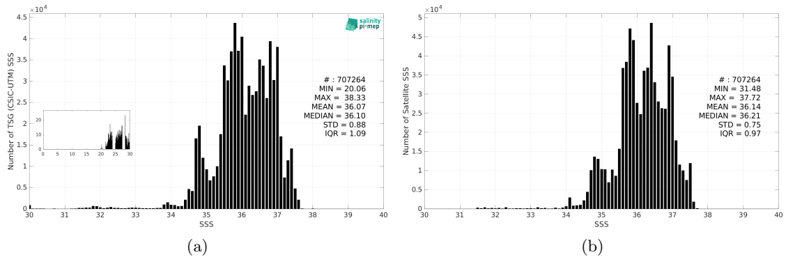
Figure 3: Histograms of SSS from TSG (CSIC-UTM) (a) and CCI SSS L4 Merged-OI v5.5 - 7-day running (ESA) (b) considering all match-up pairs per bins of 0.1 over the North Atlantic Ocean Pi-MEP region and for the full satellite product period.
