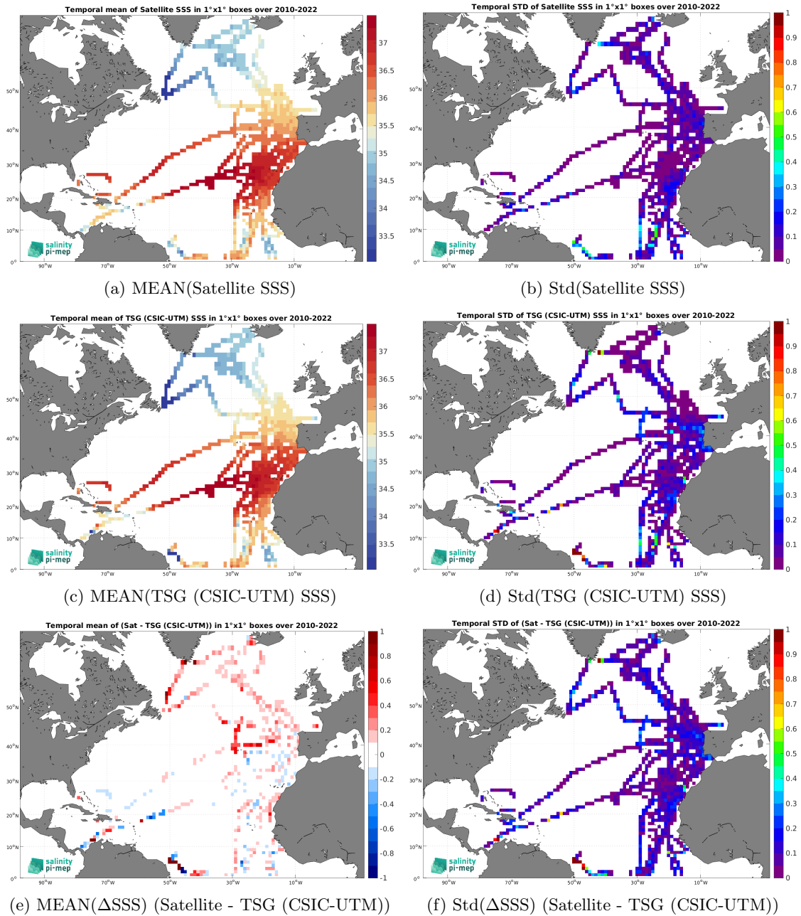
Figure 7: Temporal mean (left) and Std (right) of SSS from CCI SSS L4 Merged-OI v5.5 - 7-day running (ESA) (top), TSG (CSIC-UTM) (middle), and of \Delta SSS (Satellite - TSG (CSIC-UTM)). Only match-up pairs are used to generate these maps.
