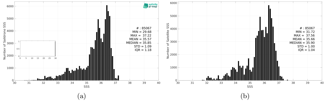
Figure 3: Histograms of SSS from Saildrone (a) and CCI SSS L4 Merged-OI v5.5 - 7-day running (ESA) (b) considering all match-up pairs per bins of 0.1 over the North Atlantic Ocean Pi-MEP region and for the full satellite product period.
