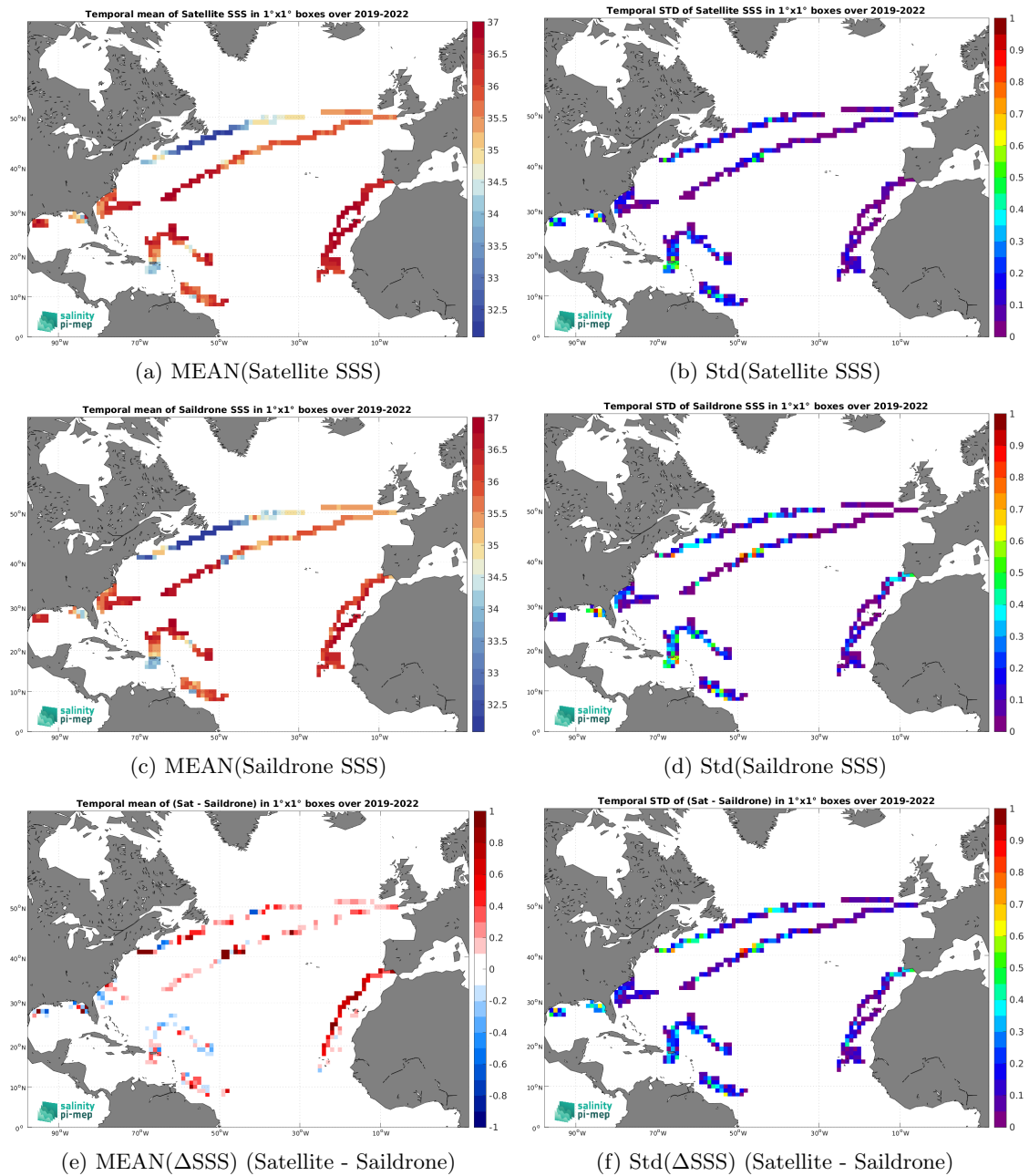
Figure 7: Temporal mean (left) and Std (right) of SSS from CCI SSS L4 Merged-OI v5.5 - 7-day running (ESA) (top), Saildrone (middle), and of \Delta SSS (Satellite - Saildrone). Only match-up pairs are used to generate these maps.
