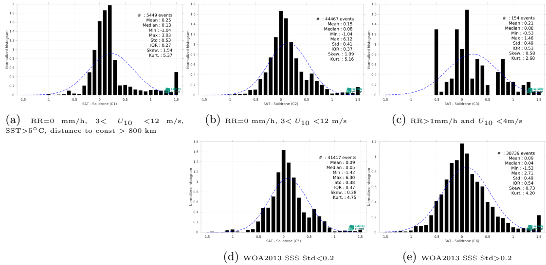
Figure 15: Normalized histogram of \Delta SSS (CCI SSS L4 Merged-OI v5.5 - 7-day running (ESA) - Saildrone) for 5 different subdatasets corresponding to: RR=0 mm/h, 3 < U_{10} < 12 m/s, SST>5°C, distance to coast > 800 km (a), RR=0 mm/h, 3 < U_{10} < 12 m/s (b), RR>1mm/h and U_{10} < 4 m/s (c), WOA2013 SSS Std<0.2 (d), WOA2013 SSS Std>0.2 (e).
