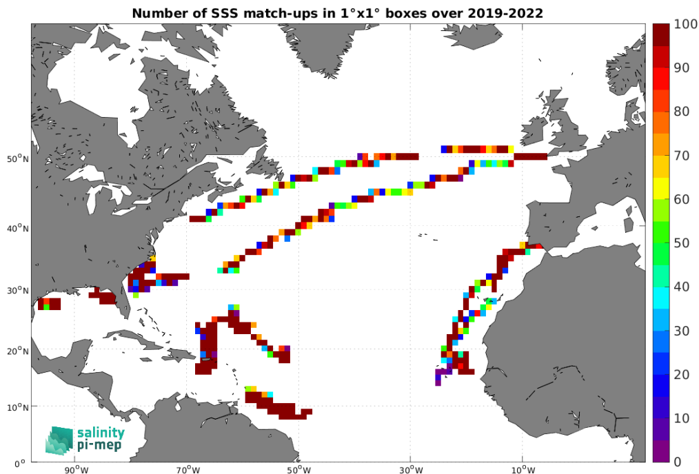
Figure 5: Number of SSS match-ups between Saildrone SSS and the CCI SSS L4 Merged-OI v5.5 - 7-day running (ESA) SSS product for the North Atlantic Ocean Pi-MEP region over 1^\circ \times 1^\circ boxes and for the full satellite product period.
