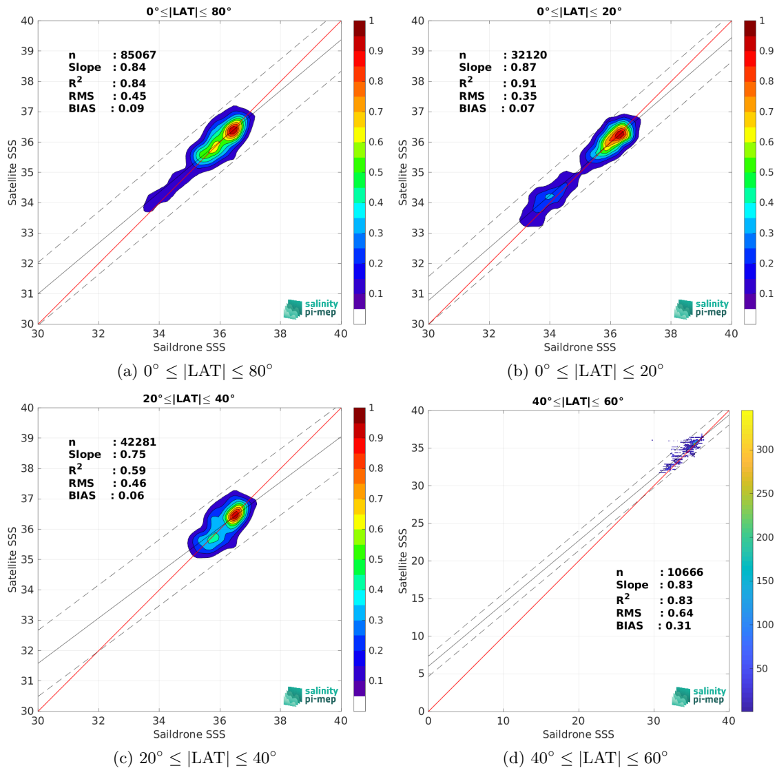
Figure 10: Contour maps of the concentration of CCI SSS L4 Merged-OI v5.5 - 7-day running (ESA) SSS (y-axis) versus Saildrone SSS (x-axis) at match-up pairs for different latitude bands. For each plot, the red line shows x=y . The black thin and dashed lines indicate a linear fit through the data cloud and the \pm 95\% confidence levels, respectively. The number match-up pairs n , the slope and R^2 coefficient of the linear fit, the root mean square (RMS) and the mean bias between satellite and in situ data are indicated for each latitude band in each plots.
