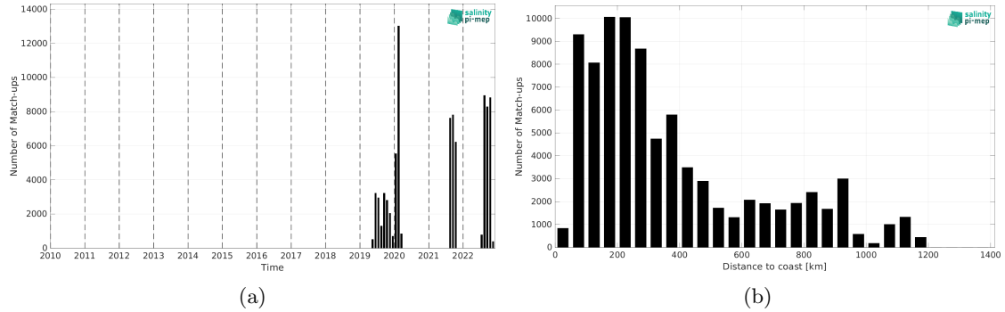
Figure 2: Number of match-ups between Saildrone and CCI SSS L4 Merged-OI v5.5 - 7-day running (ESA) SSS as a function of time (a) and as function of the distance to coast (b) over the North Atlantic Ocean Pi-MEP region and for the full satellite product period.
