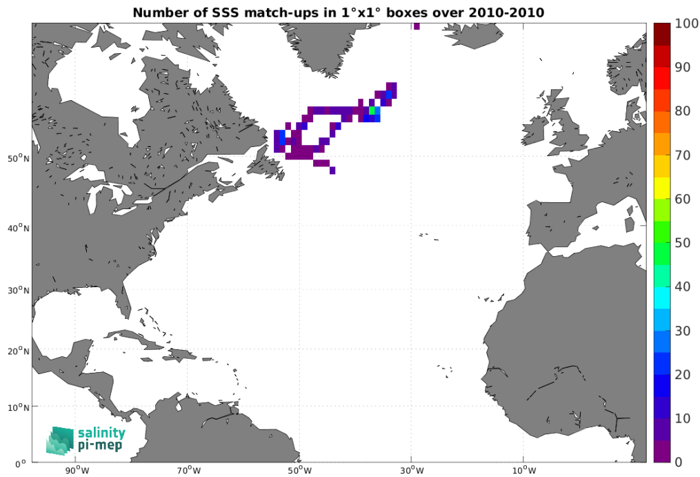
Figure 5: Number of SSS match-ups between Marine mammals SSS and the CCI SSS L4 Merged-OI v5.5 - 7-day running (ESA) SSS product for the North Atlantic Ocean Pi-MEP region over 1^\circ \times 1^\circ boxes and for the full satellite product period.
