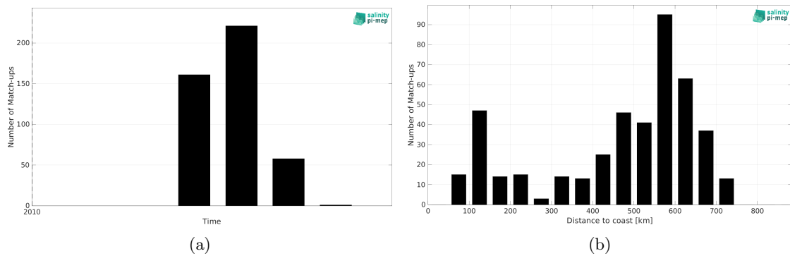
Figure 2: Number of match-ups between Marine mammals and CCI SSS L4 Merged-OI v5.5 - 7-day running (ESA) SSS as a function of time (a) and as function of the distance to coast (b) over the North Atlantic Ocean Pi-MEP region and for the full satellite product period.
