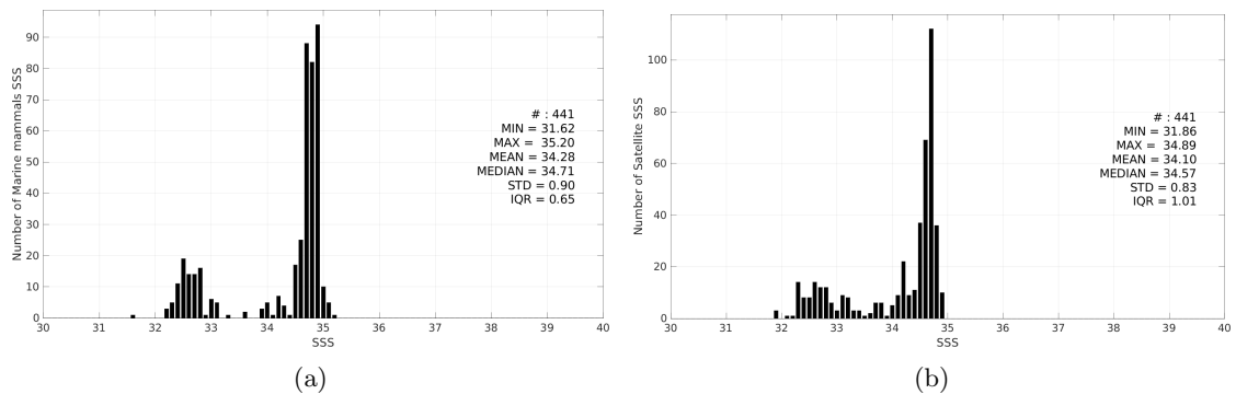
Figure 3: Histograms of SSS from Marine mammals (a) and CCI SSS L4 Merged-OI v5.5 - 7-day running (ESA) (b) considering all match-up pairs per bins of 0.1 over the North Atlantic Ocean Pi-MEP region and for the full satellite product period.
