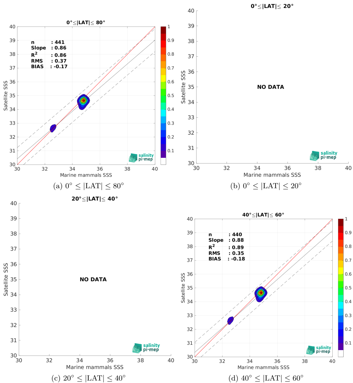
Figure 10: Contour maps of the concentration of CCI SSS L4 Merged-OI v5.5 - 7-day running (ESA) SSS (y-axis) versus Marine mammals SSS (x-axis) at match-up pairs for different latitude bands. For each plot, the red line shows x=y . The black thin and dashed lines indicate a linear fit through the data cloud and the \pm 95\% confidence levels, respectively. The number match-up pairs n , the slope and R^2 coefficient of the linear fit, the root mean square (RMS) and the mean bias between satellite and in situ data are indicated for each latitude band in each plots.
