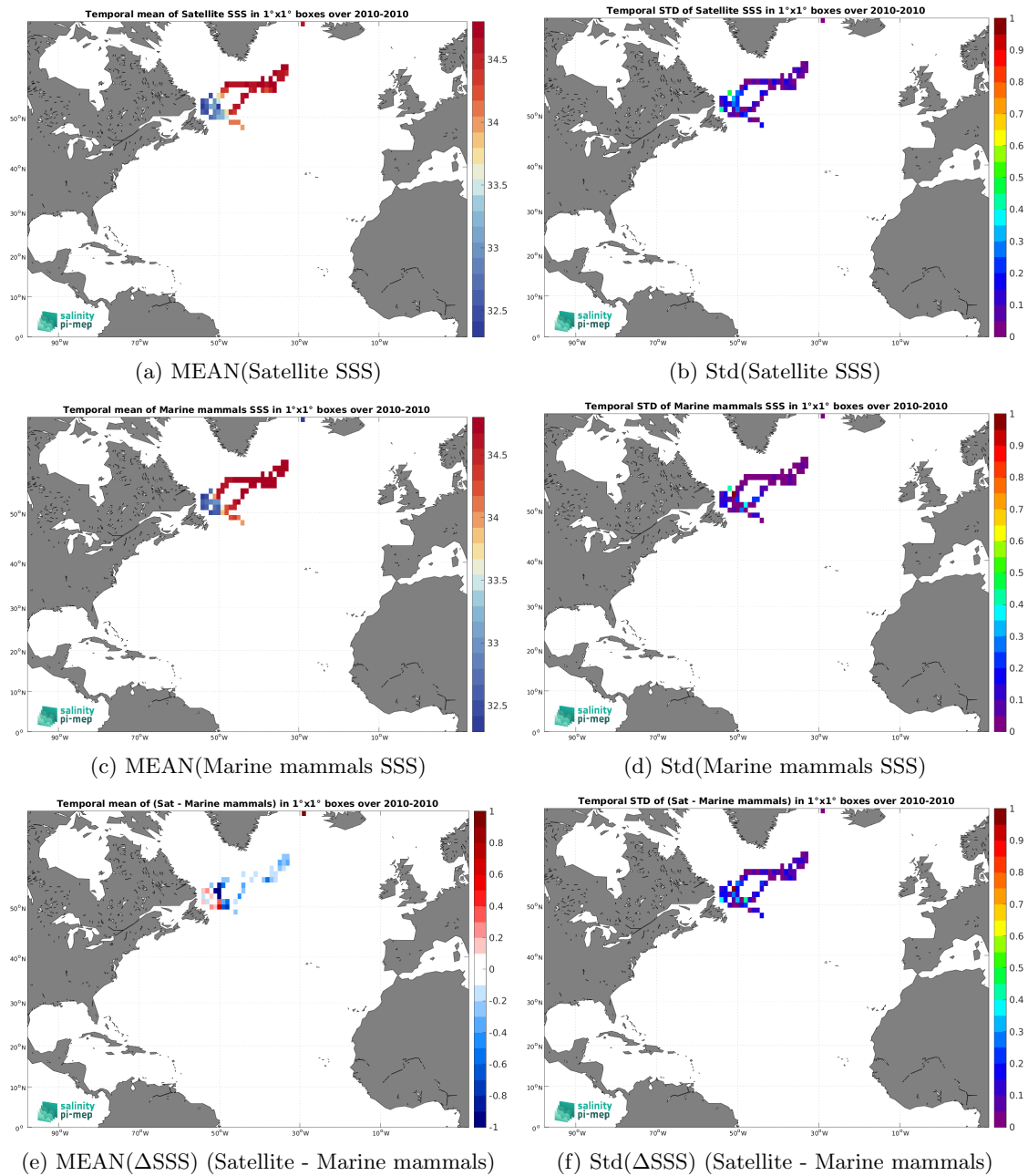
Figure 7: Temporal mean (left) and Std (right) of SSS from CCI SSS L4 Merged-OI v5.5 - 7-day running (ESA) (top), Marine mammals (middle), and of \Delta SSS (Satellite - Marine mammals). Only match-up pairs are used to generate these maps.
