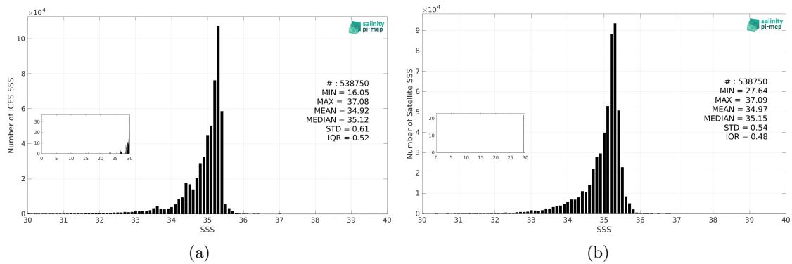
Figure 3: Histograms of SSS from ICES (a) and CCI SSS L4 Merged-OI v5.5 - 7-day running (ESA) (b) considering all match-up pairs per bins of 0.1 over the North Atlantic Ocean Pi-MEP region and for the full satellite product period.
