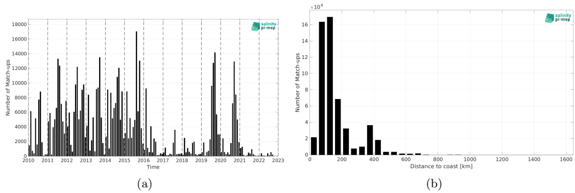
Figure 2: Number of match-ups between ICES and CCI SSS L4 Merged-OI v5.5 - 7-day running (ESA) SSS as a function of time (a) and as function of the distance to coast (b) over the North Atlantic Ocean Pi-MEP region and for the full satellite product period.
