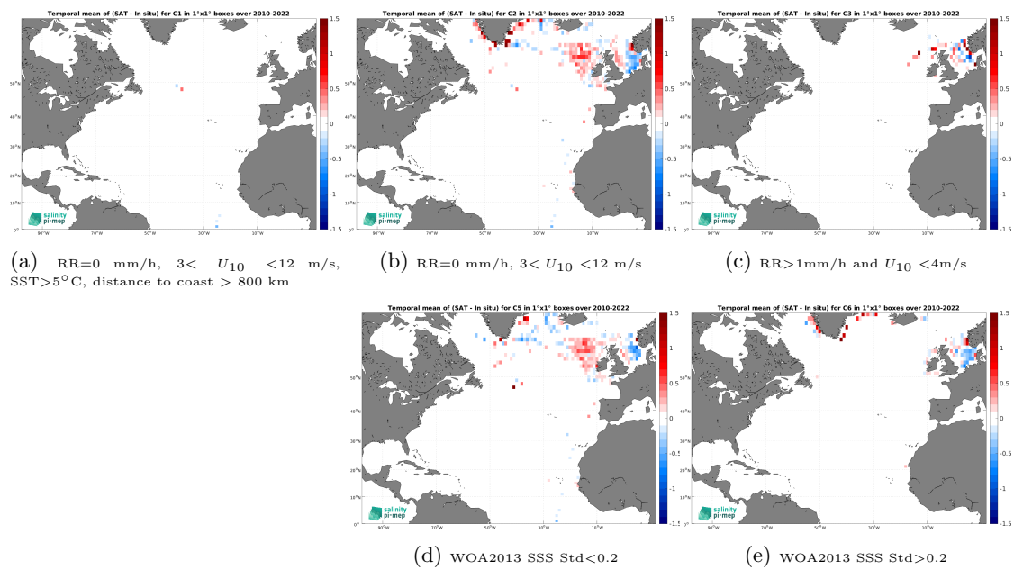
Figure 14: Temporal mean gridded over spatial boxes of size 1^\circ \times 1^\circ of \Delta\text{SSS} (CCI SSS L4 Merged-OI v5.5 - 7-day running (ESA) - ICES) for 5 different subdatasets corresponding to:RR=0 mm/h, 3 < U_{10} < 12 m/s, SST >5^\circ\text{C} , distance to coast > 800 km (a), RR=0 mm/h, 3 < U_{10} < 12 m/s (b), RR >1 mm/h and U_{10} < 4 m/s (c), WOA2013 SSS Std <0.2 (d), WOA2013 SSS Std >0.2 (e).
