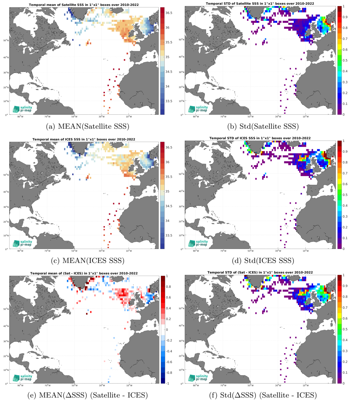
Figure 7: Temporal mean (left) and Std (right) of SSS from CCI SSS L4 Merged-OI v5.5 - 7-day running (ESA) (top), ICES (middle), and of \Delta SSS (Satellite - ICES). Only match-up pairs are used to generate these maps.
