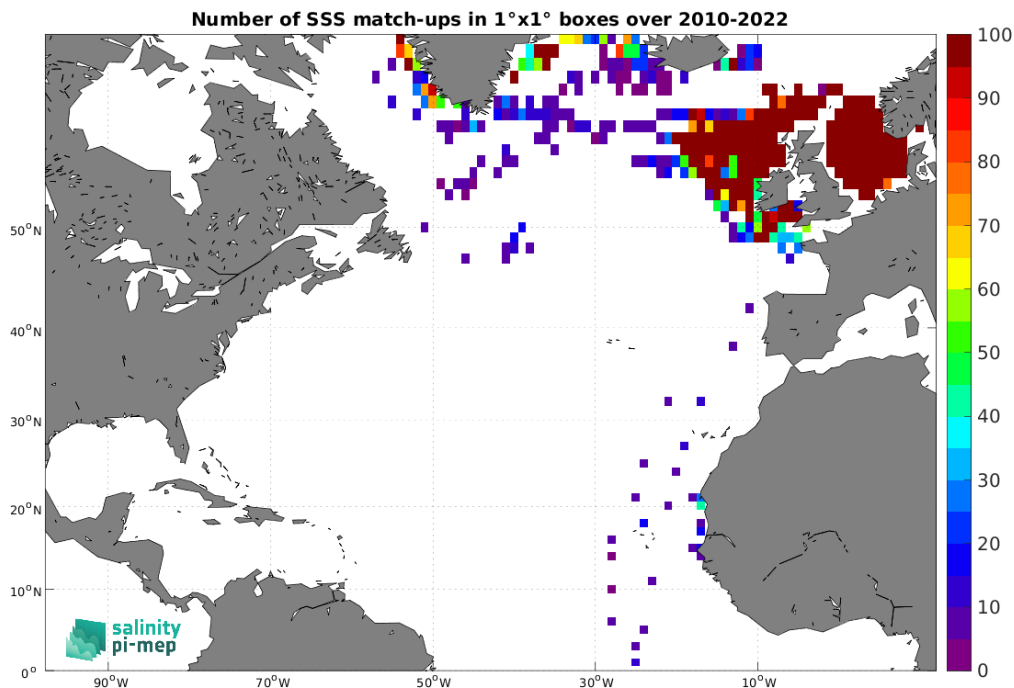
Figure 5: Number of SSS match-ups between ICES SSS and the CCI SSS L4 Merged-OI v5.5 - 7-day running (ESA) SSS product for the North Atlantic Ocean Pi-MEP region over 1^\circ \times 1^\circ boxes and for the full satellite product period.
