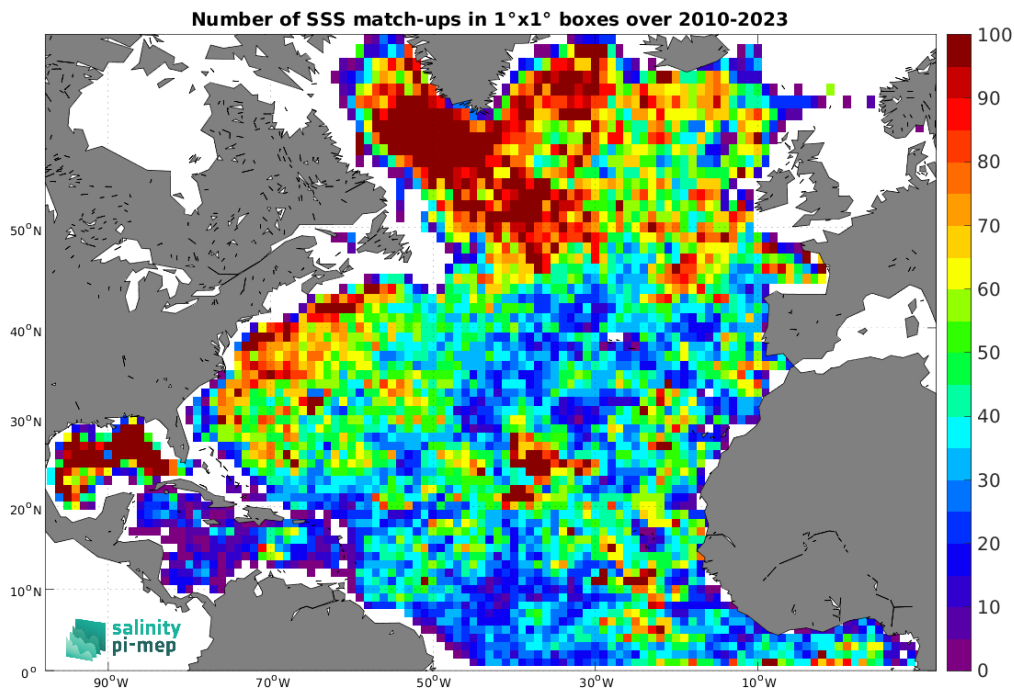
Figure 5: Number of SSS match-ups between Argo SSS and the CCI SSS L4 Merged-OI v5.5 - 7-day running (ESA) SSS product for the North Atlantic Ocean Pi-MEP region over 1^\circ \times 1^\circ boxes and for the full satellite product period.
