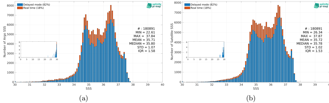
Figure 3: Histograms of SSS from Argo (a) and CCI SSS L4 Merged-OI v5.5 - 7-day running (ESA) (b) considering all match-up pairs per bins of 0.1 over the North Atlantic Ocean Pi-MEP region and for the full satellite product period.
