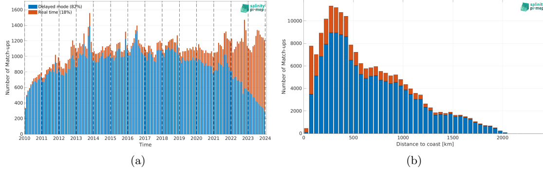
Figure 2: Number of match-ups between Argo and CCI SSS L4 Merged-OI v5.5 - 7-day running (ESA) SSS as a function of time (a) and as function of the distance to coast (b) over the North Atlantic Ocean Pi-MEP region and for the full satellite product period.
