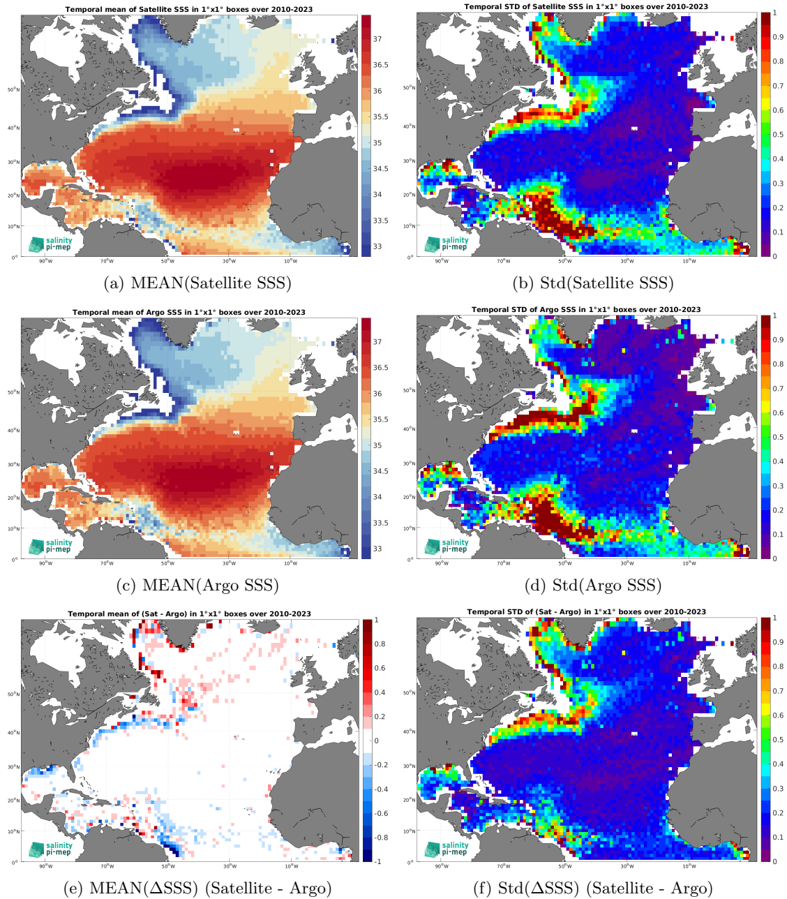
Figure 7: Temporal mean (left) and Std (right) of SSS from CCI SSS L4 Merged-OI v5.5 - 7-day running (ESA) (top), Argo (middle), and of \Delta SSS (Satellite - Argo). Only match-up pairs are used to generate these maps.
