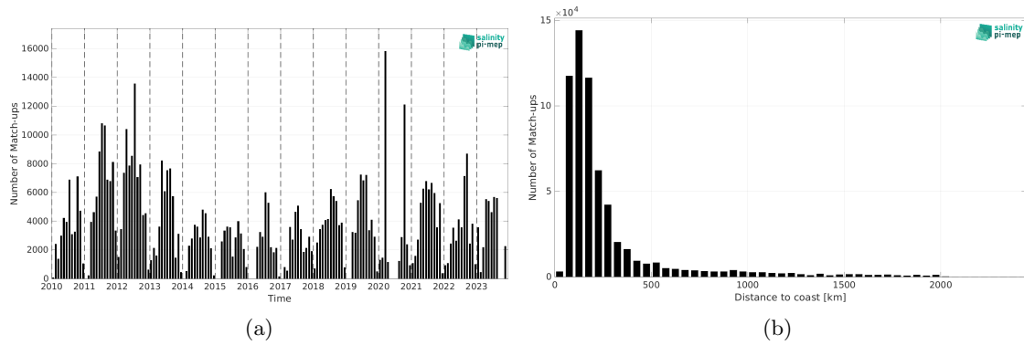
Figure 2: Number of match-ups between TSG (SAMOS) and CCI SSS L4 Merged-OI v5.5 - 30-day running (ESA) SSS as a function of time (a) and as function of the distance to coast (b) over the North Atlantic Ocean Pi-MEP region and for the full satellite product period.
