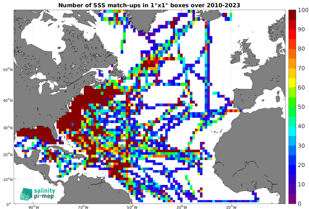
Figure 5: Number of SSS match-ups between TSG (SAMOS) SSS and the CCI SSS L4 Merged-OI v5.5 - 30-day running (ESA) SSS product for the North Atlantic Ocean Pi-MEP region over 1^\circ \times 1^\circ boxes and for the full satellite product period.
