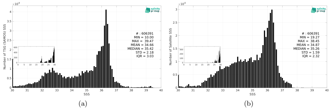
Figure 3: Histograms of SSS from TSG (SAMOS) (a) and CCI SSS L4 Merged-OI v5.5 - 30-day running (ESA) (b) considering all match-up pairs per bins of 0.1 over the North Atlantic Ocean Pi-MEP region and for the full satellite product period.
