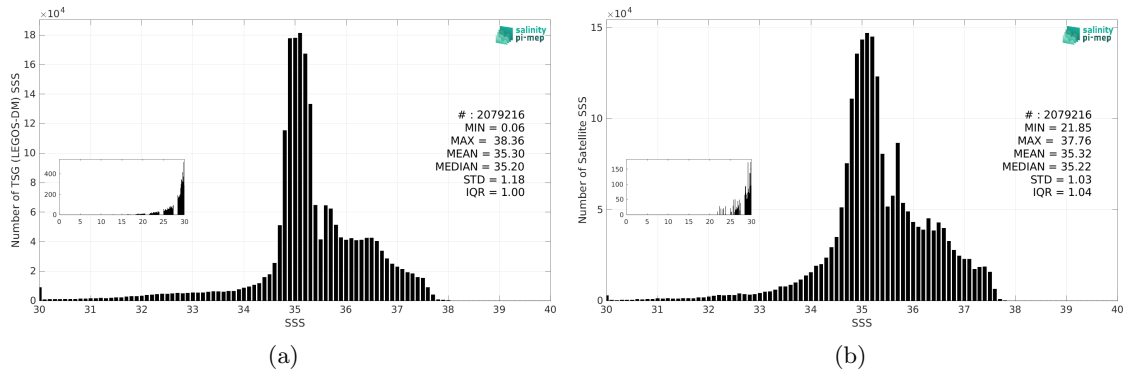
Figure 3: Histograms of SSS from TSG (LEGOS-DM) (a) and CCI SSS L4 Merged-OI v5.5 - 30-day running (ESA) (b) considering all match-up pairs per bins of 0.1 over the North Atlantic Ocean Pi-MEP region and for the full satellite product period.
