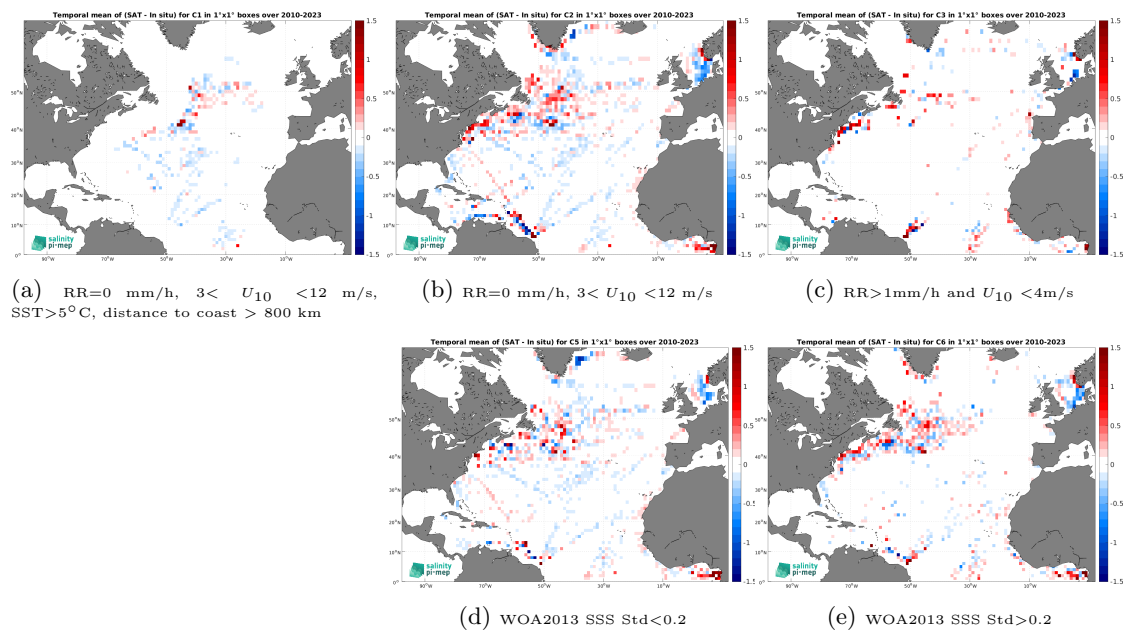
Figure 14: Temporal mean gridded over spatial boxes of size 1^\circ \times 1^\circ of \Delta\text{SSS} (CCI SSS L4 Merged-OI v5.5 - 30-day running (ESA) - TSG (LEGOS-DM)) for 5 different subdatasets corresponding to:RR=0 mm/h, 3 < U_{10} < 12 m/s, SST >5^\circ\text{C} , distance to coast > 800 km (a), RR=0 mm/h, 3 < U_{10} < 12 m/s (b), RR >1 mm/h and U_{10} < 4 m/s (c), WOA2013 SSS Std <0.2 (d), WOA2013 SSS Std >0.2 (e).
