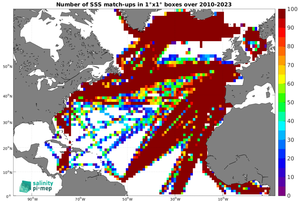
Figure 5: Number of SSS match-ups between TSG (LEGOS-DM) SSS and the CCI SSS L4 Merged-OI v5.5 - 30-day running (ESA) SSS product for the North Atlantic Ocean Pi-MEP region over 1^\circ \times 1^\circ boxes and for the full satellite product period.
