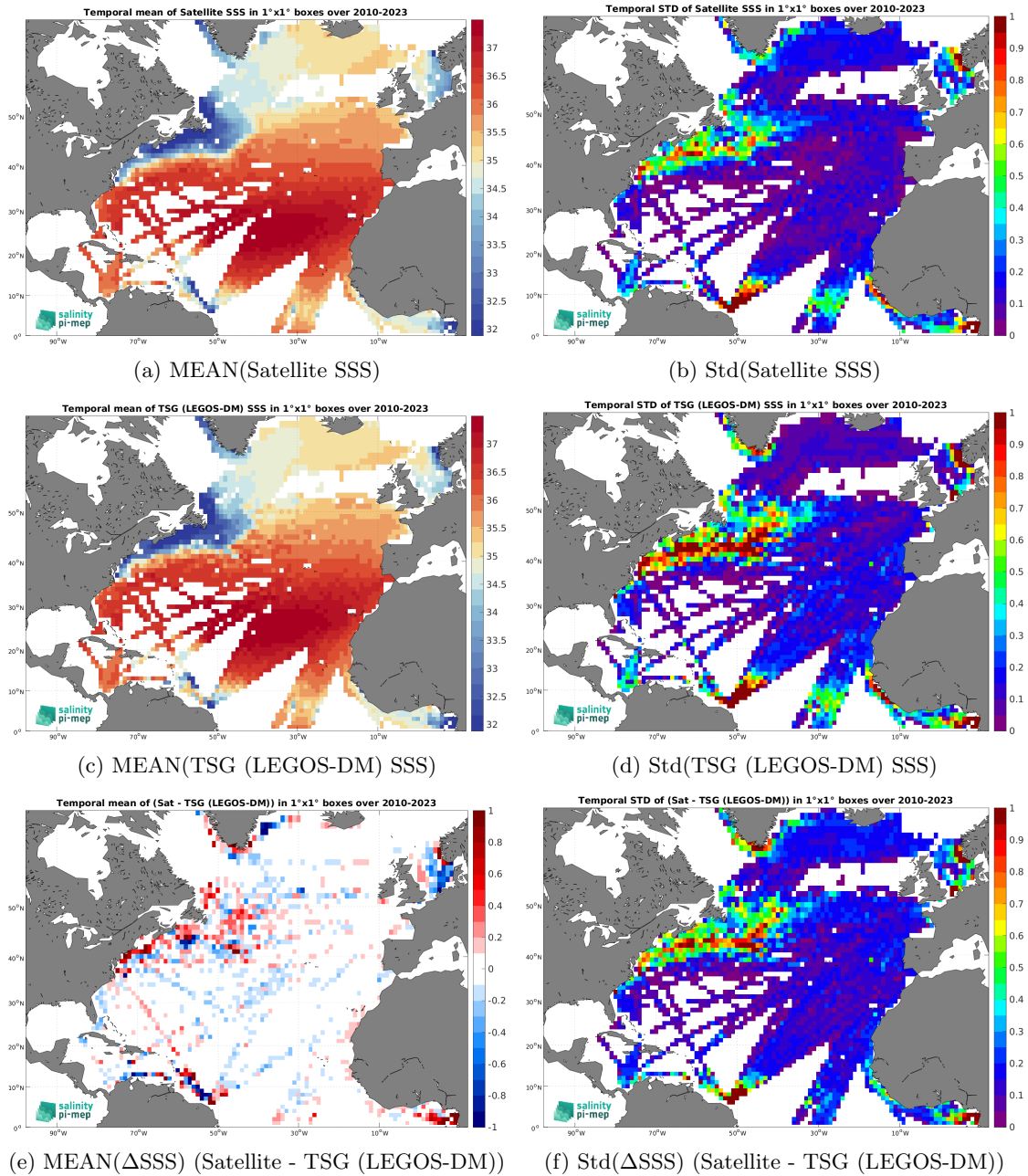
Figure 7: Temporal mean (left) and Std (right) of SSS from CCI SSS L4 Merged-OI v5.5 - 30-day running (ESA) (top), TSG (LEGOS-DM) (middle), and of \Delta SSS (Satellite - TSG (LEGOS-DM)). Only match-up pairs are used to generate these maps.
