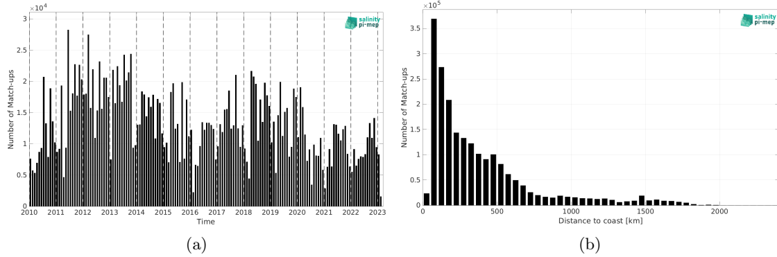
Figure 2: Number of match-ups between TSG (LEGOS-DM) and CCI SSS L4 Merged-OI v5.5 - 30-day running (ESA) SSS as a function of time (a) and as function of the distance to coast (b) over the North Atlantic Ocean Pi-MEP region and for the full satellite product period.
