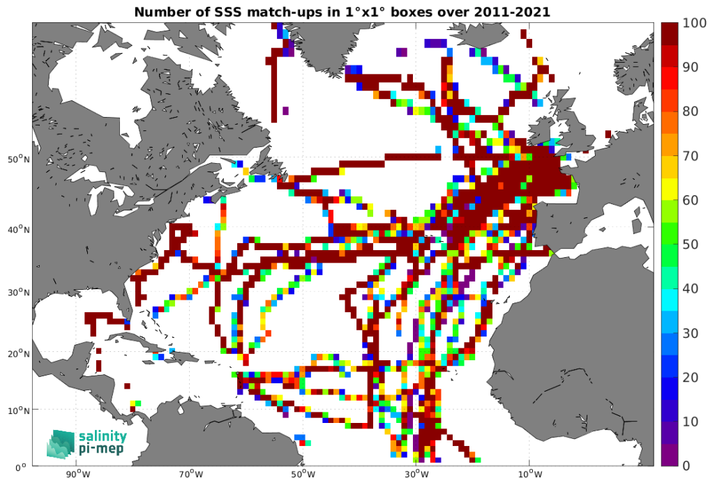
Figure 5: Number of SSS match-ups between TSG (GOSUD-Sailing-ship) SSS and the CCI SSS L4 Merged-OI v5.5 - 30-day running (ESA) SSS product for the North Atlantic Ocean Pi-MEP region over 1^\circ \times 1^\circ boxes and for the full satellite product period.
