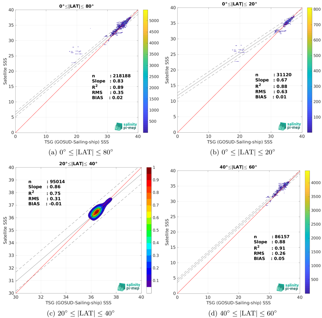
Figure 10: Contour maps of the concentration of CCI SSS L4 Merged-OI v5.5 - 30-day running (ESA) SSS ( y -axis) versus TSG (GOSUD-Sailing-ship) SSS ( x -axis) at match-up pairs for different latitude bands. For each plot, the red line shows x=y . The black thin and dashed lines indicate a linear fit through the data cloud and the \pm 95\% confidence levels, respectively. The number match-up pairs n , the slope and R^2 coefficient of the linear fit, the root mean square (RMS) and the mean bias between satellite and in situ data are indicated for each latitude band in each plots.
