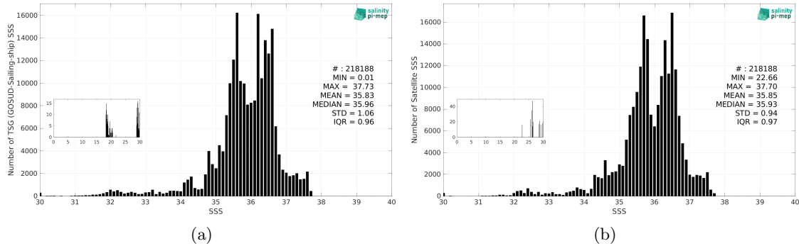
Figure 3: Histograms of SSS from TSG (GOSUD-Sailing-ship) (a) and CCI SSS L4 Merged-OI v5.5 - 30-day running (ESA) (b) considering all match-up pairs per bins of 0.1 over the North Atlantic Ocean Pi-MEP region and for the full satellite product period.
