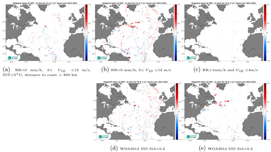
Figure 14: Temporal mean gridded over spatial boxes of size 1^\circ \times 1^\circ of \Delta\text{SSS} (CCI SSS L4 Merged-OI v5.5 - 30-day running (ESA) - TSG (GOSUD-Sailing-ship)) for 5 different subdatasets corresponding to:RR=0 mm/h, 3 < U_{10} < 12 m/s, SST >5^\circ\text{C} , distance to coast > 800 km (a), RR=0 mm/h, 3 < U_{10} < 12 m/s (b), RR >1 mm/h and U_{10} < 4 m/s (c), WOA2013 SSS Std <0.2 (d), WOA2013 SSS Std >0.2 (e).
