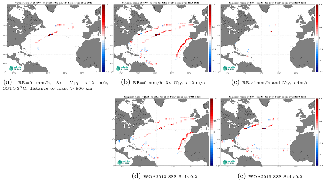
Figure 14: Temporal mean gridded over spatial boxes of size 1^\circ \times 1^\circ of \Delta\text{SSS} (CCI SSS L4 Merged-OI v5.5 - 30-day running (ESA) - Saildrone) for 5 different subdatasets corresponding to:RR=0 mm/h, 3 < U_{10} < 12 m/s, SST >5^\circ\text{C} , distance to coast > 800 km (a), RR=0 mm/h, 3 < U_{10} < 12 m/s (b), RR >1 mm/h and U_{10} < 4 m/s (c), WOA2013 SSS Std <0.2 (d), WOA2013 SSS Std >0.2 (e).
