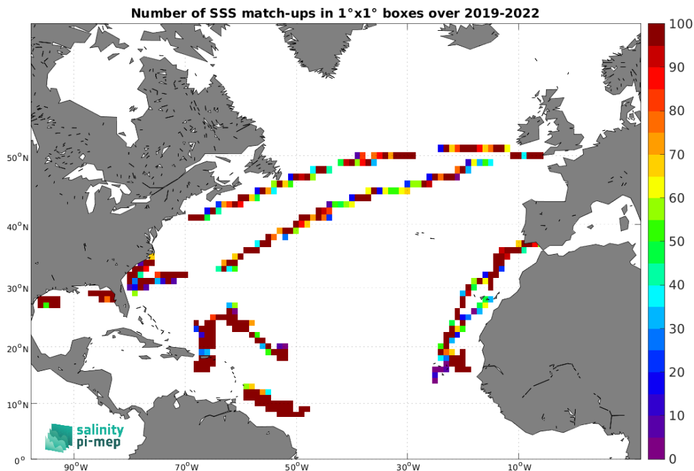
Figure 5: Number of SSS match-ups between Saildrone SSS and the CCI SSS L4 Merged-OI v5.5 - 30-day running (ESA) SSS product for the North Atlantic Ocean Pi-MEP region over 1^\circ \times 1^\circ boxes and for the full satellite product period.
