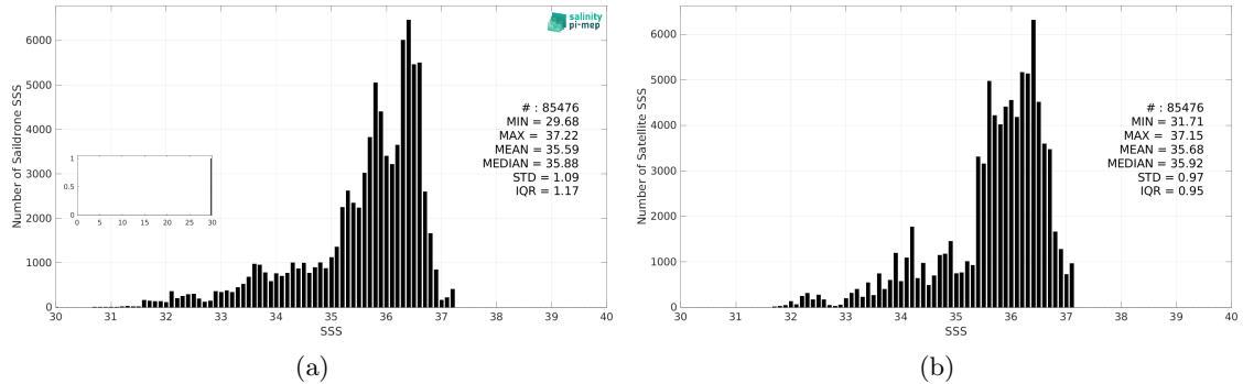
Figure 3: Histograms of SSS from Saildrone (a) and CCI SSS L4 Merged-OI v5.5 - 30-day running (ESA) (b) considering all match-up pairs per bins of 0.1 over the North Atlantic Ocean Pi-MEP region and for the full satellite product period.
