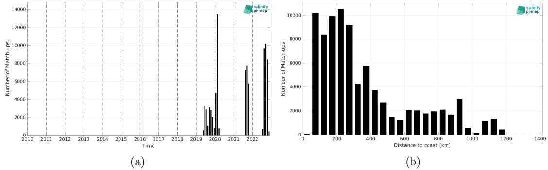
Figure 2: Number of match-ups between Saildrone and CCI SSS L4 Merged-OI v5.5 - 30-day running (ESA) SSS as a function of time (a) and as function of the distance to coast (b) over the North Atlantic Ocean Pi-MEP region and for the full satellite product period.
