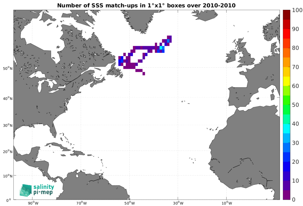
Figure 5: Number of SSS match-ups between Marine mammals SSS and the CCI SSS L4 Merged-OI v5.5 - 30-day running (ESA) SSS product for the North Atlantic Ocean Pi-MEP region over 1^\circ \times 1^\circ boxes and for the full satellite product period.
