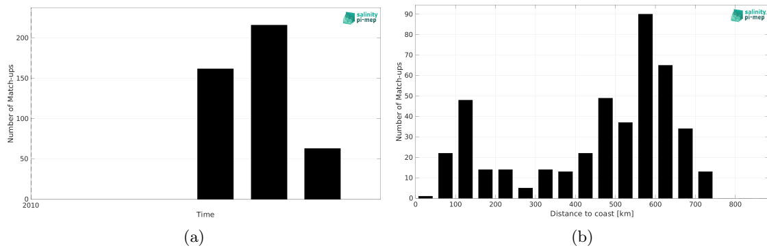
Figure 2: Number of match-ups between Marine mammals and CCI SSS L4 Merged-OI v5.5 - 30-day running (ESA) SSS as a function of time (a) and as function of the distance to coast (b) over the North Atlantic Ocean Pi-MEP region and for the full satellite product period.
