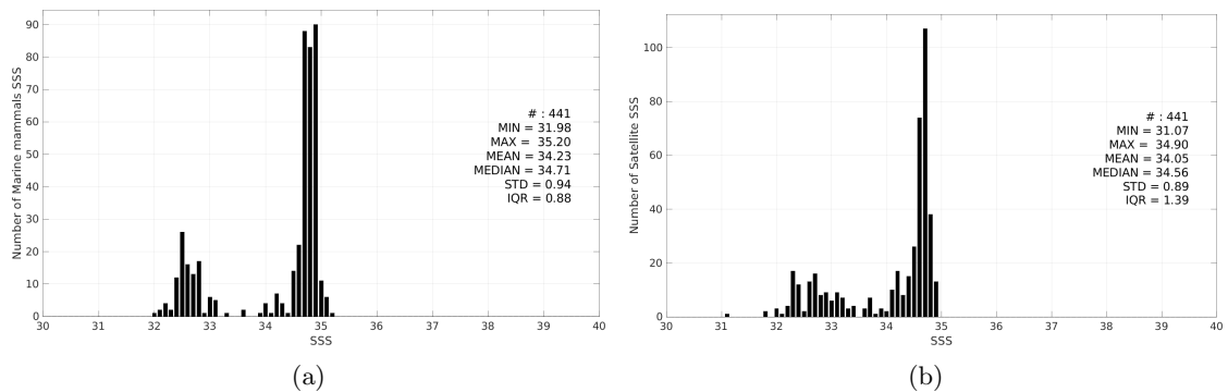
Figure 3: Histograms of SSS from Marine mammals (a) and CCI SSS L4 Merged-OI v5.5 - 30-day running (ESA) (b) considering all match-up pairs per bins of 0.1 over the North Atlantic Ocean Pi-MEP region and for the full satellite product period.
