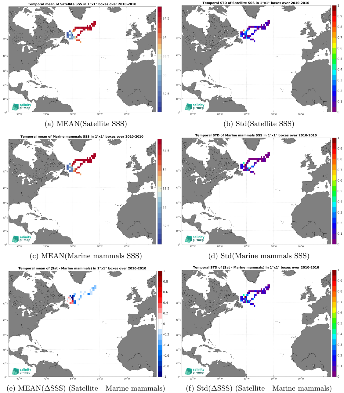
Figure 7: Temporal mean (left) and Std (right) of SSS from CCI SSS L4 Merged-OI v5.5 - 30-day running (ESA) (top), Marine mammals (middle), and of \Delta SSS (Satellite - Marine mammals). Only match-up pairs are used to generate these maps.
