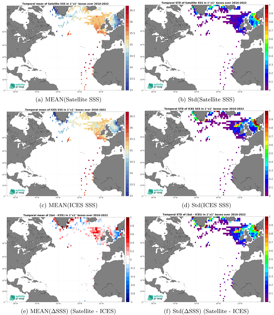
Figure 7: Temporal mean (left) and Std (right) of SSS from CCI SSS L4 Merged-OI v5.5 - 30-day running (ESA) (top), ICES (middle), and of \Delta SSS (Satellite - ICES). Only match-up pairs are used to generate these maps.
