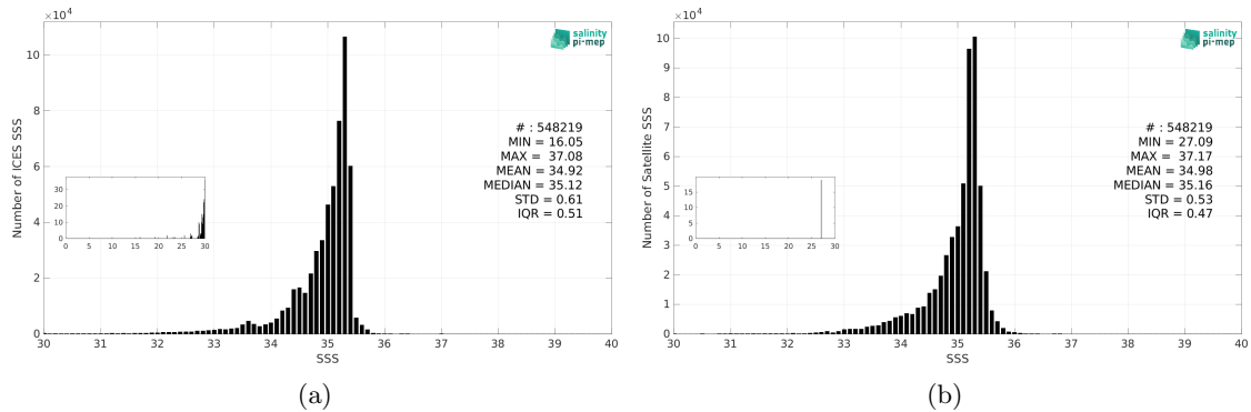
Figure 3: Histograms of SSS from ICES (a) and CCI SSS L4 Merged-OI v5.5 - 30-day running (ESA) (b) considering all match-up pairs per bins of 0.1 over the North Atlantic Ocean Pi-MEP region and for the full satellite product period.
