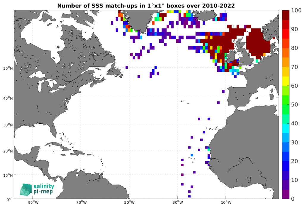
Figure 5: Number of SSS match-ups between ICES SSS and the CCI SSS L4 Merged-OI v5.5 - 30-day running (ESA) SSS product for the North Atlantic Ocean Pi-MEP region over 1^\circ \times 1^\circ boxes and for the full satellite product period.
