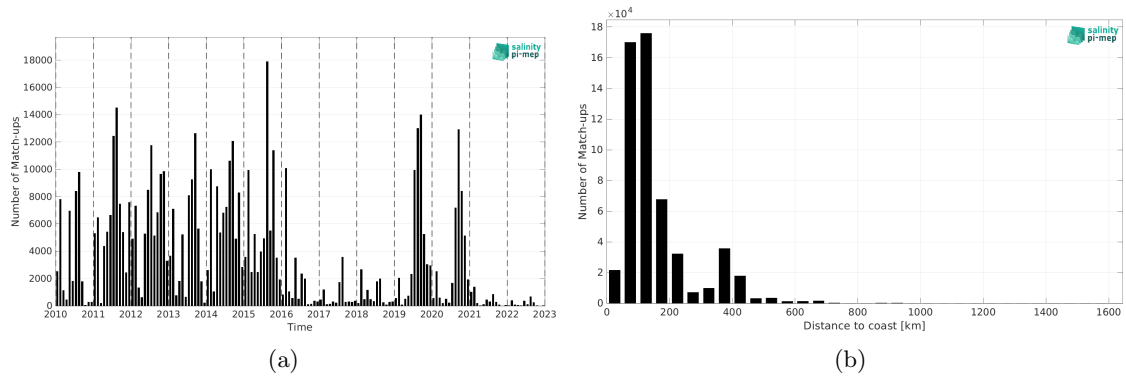
Figure 2: Number of match-ups between ICES and CCI SSS L4 Merged-OI v5.5 - 30-day running (ESA) SSS as a function of time (a) and as function of the distance to coast (b) over the North Atlantic Ocean Pi-MEP region and for the full satellite product period.
