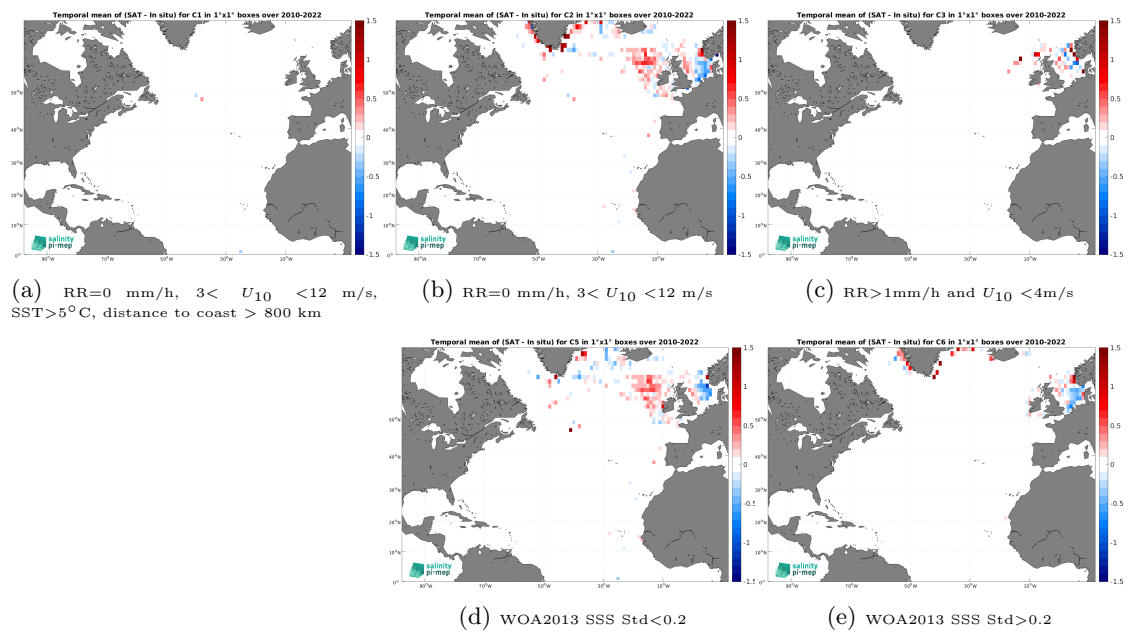
Figure 14: Temporal mean gridded over spatial boxes of size 1^\circ \times 1^\circ of \Delta\text{SSS} (CCI SSS L4 Merged-OI v5.5 - 30-day running (ESA) - ICES) for 5 different subdatasets corresponding to:RR=0 mm/h, 3 < U_{10} < 12 m/s, SST >5^\circ\text{C} , distance to coast > 800 km (a), RR=0 mm/h, 3 < U_{10} < 12 m/s (b), RR >1 mm/h and U_{10} < 4 m/s (c), WOA2013 SSS Std <0.2 (d), WOA2013 SSS Std >0.2 (e).
