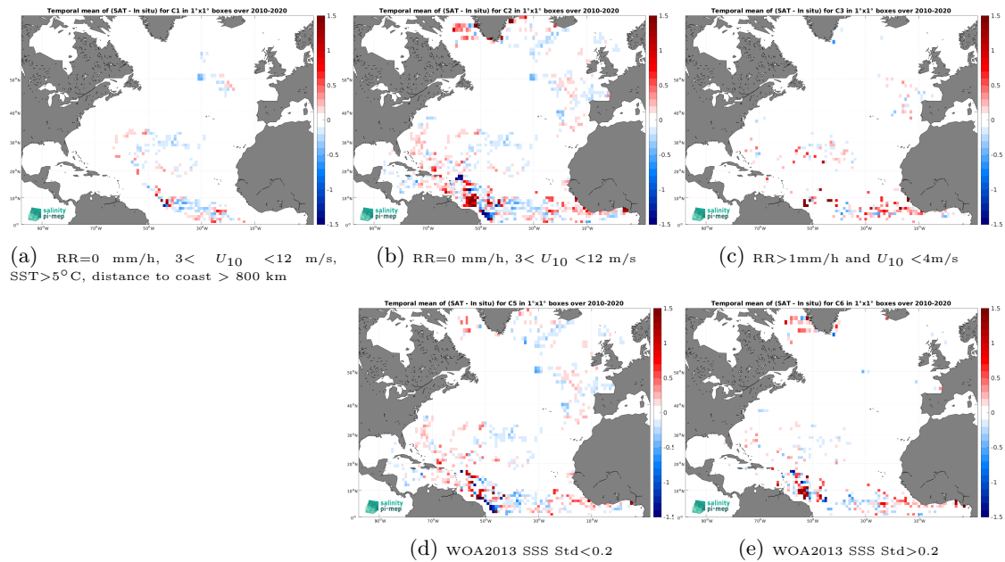
Figure 13: Temporal mean gridded over spatial boxes of size 1^\circ \times 1^\circ of \Delta\text{SSS} (CCI SSS L4 Merged-OI v5.5 - 30-day running (ESA) - Surface drifters) for 5 different subdatasets corresponding to:RR=0 mm/h, 3 < U_{10} < 12 m/s, SST >5^\circ\text{C} , distance to coast > 800 km (a), RR=0 mm/h, 3 < U_{10} < 12 m/s (b), RR >1 mm/h and U_{10} < 4 m/s (c), WOA2013 SSS Std <0.2 (d), WOA2013 SSS Std >0.2 (e).
