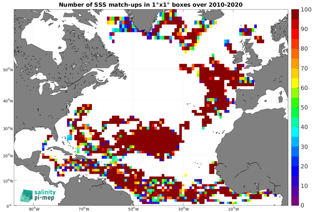
Figure 4: Number of SSS match-ups between Surface drifters SSS and the CCI SSS L4 Merged-OI v5.5 - 30-day running (ESA) SSS product for the North Atlantic Ocean Pi-MEP region over 1^\circ \times 1^\circ boxes and for the full satellite product period.
