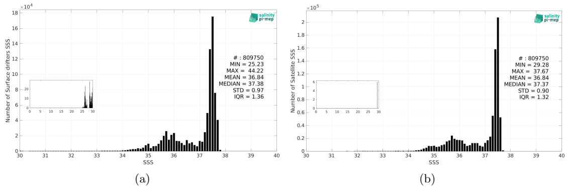
Figure 3: Histograms of SSS from Surface drifters (a) and CCI SSS L4 Merged-OI v5.5 - 30-day running (ESA) (b) considering all match-up pairs per bins of 0.1 over the North Atlantic Ocean Pi-MEP region and for the full satellite product period.
