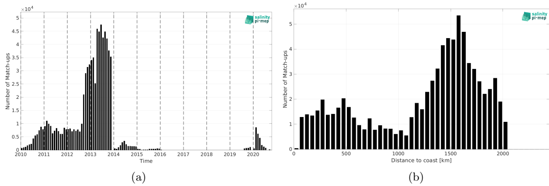
Figure 2: Number of match-ups between Surface drifters and CCI SSS L4 Merged-OI v5.5 - 30-day running (ESA) SSS as a function of time (a) and as function of the distance to coast (b) over the North Atlantic Ocean Pi-MEP region and for the full satellite product period.
