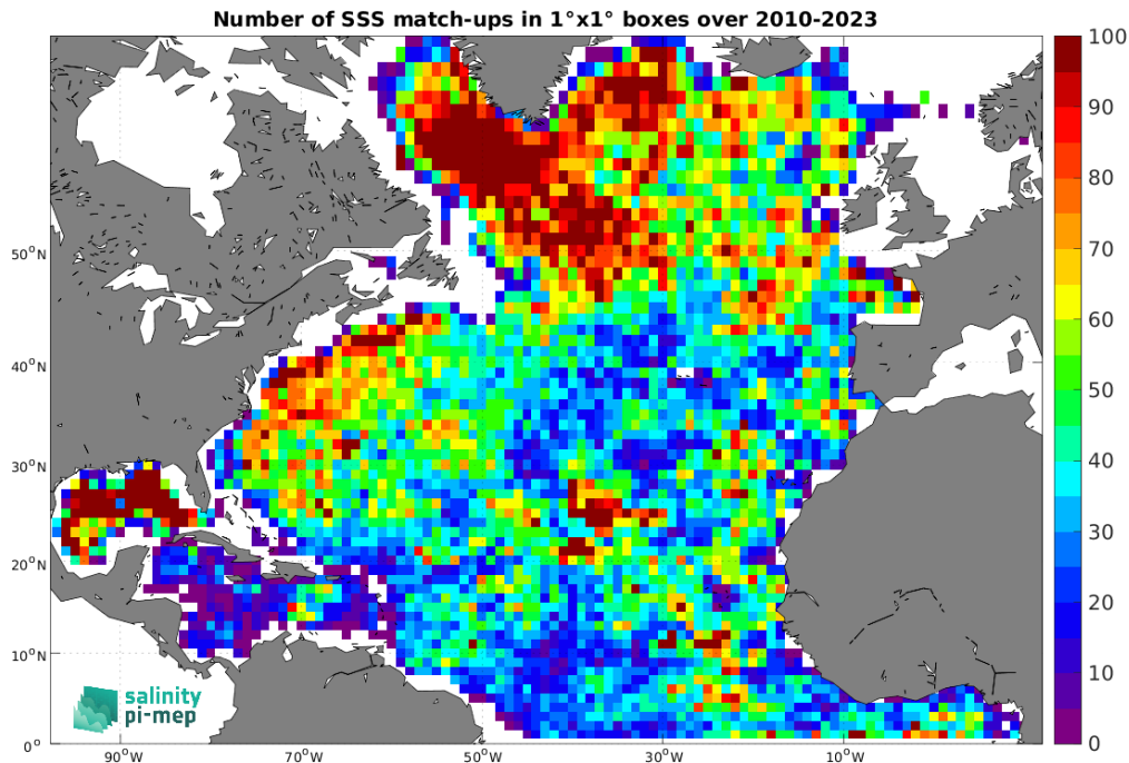
Figure 5: Number of SSS match-ups between Argo SSS and the CCI SSS L4 Merged-OI v5.5 - 30-day running (ESA) SSS product for the North Atlantic Ocean Pi-MEP region over 1^\circ \times 1^\circ boxes and for the full satellite product period.
