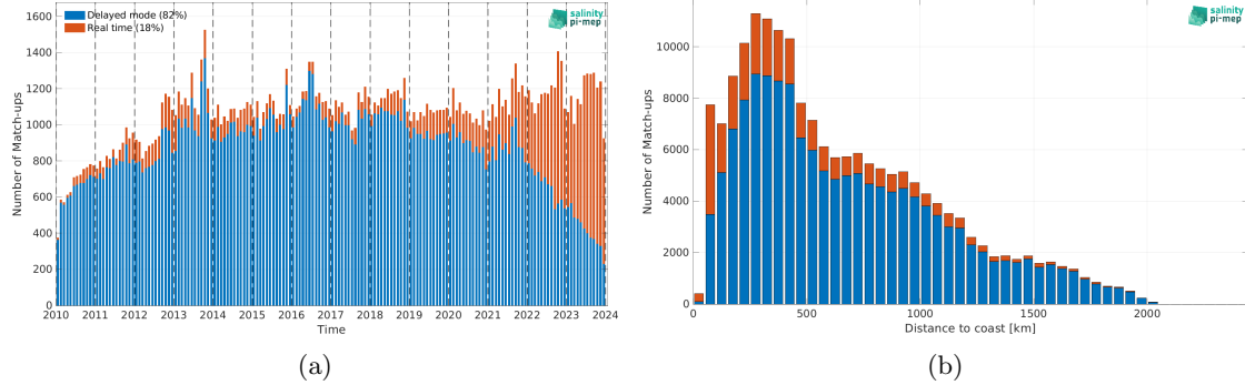
Figure 2: Number of match-ups between Argo and CCI SSS L4 Merged-OI v5.5 - 30-day running (ESA) SSS as a function of time (a) and as function of the distance to coast (b) over the North Atlantic Ocean Pi-MEP region and for the full satellite product period.
