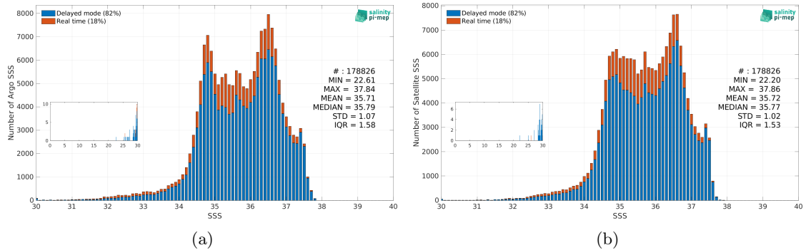
Figure 3: Histograms of SSS from Argo (a) and CCI SSS L4 Merged-OI v5.5 - 30-day running (ESA) (b) considering all match-up pairs per bins of 0.1 over the North Atlantic Ocean Pi-MEP region and for the full satellite product period.
