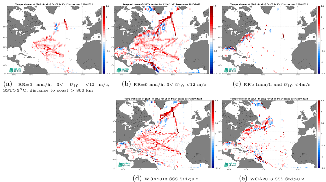
Figure 14: Temporal mean gridded over spatial boxes of size 1^\circ \times 1^\circ of \Delta\text{SSS} (CCI SSS L4 Merged-OI v4.41 - 7-day running (ESA) - TSG (SAMOS)) for 5 different subdatasets corresponding to:RR=0 mm/h, 3 < U_{10} < 12 m/s, SST >5^\circ\text{C} , distance to coast > 800 km (a), RR=0 mm/h, 3 < U_{10} < 12 m/s (b), RR >1 mm/h and U_{10} < 4 m/s (c), WOA2013 SSS Std <0.2 (d), WOA2013 SSS Std >0.2 (e).
