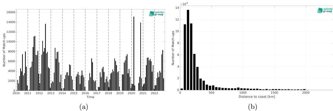
Figure 2: Number of match-ups between TSG (SAMOS) and CCI SSS L4 Merged-OI v4.41 - 7-day running (ESA) SSS as a function of time (a) and as function of the distance to coast (b) over the North Atlantic Ocean Pi-MEP region and for the full satellite product period.
