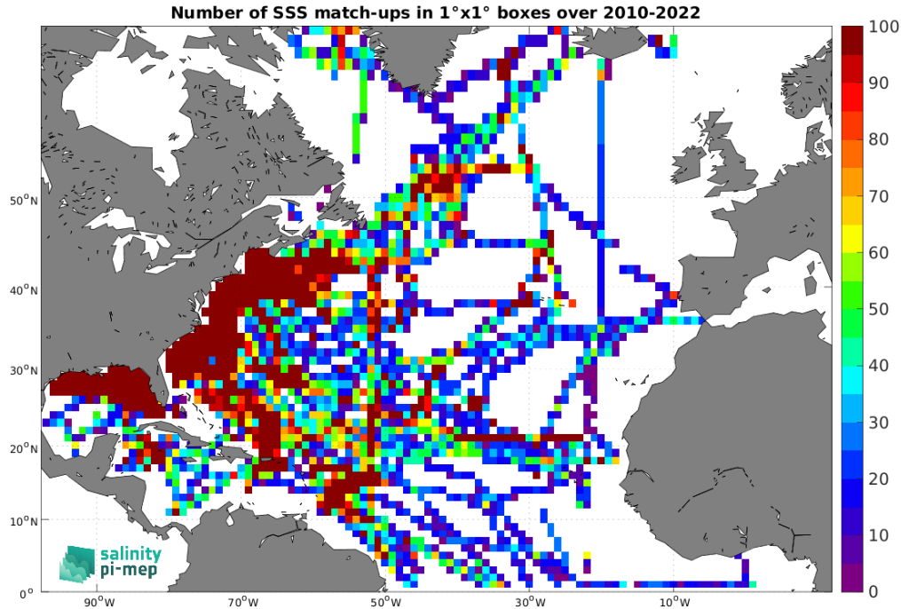
Figure 5: Number of SSS match-ups between TSG (SAMOS) SSS and the CCI SSS L4 Merged-OI v4.41 - 7-day running (ESA) SSS product for the North Atlantic Ocean Pi-MEP region over 1^\circ \times 1^\circ boxes and for the full satellite product period.
