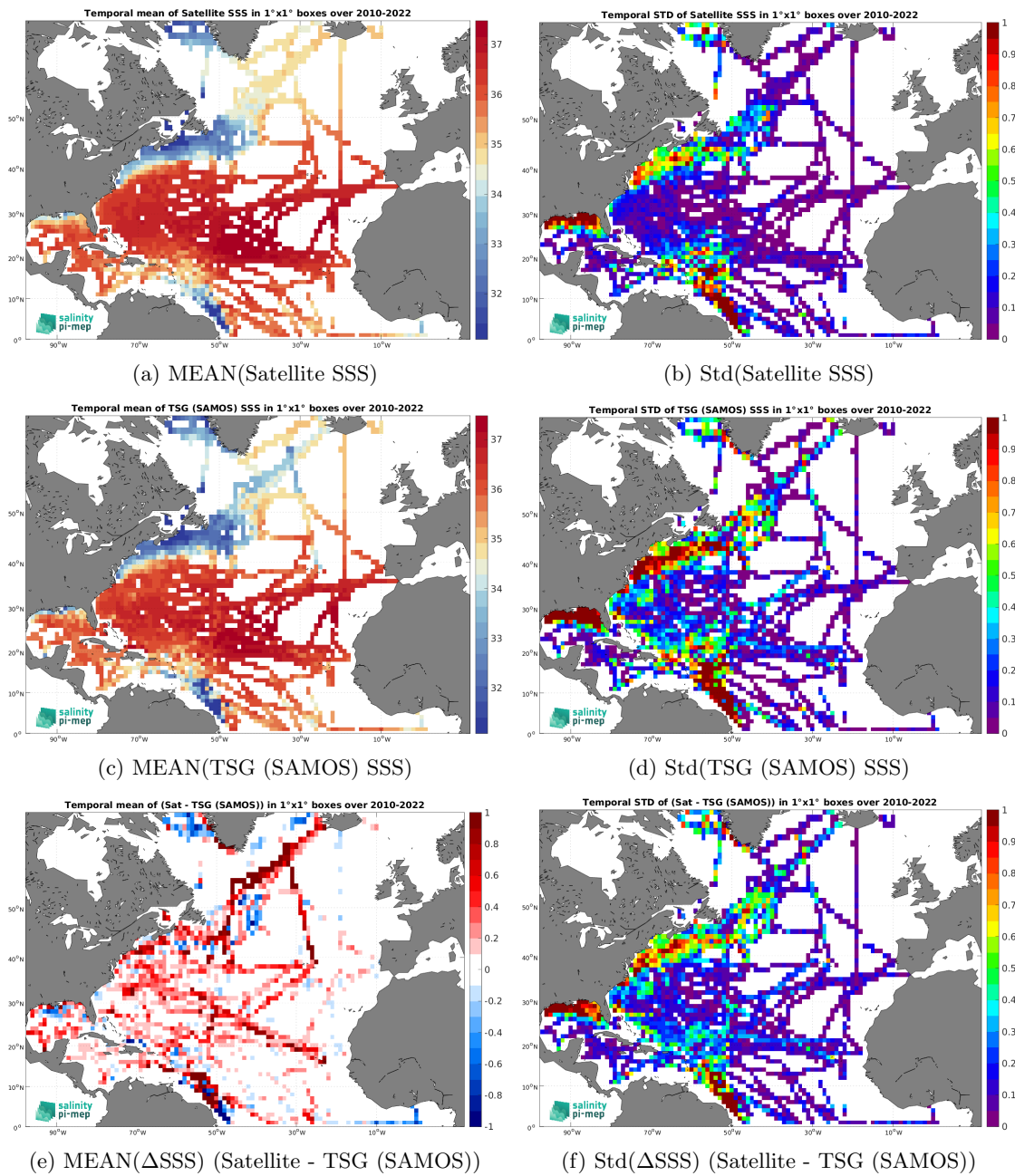
Figure 7: Temporal mean (left) and Std (right) of SSS from CCI SSS L4 Merged-OI v4.41 - 7-day running (ESA) (top), TSG (SAMOS) (middle), and of \Delta SSS (Satellite - TSG (SAMOS)). Only match-up pairs are used to generate these maps.
