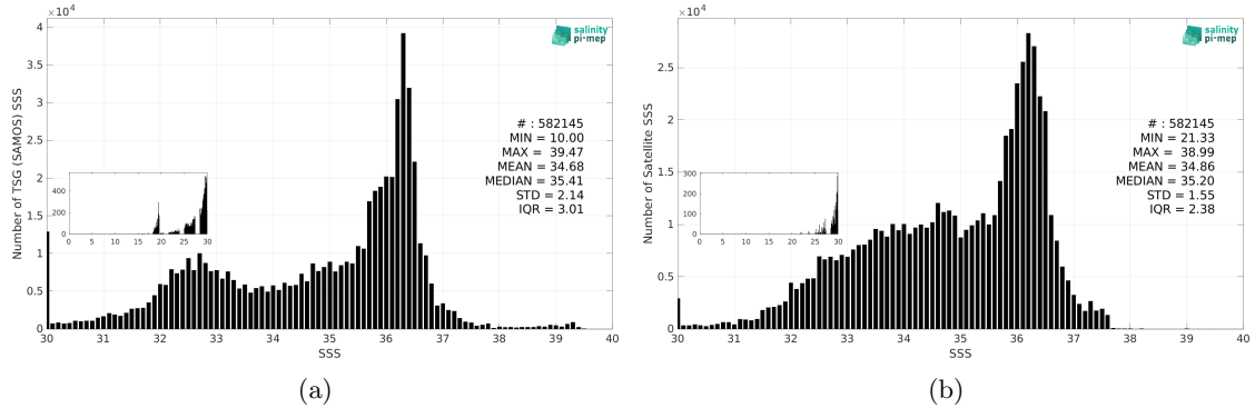
Figure 3: Histograms of SSS from TSG (SAMOS) (a) and CCI SSS L4 Merged-OI v4.41 - 7-day running (ESA) (b) considering all match-up pairs per bins of 0.1 over the North Atlantic Ocean Pi-MEP region and for the full satellite product period.
