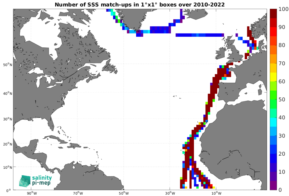
Figure 5: Number of SSS match-ups between TSG (Polarstern) SSS and the CCI SSS L4 Merged-OI v4.41 - 7-day running (ESA) SSS product for the North Atlantic Ocean Pi-MEP region over 1^\circ \times 1^\circ boxes and for the full satellite product period.
