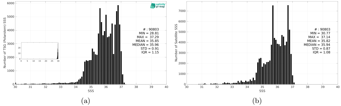
Figure 3: Histograms of SSS from TSG (Polarstern) (a) and CCI SSS L4 Merged-OI v4.41 - 7-day running (ESA) (b) considering all match-up pairs per bins of 0.1 over the North Atlantic Ocean Pi-MEP region and for the full satellite product period.
