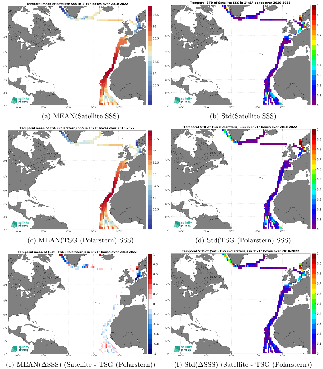
Figure 7: Temporal mean (left) and Std (right) of SSS from CCI SSS L4 Merged-OI v4.41 - 7-day running (ESA) (top), TSG (Polarstern) (middle), and of \Delta SSS (Satellite - TSG (Polarstern)). Only match-up pairs are used to generate these maps.
