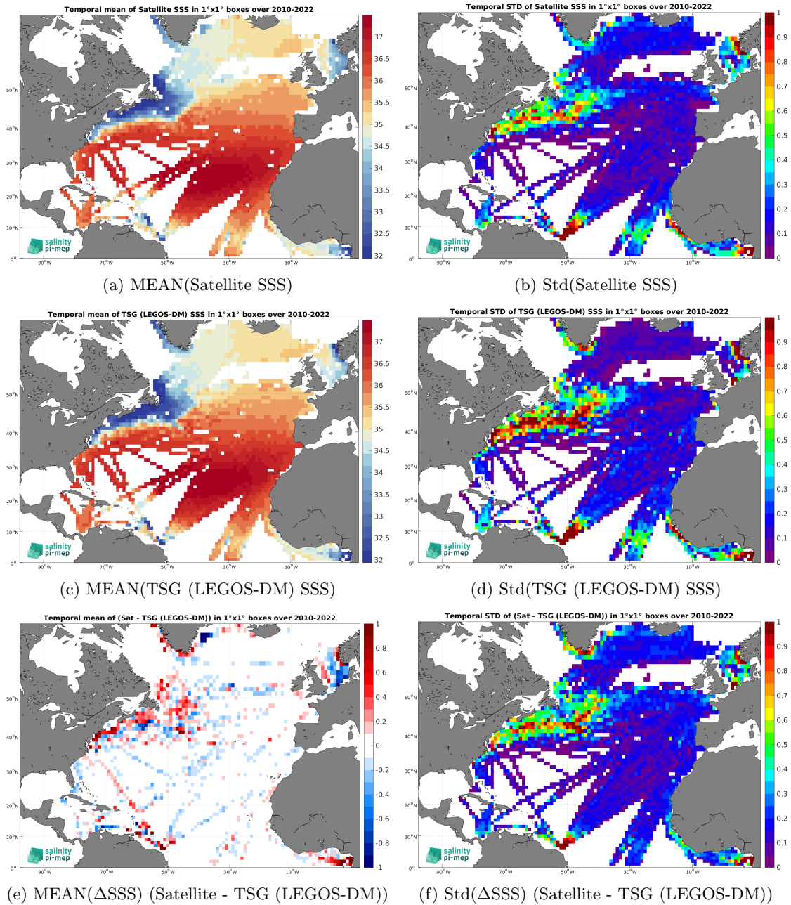
Figure 7: Temporal mean (left) and Std (right) of SSS from CCI SSS L4 Merged-OI v4.41 - 7-day running (ESA) (top), TSG (LEGOS-DM) (middle), and of \Delta SSS (Satellite - TSG (LEGOS-DM)). Only match-up pairs are used to generate these maps.
