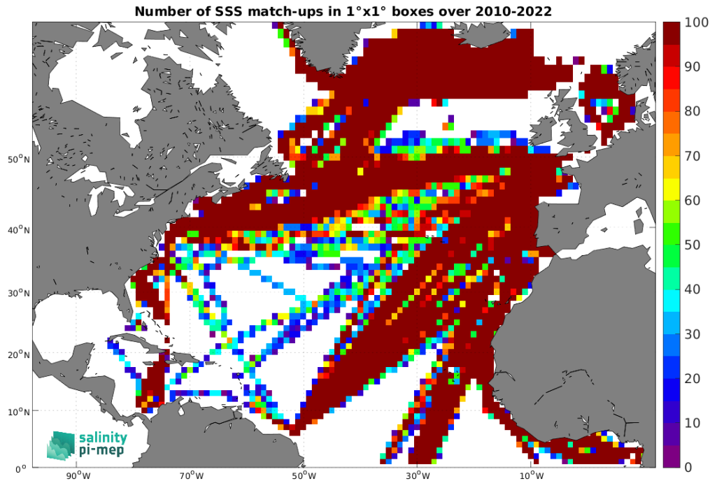
Figure 5: Number of SSS match-ups between TSG (LEGOS-DM) SSS and the CCI SSS L4 Merged-OI v4.41 - 7-day running (ESA) SSS product for the North Atlantic Ocean Pi-MEP region over 1^\circ \times 1^\circ boxes and for the full satellite product period.
