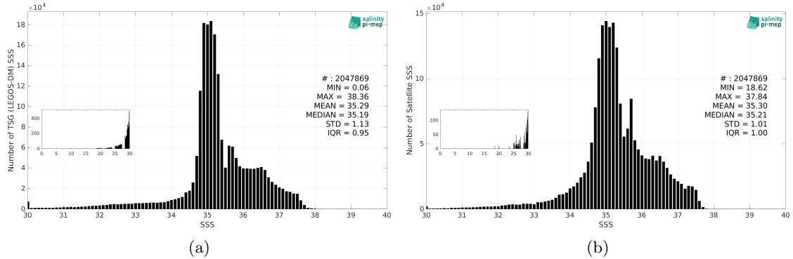
Figure 3: Histograms of SSS from TSG (LEGOS-DM) (a) and CCI SSS L4 Merged-OI v4.41 - 7-day running (ESA) (b) considering all match-up pairs per bins of 0.1 over the North Atlantic Ocean Pi-MEP region and for the full satellite product period.
