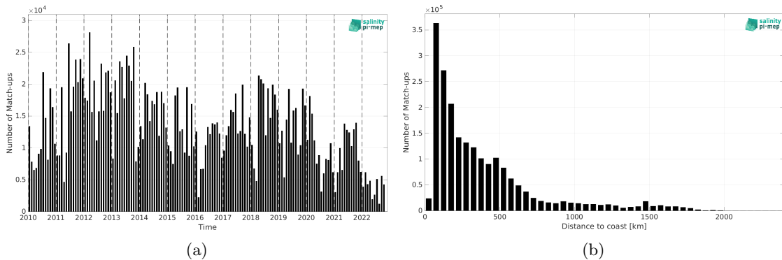
Figure 2: Number of match-ups between TSG (LEGOS-DM) and CCI SSS L4 Merged-OI v4.41 - 7-day running (ESA) SSS as a function of time (a) and as function of the distance to coast (b) over the North Atlantic Ocean Pi-MEP region and for the full satellite product period.
