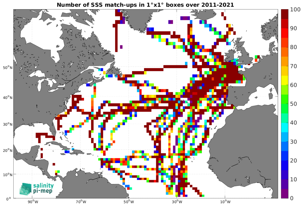
Figure 5: Number of SSS match-ups between TSG (GOSUD-Sailing-ship) SSS and the CCI SSS L4 Merged-OI v4.41 - 7-day running (ESA) SSS product for the North Atlantic Ocean Pi-MEP region over 1^\circ \times 1^\circ boxes and for the full satellite product period.
