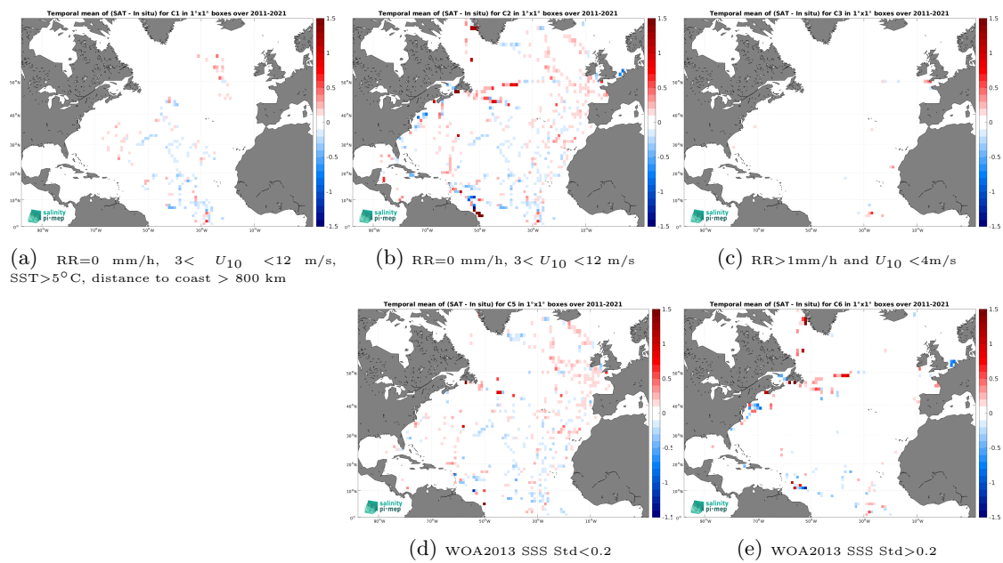
Figure 14: Temporal mean gridded over spatial boxes of size 1^\circ \times 1^\circ of \Delta\text{SSS} (CCI SSS L4 Merged-OI v4.41 - 7-day running (ESA) - TSG (GOSUD-Sailing-ship)) for 5 different subdatasets corresponding to:RR=0 mm/h, 3 < U_{10} < 12 m/s, SST >5^\circ\text{C} , distance to coast > 800 km (a), RR=0 mm/h, 3 < U_{10} < 12 m/s (b), RR >1 mm/h and U_{10} < 4 m/s (c), WOA2013 SSS Std <0.2 (d), WOA2013 SSS Std >0.2 (e).
