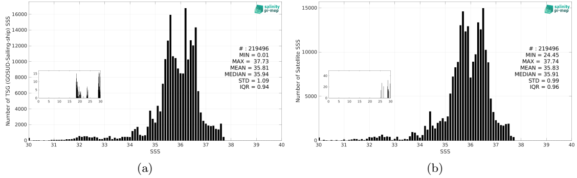
Figure 3: Histograms of SSS from TSG (GOSUD-Sailing-ship) (a) and CCI SSS L4 Merged-OI v4.41 - 7-day running (ESA) (b) considering all match-up pairs per bins of 0.1 over the North Atlantic Ocean Pi-MEP region and for the full satellite product period.
