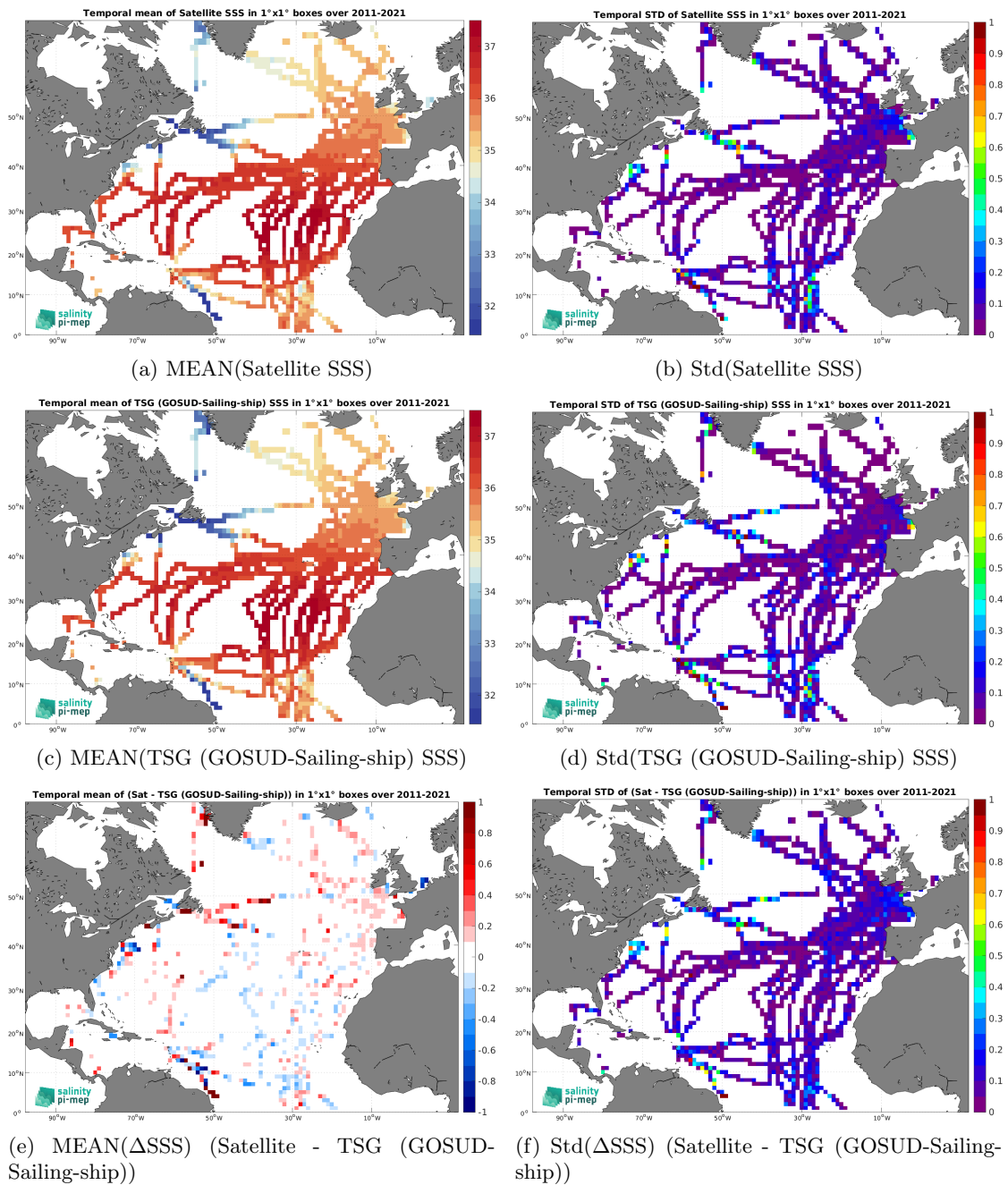
Figure 7: Temporal mean (left) and Std (right) of SSS from CCI SSS L4 Merged-OI v4.41 - 7-day running (ESA) (top), TSG (GOSUD-Sailing-ship) (middle), and of \Delta SSS (Satellite - TSG (GOSUD-Sailing-ship)). Only match-up pairs are used to generate these maps.
