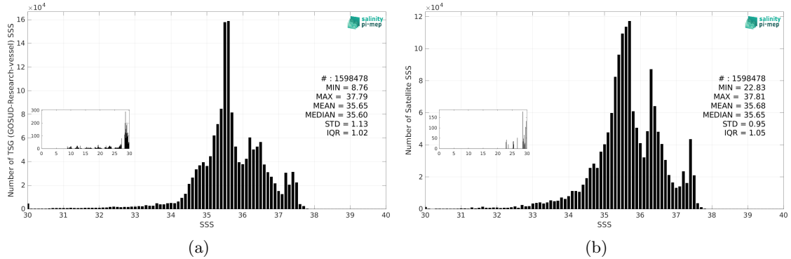
Figure 3: Histograms of SSS from TSG (GOSUD-Research-vessel) (a) and CCI SSS L4 Merged-OI v4.41 - 7-day running (ESA) (b) considering all match-up pairs per bins of 0.1 over the North Atlantic Ocean Pi-MEP region and for the full satellite product period.
