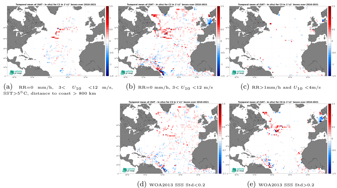
Figure 14: Temporal mean gridded over spatial boxes of size 1^\circ \times 1^\circ of \Delta\text{SSS} (CCI SSS L4 Merged-OI v4.41 - 7-day running (ESA) - TSG (GOSUD-Research-vessel)) for 5 different subdatasets corresponding to:RR=0 mm/h, 3 < U_{10} < 12 m/s, SST >5^\circ\text{C} , distance to coast > 800 km (a), RR=0 mm/h, 3 < U_{10} < 12 m/s (b), RR >1 mm/h and U_{10} < 4 m/s (c), WOA2013 SSS Std <0.2 (d), WOA2013 SSS Std >0.2 (e).
