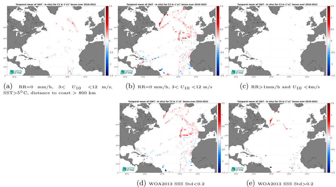
Figure 14: Temporal mean gridded over spatial boxes of size 1^\circ \times 1^\circ of \Delta\text{SSS} (CCI SSS L4 Merged-OI v4.41 - 7-day running (ESA) - TSG (CSIC-UTM)) for 5 different subdatasets corresponding to:RR=0 mm/h, 3 < U_{10} < 12 m/s, SST > 5°C, distance to coast > 800 km (a), RR=0 mm/h, 3 < U_{10} < 12 m/s (b), RR > 1mm/h and U_{10} < 4 m/s (c), WOA2013 SSS Std < 0.2 (d), WOA2013 SSS Std > 0.2 (e).
