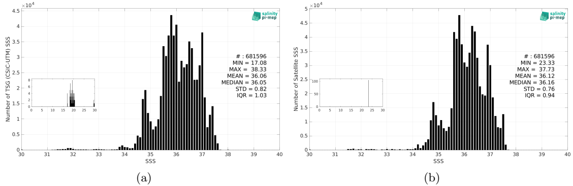
Figure 3: Histograms of SSS from TSG (CSIC-UTM) (a) and CCI SSS L4 Merged-OI v4.41 - 7-day running (ESA) (b) considering all match-up pairs per bins of 0.1 over the North Atlantic Ocean Pi-MEP region and for the full satellite product period.
