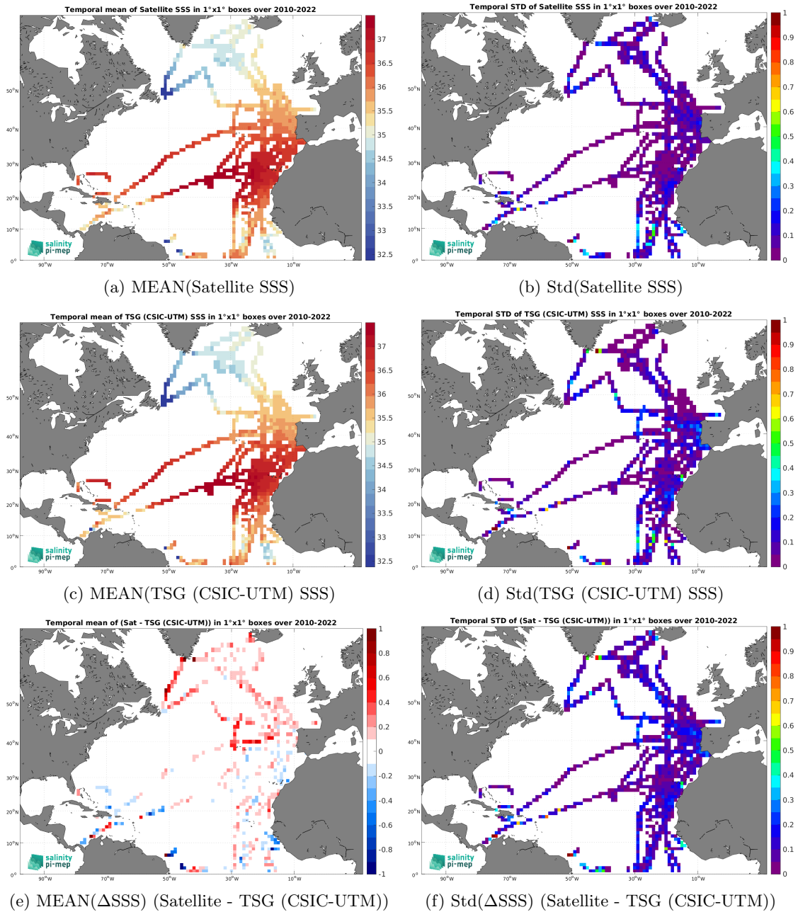
Figure 7: Temporal mean (left) and Std (right) of SSS from CCI SSS L4 Merged-OI v4.41 - 7-day running (ESA) (top), TSG (CSIC-UTM) (middle), and of \Delta SSS (Satellite - TSG (CSIC-UTM)). Only match-up pairs are used to generate these maps.
