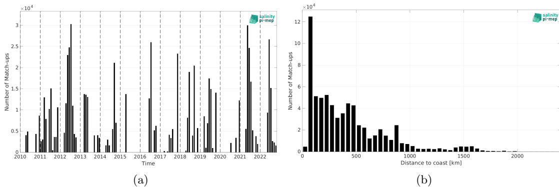
Figure 2: Number of match-ups between TSG (CSIC-UTM) and CCI SSS L4 Merged-OI v4.41 - 7-day running (ESA) SSS as a function of time (a) and as function of the distance to coast (b) over the North Atlantic Ocean Pi-MEP region and for the full satellite product period.
