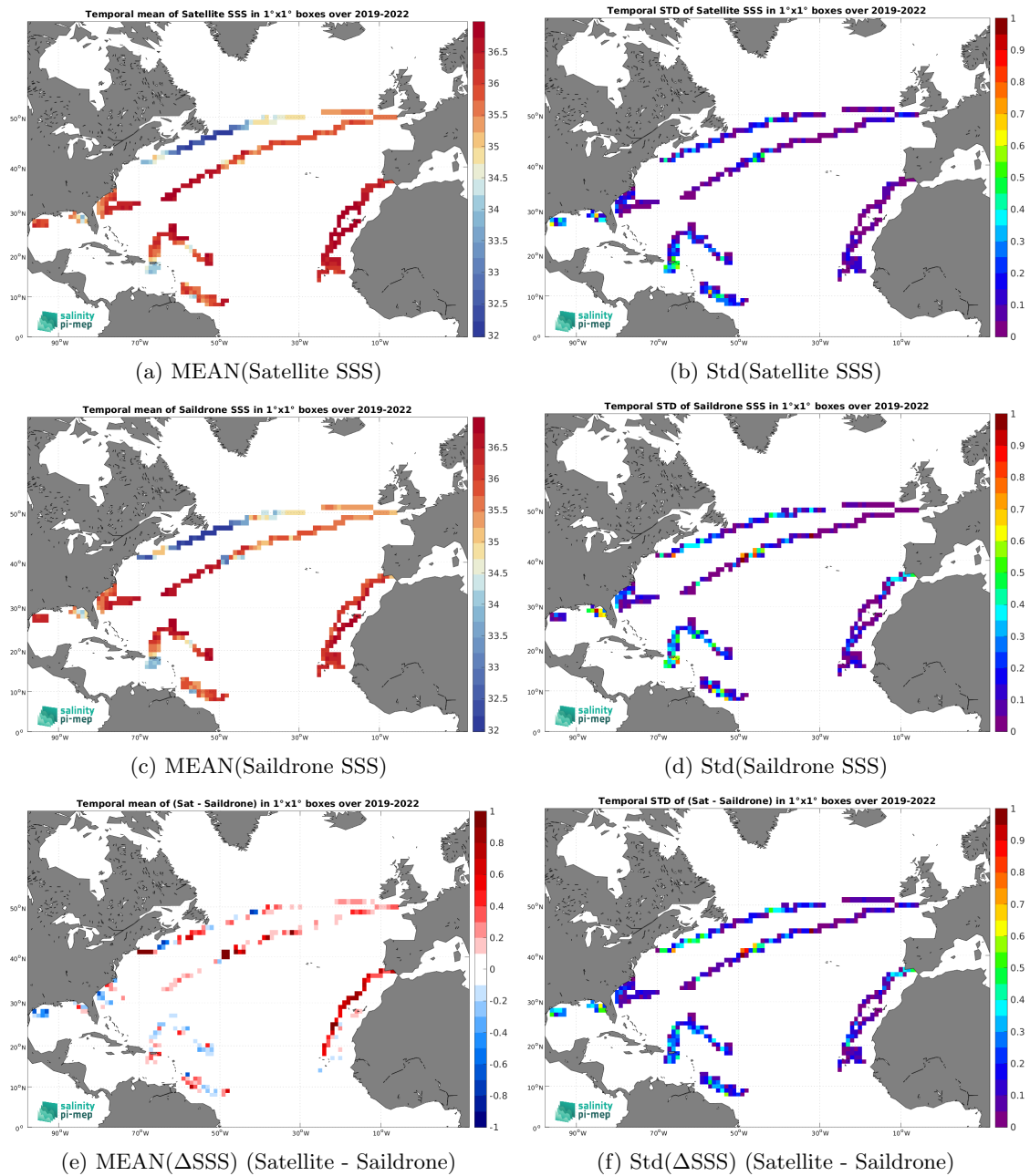
Figure 7: Temporal mean (left) and Std (right) of SSS from CCI SSS L4 Merged-OI v4.41 - 7-day running (ESA) (top), Saildrone (middle), and of \Delta SSS (Satellite - Saildrone). Only match-up pairs are used to generate these maps.
