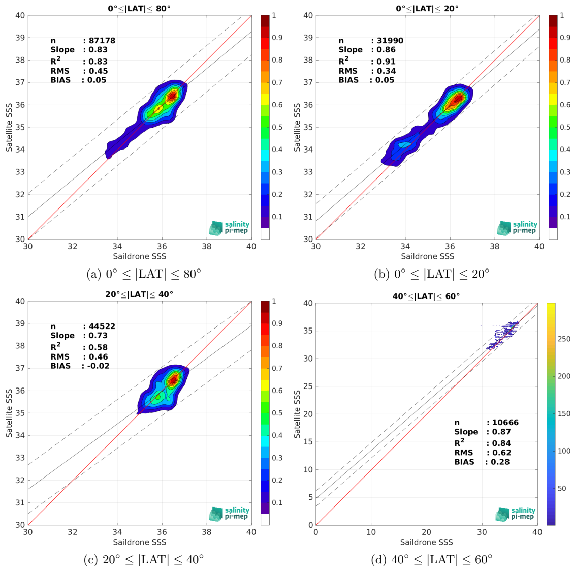
Figure 10: Contour maps of the concentration of CCI SSS L4 Merged-OI v4.41 - 7-day running (ESA) SSS (y-axis) versus Saldrone SSS (x-axis) at match-up pairs for different latitude bands. For each plot, the red line shows x=y . The black thin and dashed lines indicate a linear fit through the data cloud and the \pm 95\% confidence levels, respectively. The number match-up pairs n , the slope and R^2 coefficient of the linear fit, the root mean square (RMS) and the mean bias between satellite and in situ data are indicated for each latitude band in each plots.
