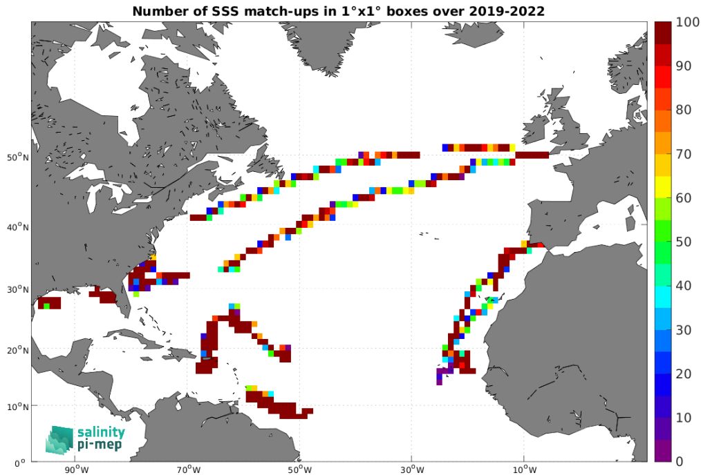
Figure 5: Number of SSS match-ups between Saildrone SSS and the CCI SSS L4 Merged-OI v4.41 - 7-day running (ESA) SSS product for the North Atlantic Ocean Pi-MEP region over 1^\circ \times 1^\circ boxes and for the full satellite product period.
