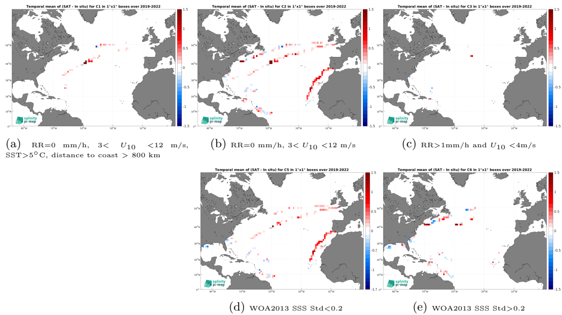
Figure 14: Temporal mean gridded over spatial boxes of size 1^\circ \times 1^\circ of \Delta\text{SSS} (CCI SSS L4 Merged-OI v4.41 - 7-day running (ESA) - Saildrone) for 5 different subdatasets corresponding to:RR=0 mm/h, 3 < U_{10} < 12 m/s, SST >5^\circ\text{C} , distance to coast > 800 km (a), RR=0 mm/h, 3 < U_{10} < 12 m/s (b), RR >1 mm/h and U_{10} < 4 m/s (c), WOA2013 SSS Std <0.2 (d), WOA2013 SSS Std >0.2 (e).
