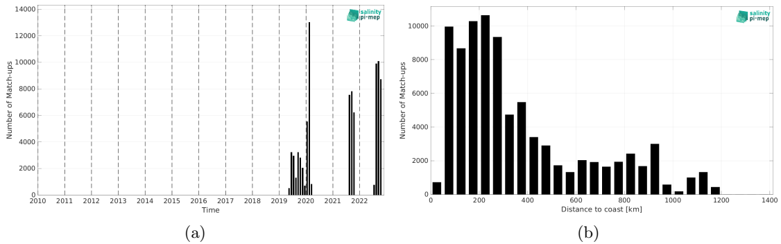
Figure 2: Number of match-ups between Saildrone and CCI SSS L4 Merged-OI v4.41 - 7-day running (ESA) SSS as a function of time (a) and as function of the distance to coast (b) over the North Atlantic Ocean Pi-MEP region and for the full satellite product period.
