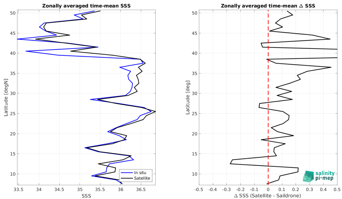
Figure 9: Left panel: Zonal mean SSS from CCI SSS L4 Merged-OI v4.41 - 7-day running (ESA) satellite product (black) and from Sairdrone (blue). Right panel: Zonal mean of \Delta SSS (Satellite - Sairdrone) for all the collected Pi-MEP match-up pairs estimated over the full satellite product period.
