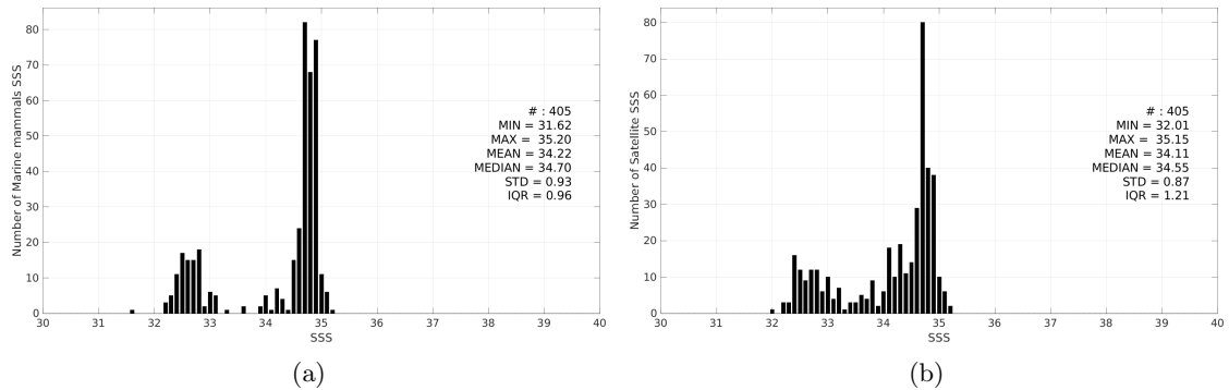
Figure 3: Histograms of SSS from Marine mammals (a) and CCI SSS L4 Merged-OI v4.41 - 7-day running (ESA) (b) considering all match-up pairs per bins of 0.1 over the North Atlantic Ocean Pi-MEP region and for the full satellite product period.
