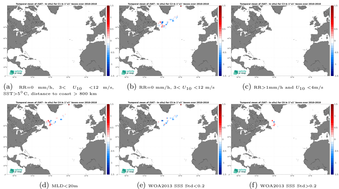
Figure 14: Temporal mean gridded over spatial boxes of size 1^\circ \times 1^\circ of \Delta SSS (CCI SSS L4 Merged-OI v4.41 - 7-day running (ESA) - Marine mammals) for 6 different subdatasets corresponding to:RR=0 mm/h, 3 < U_{10} < 12 m/s, SST > 5^\circ\text{C} , distance to coast > 800 km (a), RR=0 mm/h, 3 < U_{10} < 12 m/s (b), RR > 1 mm/h and U_{10} < 4 m/s (c),MLD < 20 m (d),WOA2013 SSS Std < 0.2 (e),WOA2013 SSS Std > 0.2 (f).
