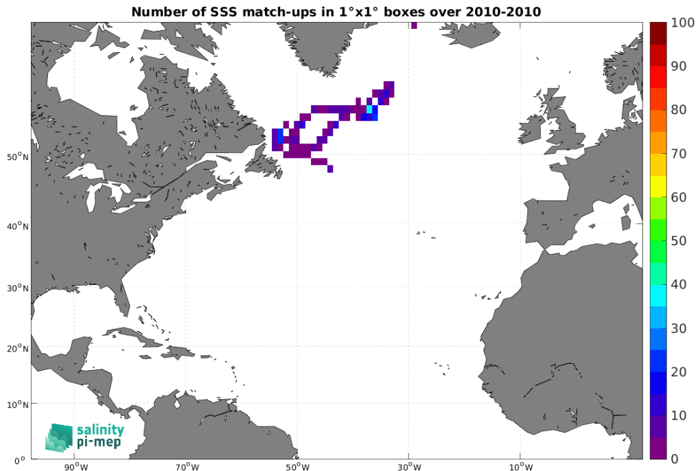
Figure 5: Number of SSS match-ups between Marine mammals SSS and the CCI SSS L4 Merged-OI v4.41 - 7-day running (ESA) SSS product for the North Atlantic Ocean Pi-MEP region over 1^\circ \times 1^\circ boxes and for the full satellite product period.
