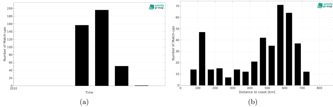
Figure 2: Number of match-ups between Marine mammals and CCI SSS L4 Merged-OI v4.41 - 7-day running (ESA) SSS as a function of time (a) and as function of the distance to coast (b) over the North Atlantic Ocean Pi-MEP region and for the full satellite product period.
