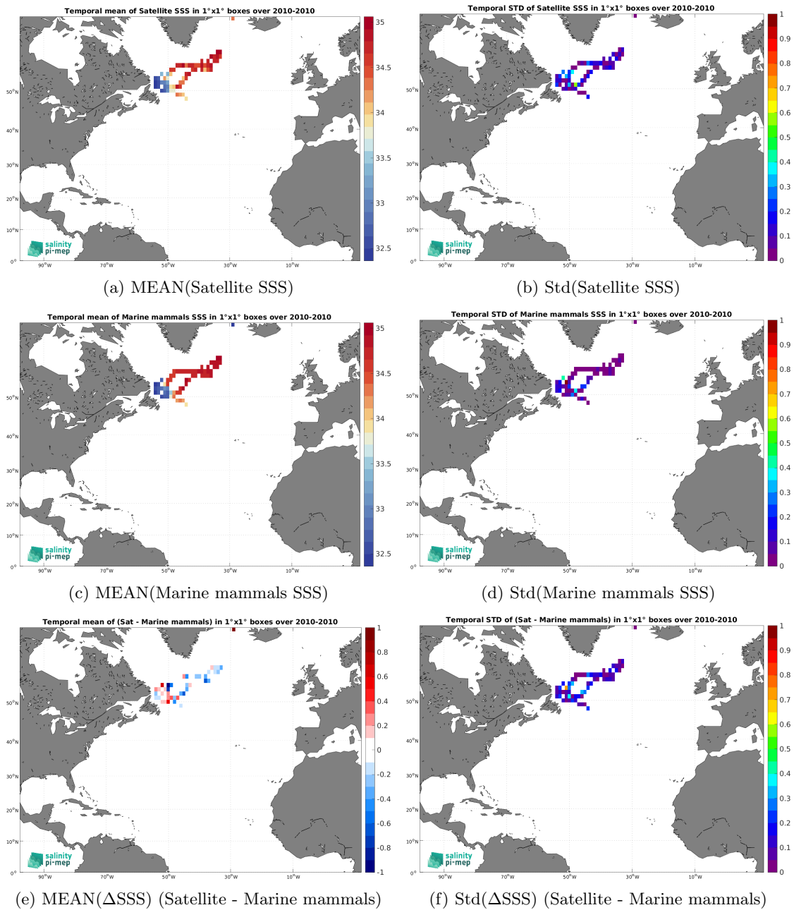
Figure 7: Temporal mean (left) and Std (right) of SSS from CCI SSS L4 Merged-OI v4.41 - 7-day running (ESA) (top), Marine mammals (middle), and of \Delta SSS (Satellite - Marine mammals). Only match-up pairs are used to generate these maps.
