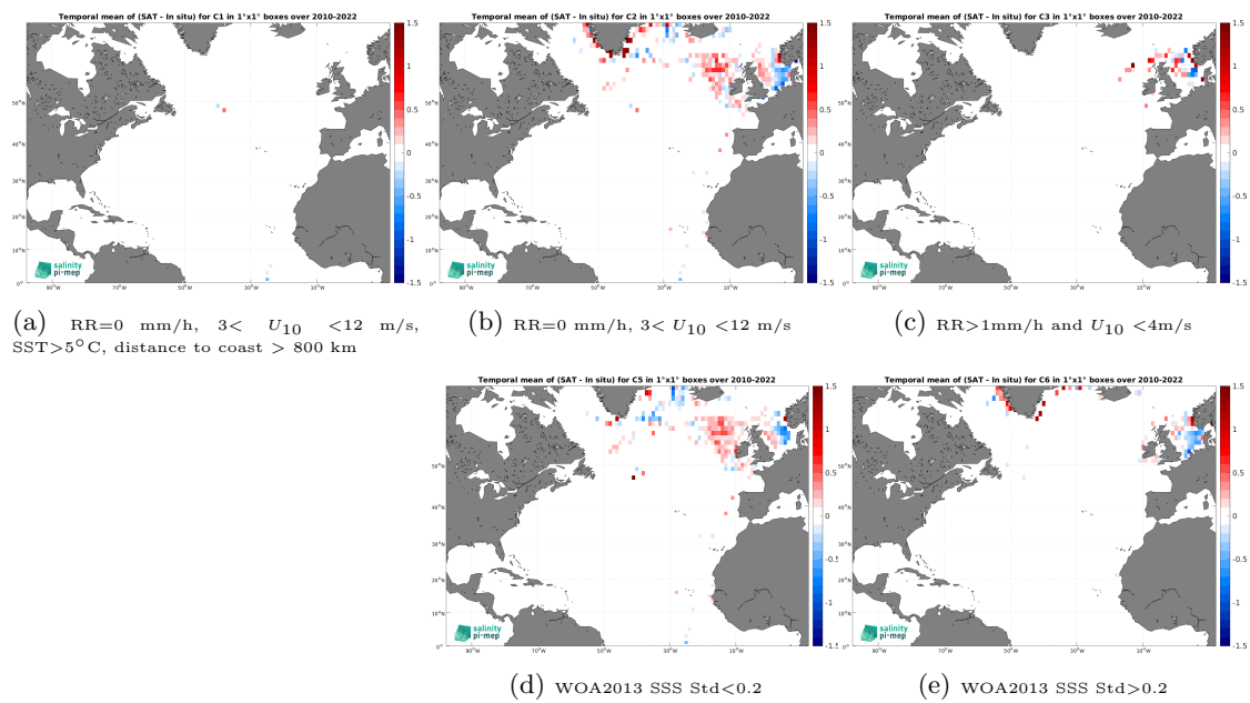
Figure 14: Temporal mean gridded over spatial boxes of size 1^\circ \times 1^\circ of \Delta\text{SSS} (CCI SSS L4 Merged-OI v4.41 - 7-day running (ESA) - ICES) for 5 different subdatasets corresponding to:RR=0 mm/h, 3 < U_{10} < 12 m/s, SST > 5^\circ\text{C} , distance to coast > 800 km (a), RR=0 mm/h, 3 < U_{10} < 12 m/s (b), RR > 1 mm/h and U_{10} < 4 m/s (c), WOA2013 SSS Std < 0.2 (d), WOA2013 SSS Std > 0.2 (e).
