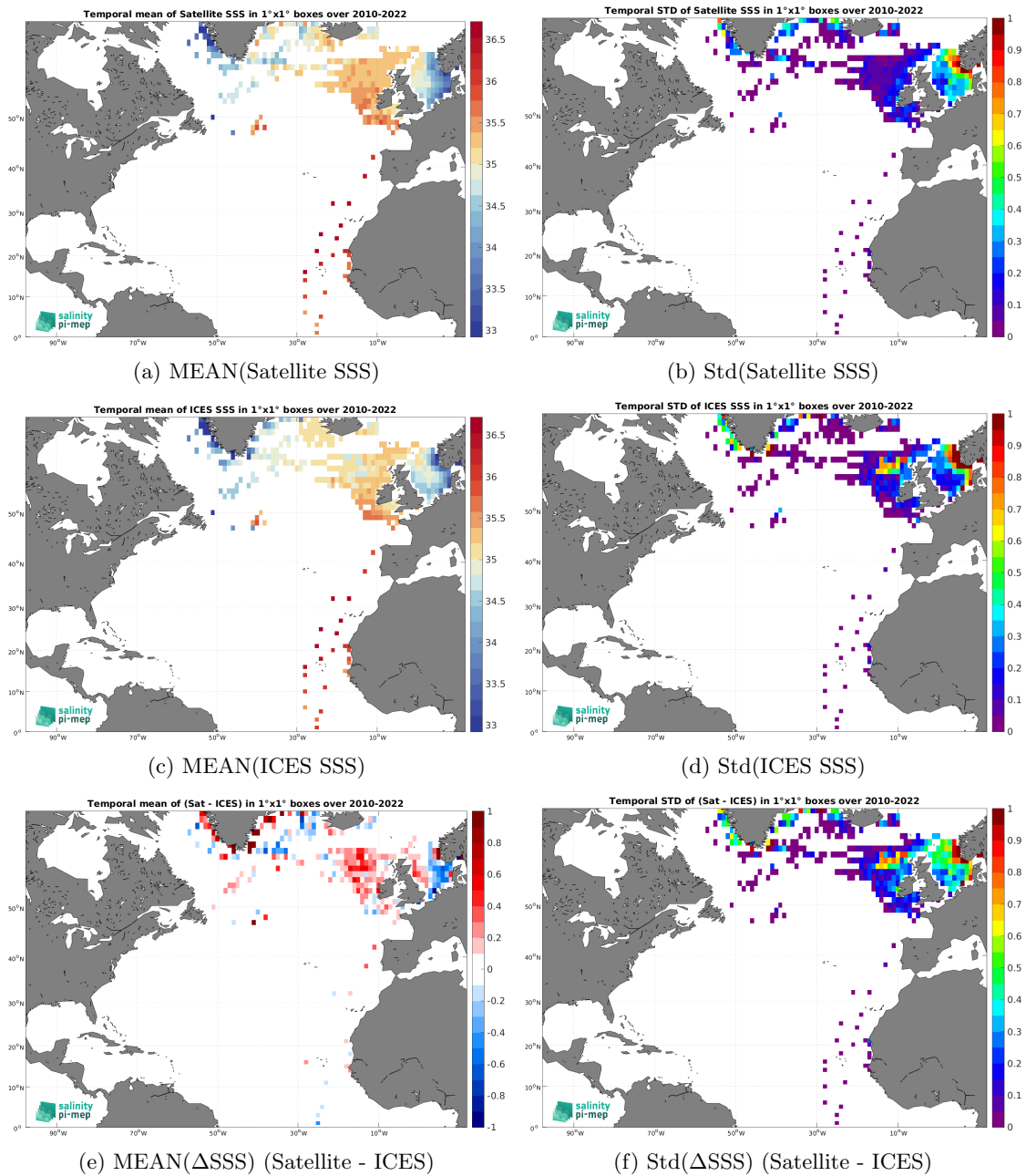
Figure 7: Temporal mean (left) and Std (right) of SSS from CCI SSS L4 Merged-OI v4.41 - 7-day running (ESA) (top), ICES (middle), and of \Delta SSS (Satellite - ICES). Only match-up pairs are used to generate these maps.
