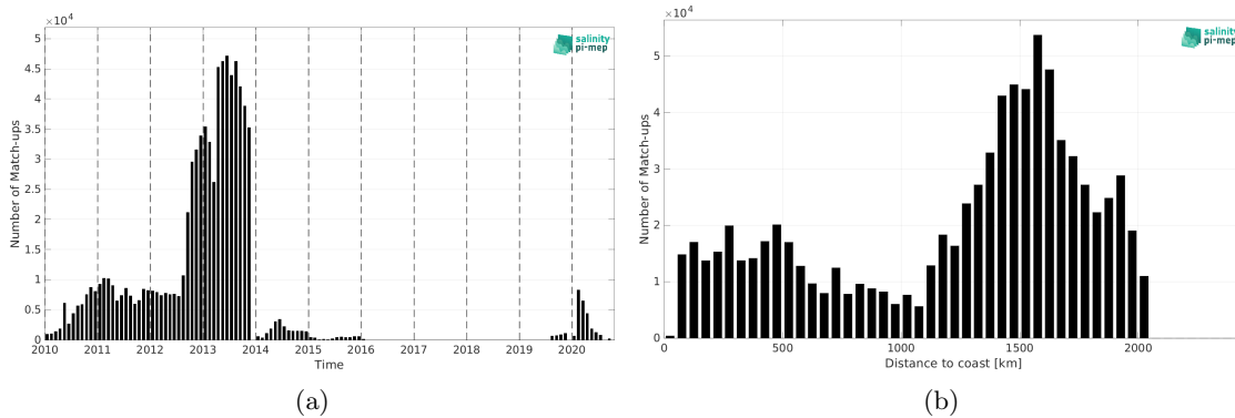
Figure 2: Number of match-ups between Surface drifters and CCI SSS L4 Merged-OI v4.41 - 7-day running (ESA) SSS as a function of time (a) and as function of the distance to coast (b) over the North Atlantic Ocean Pi-MEP region and for the full satellite product period.
