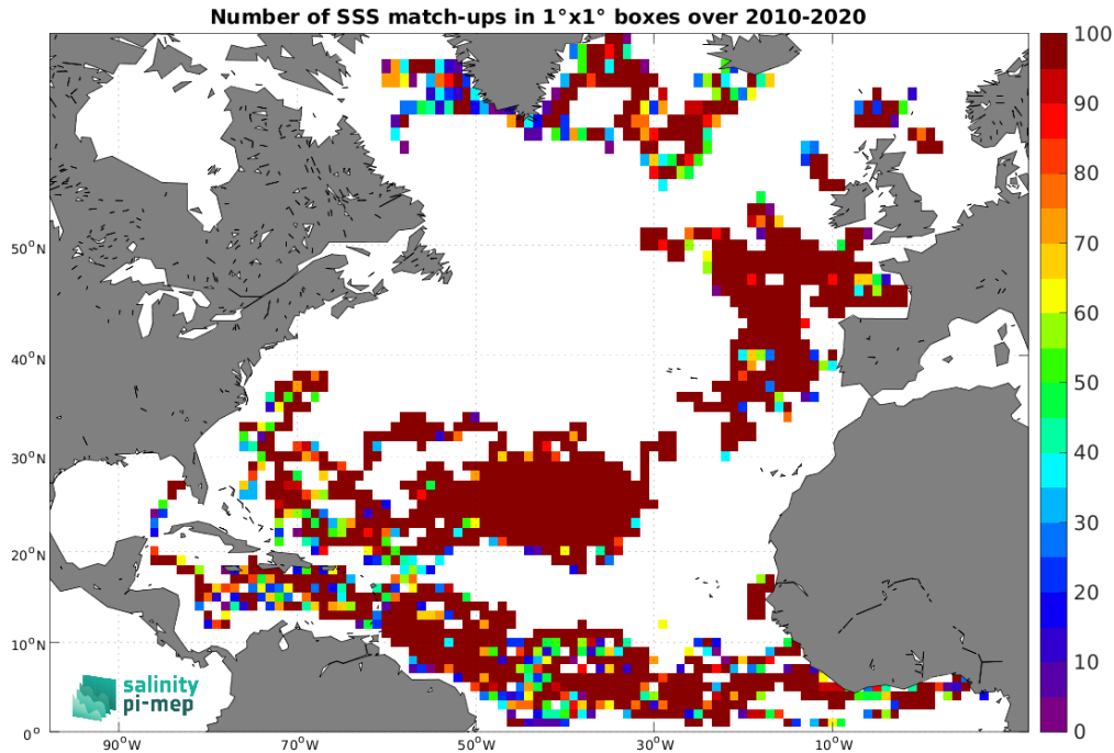
Figure 4: Number of SSS match-ups between Surface drifters SSS and the CCI SSS L4 Merged-OI v4.41 - 7-day running (ESA) SSS product for the North Atlantic Ocean Pi-MEP region over 1^\circ \times 1^\circ boxes and for the full satellite product period.
