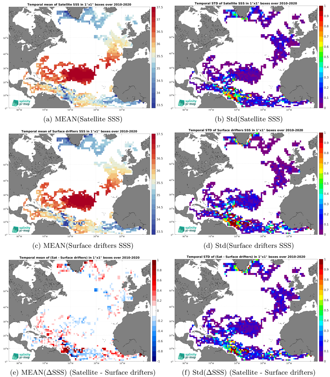
Figure 6: Temporal mean (left) and Std (right) of SSS from CCI SSS L4 Merged-OI v4.41 - 7-day running (ESA) (top), Surface drifters (middle), and of \Delta SSS (Satellite - Surface drifters). Only match-up pairs are used to generate these maps.
