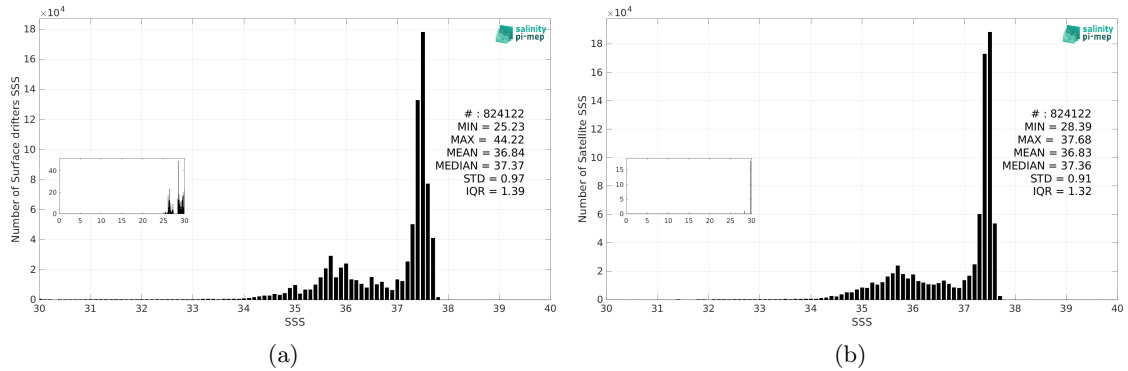
Figure 3: Histograms of SSS from Surface drifters (a) and CCI SSS L4 Merged-OI v4.41 - 7-day running (ESA) (b) considering all match-up pairs per bins of 0.1 over the North Atlantic Ocean Pi-MEP region and for the full satellite product period.
