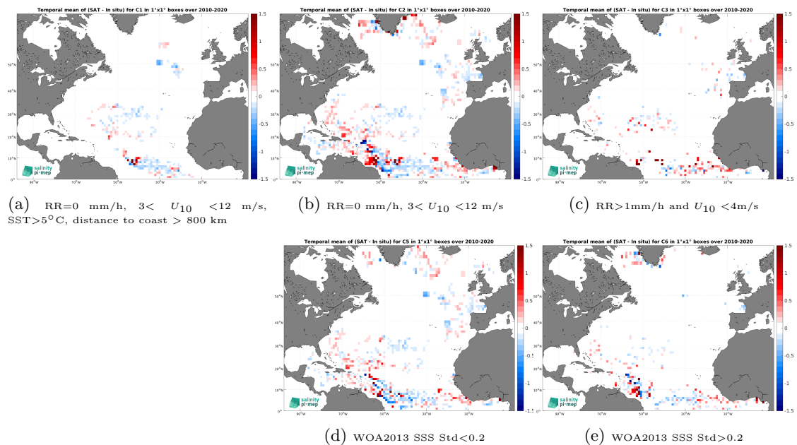
Figure 13: Temporal mean gridded over spatial boxes of size 1^\circ \times 1^\circ of \Delta\text{SSS} (CCI SSS L4 Merged-OI v4.41 - 7-day running (ESA) - Surface drifters) for 5 different subdatasets corresponding to:RR=0 mm/h, 3 < U_{10} < 12 m/s, SST >5^\circ\text{C} , distance to coast > 800 km (a), RR=0 mm/h, 3 < U_{10} < 12 m/s (b), RR >1 mm/h and U_{10} < 4 m/s (c), WOA2013 SSS Std <0.2 (d), WOA2013 SSS Std >0.2 (e).
