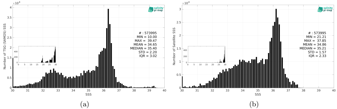
Figure 3: Histograms of SSS from TSG (SAMOS) (a) and CCI SSS L4 Merged-OI v4.41 - 30-day running (ESA) (b) considering all match-up pairs per bins of 0.1 over the North Atlantic Ocean Pi-MEP region and for the full satellite product period.
