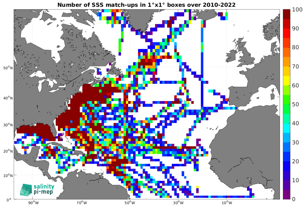
Figure 5: Number of SSS match-ups between TSG (SAMOS) SSS and the CCI SSS L4 Merged-OI v4.41 - 30-day running (ESA) SSS product for the North Atlantic Ocean Pi-MEP region over 1^\circ \times 1^\circ boxes and for the full satellite product period.
