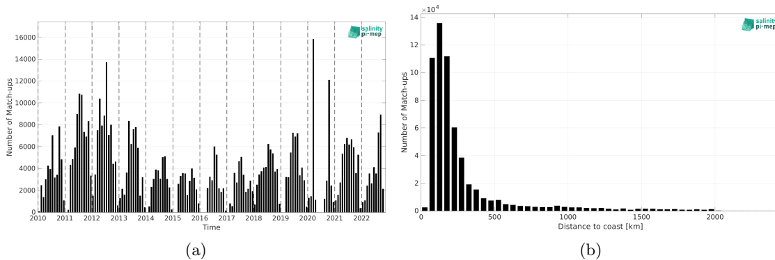
Figure 2: Number of match-ups between TSG (SAMOS) and CCI SSS L4 Merged-OI v4.41 - 30-day running (ESA) SSS as a function of time (a) and as function of the distance to coast (b) over the North Atlantic Ocean Pi-MEP region and for the full satellite product period.
