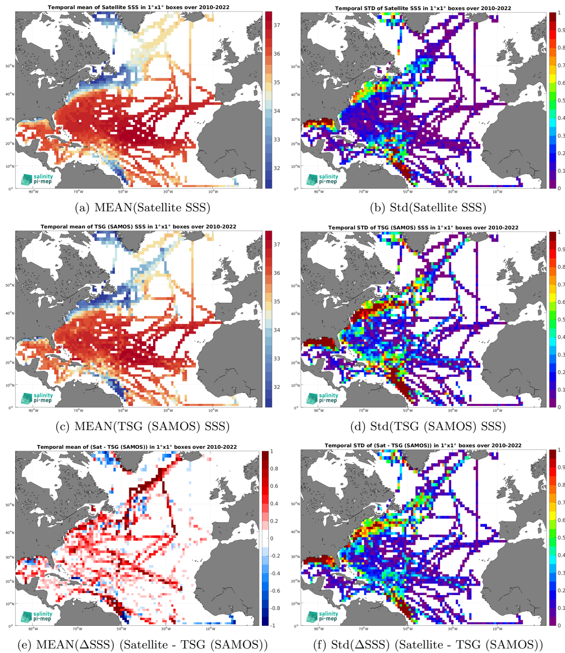
Figure 7: Temporal mean (left) and Std (right) of SSS from CCI SSS L4 Merged-OI v4.41 - 30-day running (ESA) (top), TSG (SAMOS) (middle), and of \Delta SSS (Satellite - TSG (SAMOS)). Only match-up pairs are used to generate these maps.
