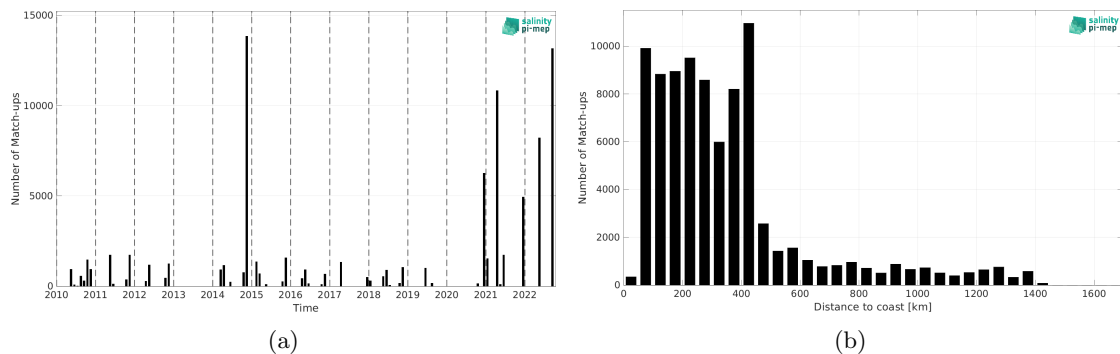
Figure 2: Number of match-ups between TSG (Polarstern) and CCI SSS L4 Merged-OI v4.41 - 30-day running (ESA) SSS as a function of time (a) and as function of the distance to coast (b) over the North Atlantic Ocean Pi-MEP region and for the full satellite product period.
