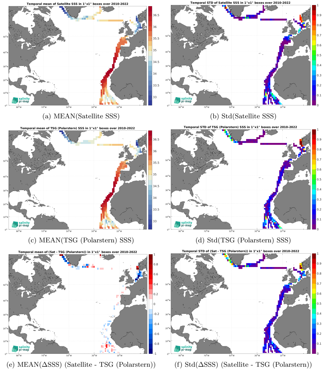
Figure 7: Temporal mean (left) and Std (right) of SSS from CCI SSS L4 Merged-OI v4.41 - 30-day running (ESA) (top), TSG (Polarstern) (middle), and of \Delta SSS (Satellite - TSG (Polarstern)). Only match-up pairs are used to generate these maps.
