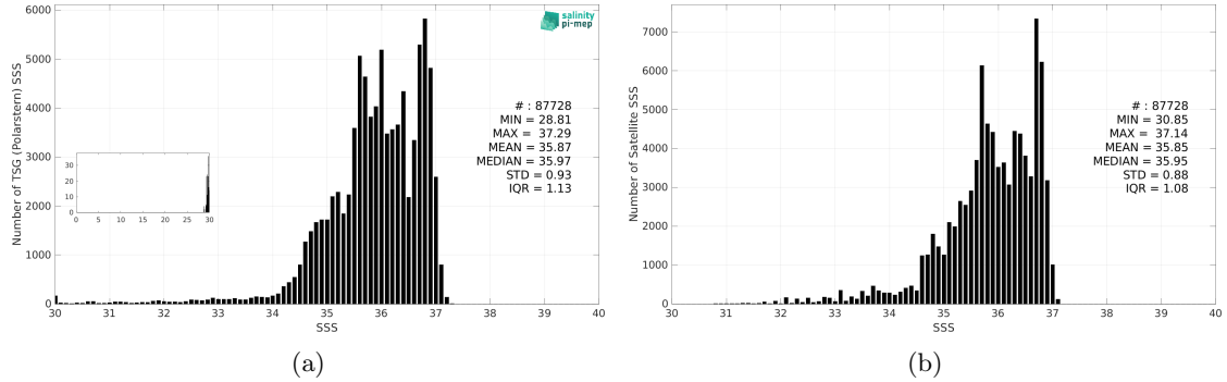
Figure 3: Histograms of SSS from TSG (Polarstern) (a) and CCI SSS L4 Merged-OI v4.41 - 30-day running (ESA) (b) considering all match-up pairs per bins of 0.1 over the North Atlantic Ocean Pi-MEP region and for the full satellite product period.
