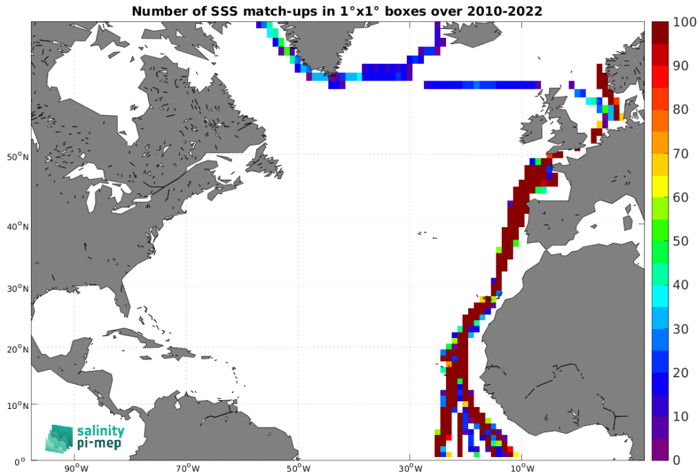
Figure 5: Number of SSS match-ups between TSG (Polarstern) SSS and the CCI SSS L4 Merged-OI v4.41 - 30-day running (ESA) SSS product for the North Atlantic Ocean Pi-MEP region over 1^\circ \times 1^\circ boxes and for the full satellite product period.
