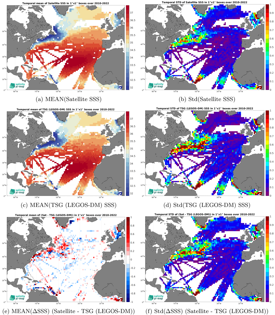
Figure 7: Temporal mean (left) and Std (right) of SSS from CCI SSS L4 Merged-OI v4.41 - 30-day running (ESA) (top), TSG (LEGOS-DM) (middle), and of \Delta SSS (Satellite - TSG (LEGOS-DM)). Only match-up pairs are used to generate these maps.
