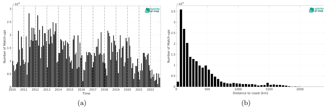
Figure 2: Number of match-ups between TSG (LEGOS-DM) and CCI SSS L4 Merged-OI v4.41 - 30-day running (ESA) SSS as a function of time (a) and as function of the distance to coast (b) over the North Atlantic Ocean Pi-MEP region and for the full satellite product period.
