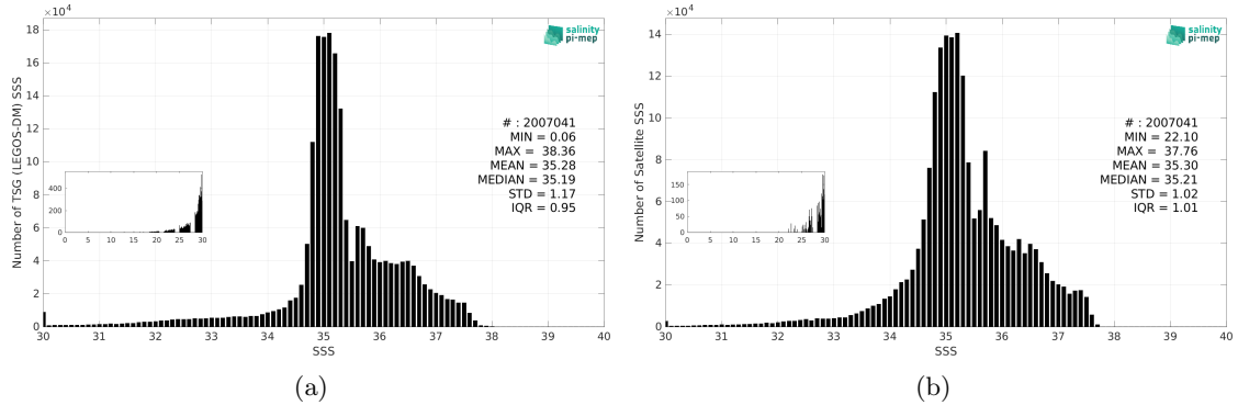
Figure 3: Histograms of SSS from TSG (LEGOS-DM) (a) and CCI SSS L4 Merged-OI v4.41 - 30-day running (ESA) (b) considering all match-up pairs per bins of 0.1 over the North Atlantic Ocean Pi-MEP region and for the full satellite product period.
