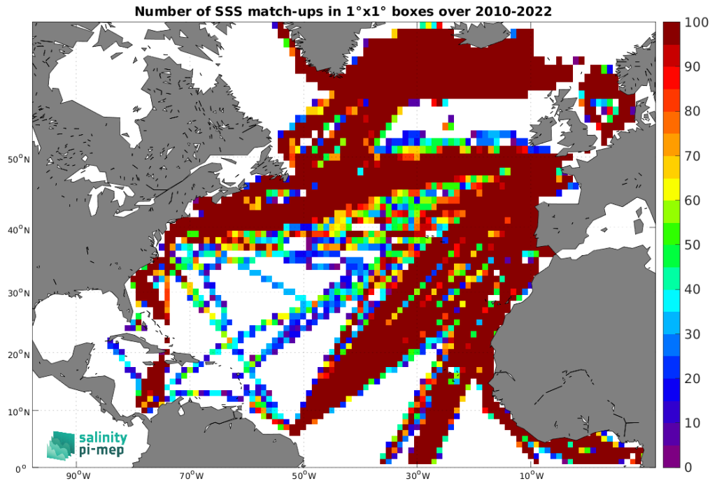
Figure 5: Number of SSS match-ups between TSG (LEGOS-DM) SSS and the CCI SSS L4 Merged-OI v4.41 - 30-day running (ESA) SSS product for the North Atlantic Ocean Pi-MEP region over 1^\circ \times 1^\circ boxes and for the full satellite product period.
