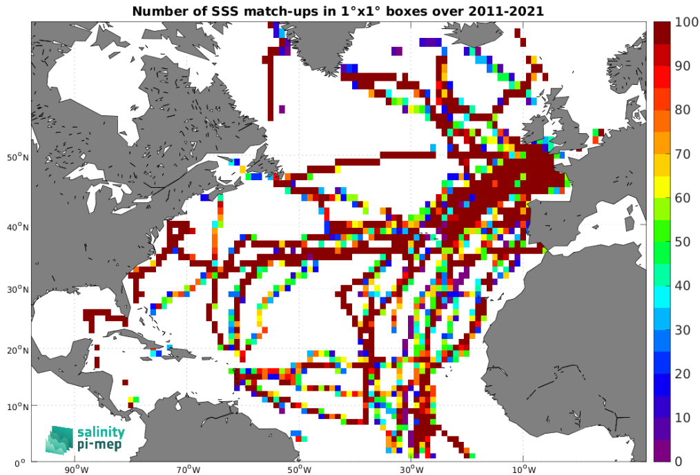
Figure 5: Number of SSS match-ups between TSG (GOSUD-Sailing-ship) SSS and the CCI SSS L4 Merged-OI v4.41 - 30-day running (ESA) SSS product for the North Atlantic Ocean Pi-MEP region over 1^\circ \times 1^\circ boxes and for the full satellite product period.
