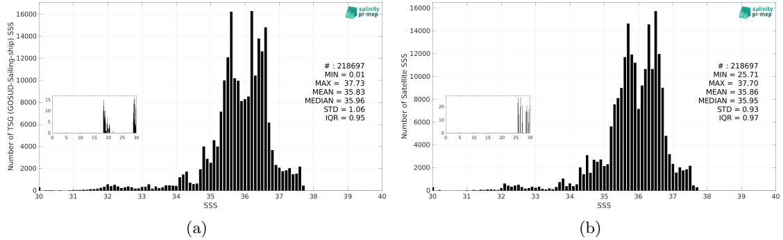
Figure 3: Histograms of SSS from TSG (GOSUD-Sailing-ship) (a) and CCI SSS L4 Merged-OI v4.41 - 30-day running (ESA) (b) considering all match-up pairs per bins of 0.1 over the North Atlantic Ocean Pi-MEP region and for the full satellite product period.
