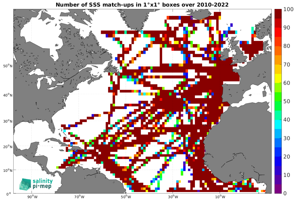
Figure 5: Number of SSS match-ups between TSG (GOSUD-Research-vessel) SSS and the CCI SSS L4 Merged-OI v4.41 - 30-day running (ESA) SSS product for the North Atlantic Ocean Pi-MEP region over 1^\circ \times 1^\circ boxes and for the full satellite product period.
