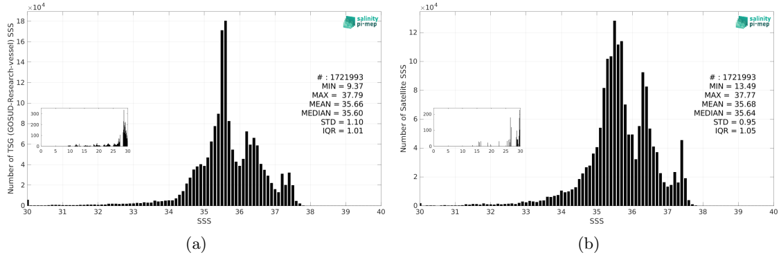
Figure 3: Histograms of SSS from TSG (GOSUD-Research-vessel) (a) and CCI SSS L4 Merged-OI v4.41 - 30-day running (ESA) (b) considering all match-up pairs per bins of 0.1 over the North Atlantic Ocean Pi-MEP region and for the full satellite product period.
