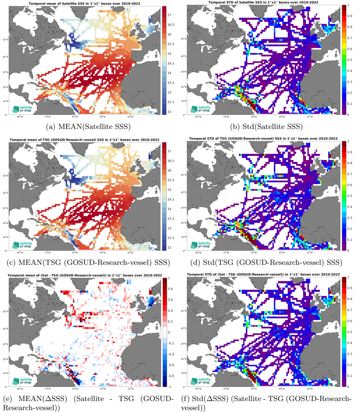
Figure 7: Temporal mean (left) and Std (right) of SSS from CCI SSS L4 Merged-OI v4.41 - 30-day running (ESA) (top), TSG (GOSUD-Research-vessel) (middle), and of \Delta SSS (Satellite - TSG (GOSUD-Research-vessel)). Only match-up pairs are used to generate these maps.
