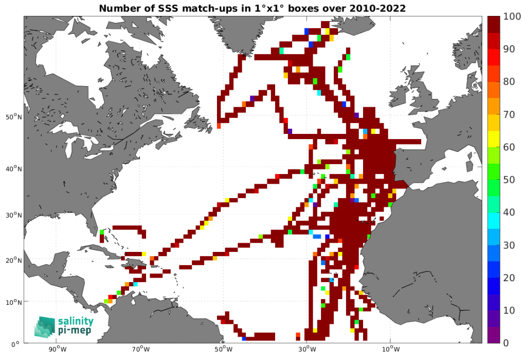
Figure 5: Number of SSS match-ups between TSG (CSIC-UTM) SSS and the CCI SSS L4 Merged-OI v4.41 - 30-day running (ESA) SSS product for the North Atlantic Ocean Pi-MEP region over 1^\circ \times 1^\circ boxes and for the full satellite product period.
