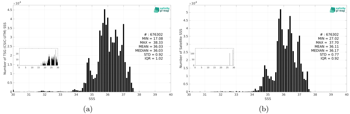
Figure 3: Histograms of SSS from TSG (CSIC-UTM) (a) and CCI SSS L4 Merged-OI v4.41 - 30-day running (ESA) (b) considering all match-up pairs per bins of 0.1 over the North Atlantic Ocean Pi-MEP region and for the full satellite product period.
