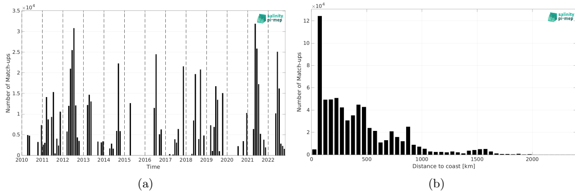
Figure 2: Number of match-ups between TSG (CSIC-UTM) and CCI SSS L4 Merged-OI v4.41 - 30-day running (ESA) SSS as a function of time (a) and as function of the distance to coast (b) over the North Atlantic Ocean Pi-MEP region and for the full satellite product period.
