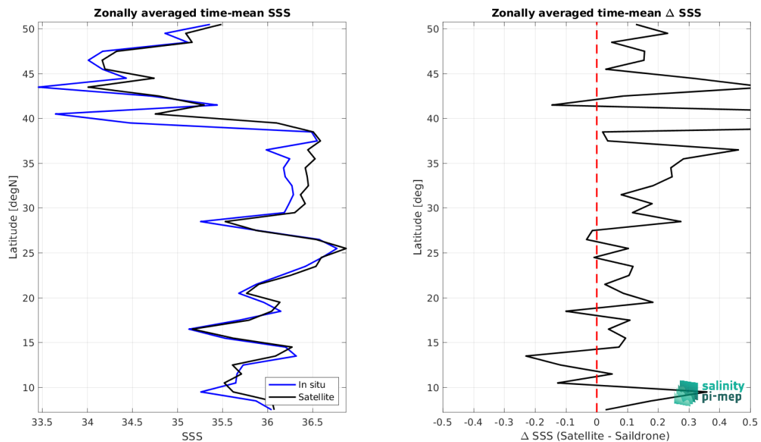
Figure 9: Left panel: Zonal mean SSS from CCI SSS L4 Merged-OI v4.41 - 30-day running (ESA) satellite product (black) and from Saildrone (blue). Right panel: Zonal mean of \Delta SSS (Satellite - Saildrone) for all the collected Pi-MEP match-up pairs estimated over the full satellite product period.
