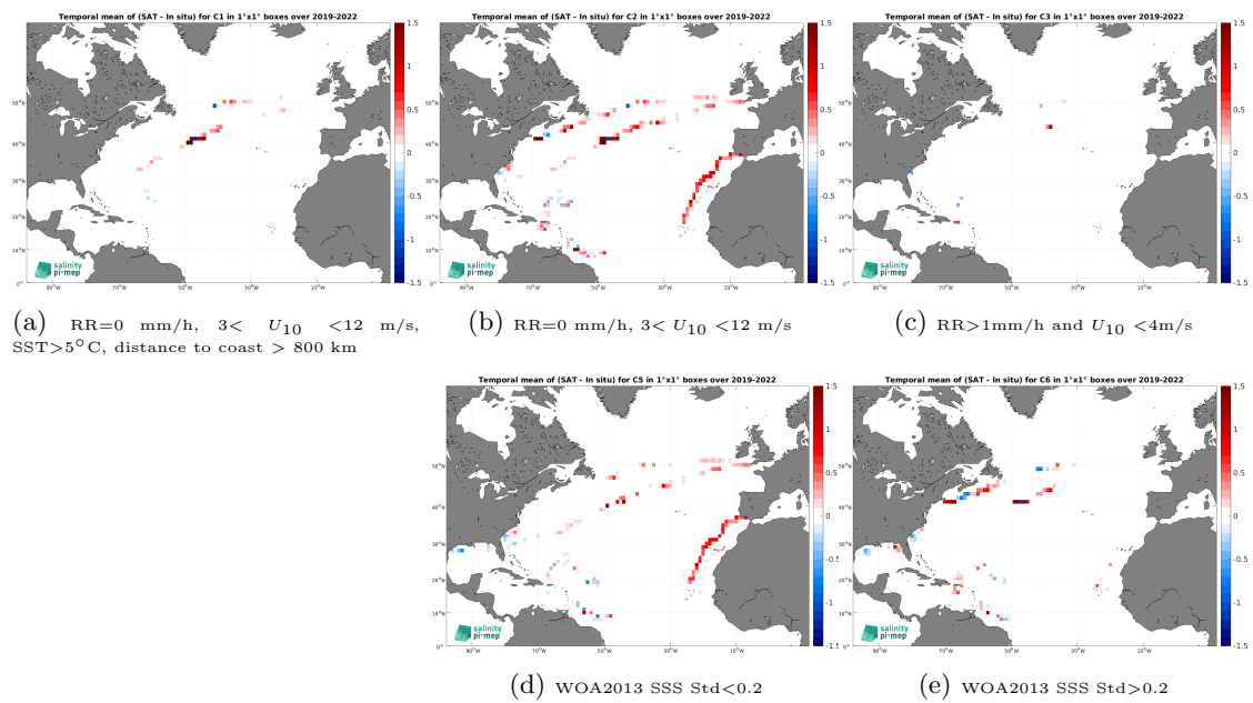
Figure 14: Temporal mean gridded over spatial boxes of size 1^\circ \times 1^\circ of \Delta\text{SSS} (CCI SSS L4 Merged-OI v4.41 - 30-day running (ESA) - Saildrone) for 5 different subdatasets corresponding to:RR=0 mm/h, 3 < U_{10} < 12 m/s, SST >5^\circ\text{C} , distance to coast > 800 km (a), RR=0 mm/h, 3 < U_{10} < 12 m/s (b), RR >1 mm/h and U_{10} < 4 m/s (c), WOA2013 SSS Std <0.2 (d), WOA2013 SSS Std >0.2 (e).
