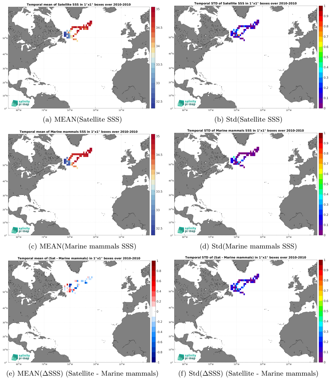
Figure 7: Temporal mean (left) and Std (right) of SSS from CCI SSS L4 Merged-OI v4.41 - 30-day running (ESA) (top), Marine mammals (middle), and of \Delta SSS (Satellite - Marine mammals). Only match-up pairs are used to generate these maps.
