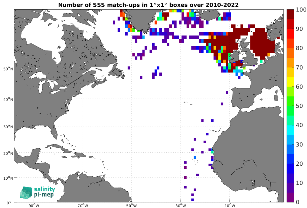
Figure 5: Number of SSS match-ups between ICES SSS and the CCI SSS L4 Merged-OI v4.41 - 30-day running (ESA) SSS product for the North Atlantic Ocean Pi-MEP region over 1^\circ \times 1^\circ boxes and for the full satellite product period.
