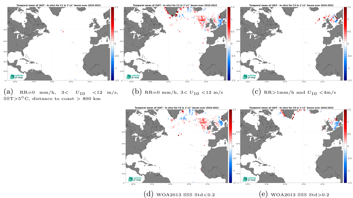
Figure 14: Temporal mean gridded over spatial boxes of size 1^\circ \times 1^\circ of \Delta\text{SSS} (CCI SSS L4 Merged-OI v4.41 - 30-day running (ESA) - ICES) for 5 different subdatasets corresponding to:RR=0 mm/h, 3 < U_{10} < 12 m/s, SST >5^\circ\text{C} , distance to coast > 800 km (a), RR=0 mm/h, 3 < U_{10} < 12 m/s (b), RR >1 mm/h and U_{10} < 4 m/s (c), WOA2013 SSS Std <0.2 (d), WOA2013 SSS Std >0.2 (e).
