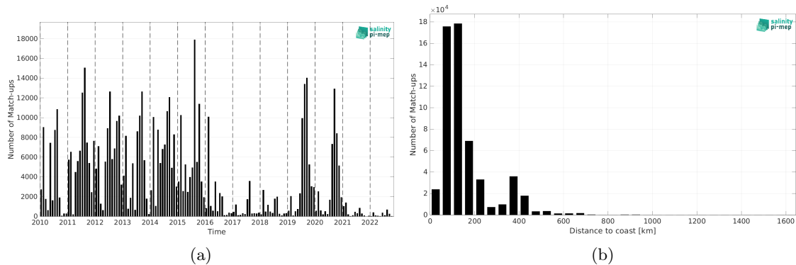
Figure 2: Number of match-ups between ICES and CCI SSS L4 Merged-OI v4.41 - 30-day running (ESA) SSS as a function of time (a) and as function of the distance to coast (b) over the North Atlantic Ocean Pi-MEP region and for the full satellite product period.
