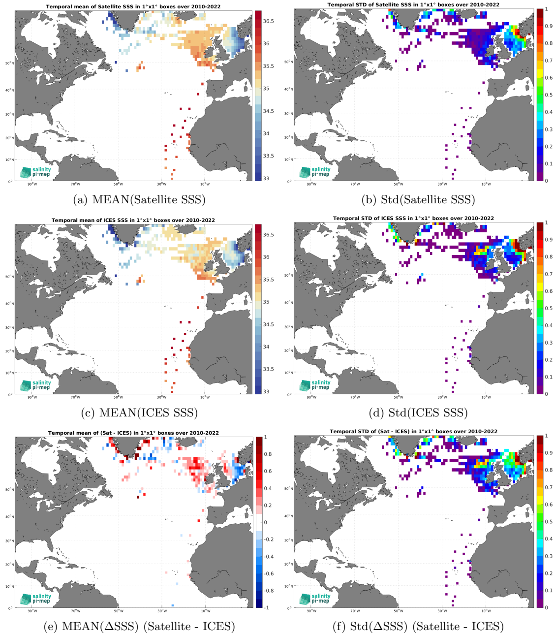
Figure 7: Temporal mean (left) and Std (right) of SSS from CCI SSS L4 Merged-OI v4.41 - 30-day running (ESA) (top), ICES (middle), and of \Delta SSS (Satellite - ICES). Only match-up pairs are used to generate these maps.
