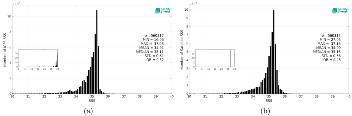
Figure 3: Histograms of SSS from ICES (a) and CCI SSS L4 Merged-OI v4.41 - 30-day running (ESA) (b) considering all match-up pairs per bins of 0.1 over the North Atlantic Ocean Pi-MEP region and for the full satellite product period.
