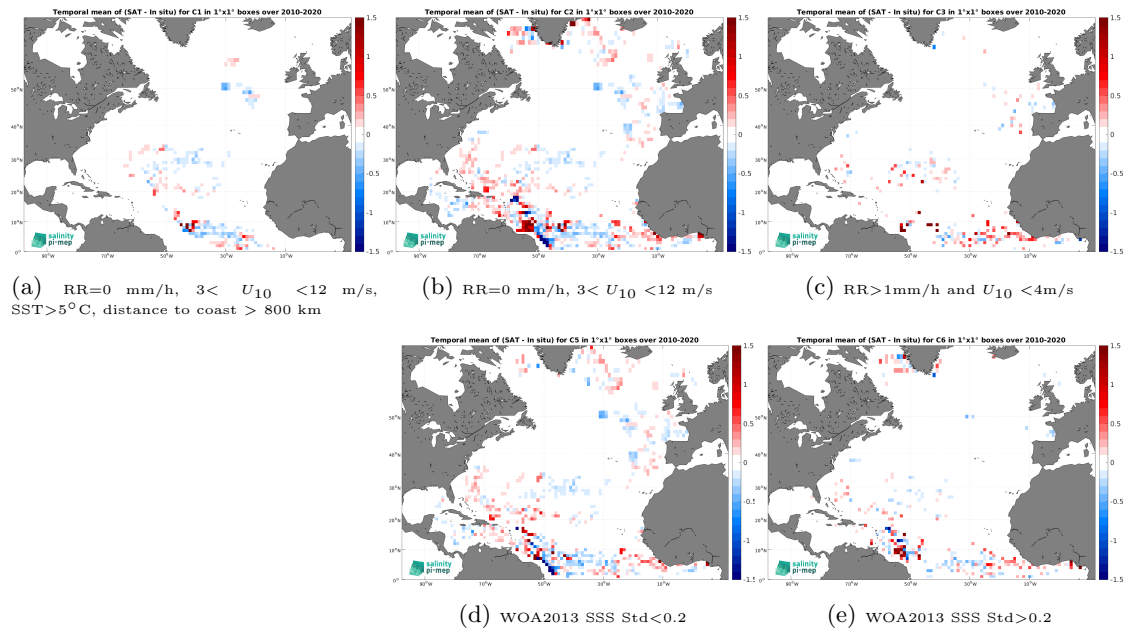
Figure 13: Temporal mean gridded over spatial boxes of size 1^\circ \times 1^\circ of \Delta\text{SSS} (CCI SSS L4 Merged-OI v4.41 - 30-day running (ESA) - Surface drifters) for 5 different subdatasets corresponding to:RR=0 mm/h, 3 < U_{10} < 12 m/s, SST >5^\circ\text{C} , distance to coast > 800 km (a), RR=0 mm/h, 3 < U_{10} < 12 m/s (b), RR >1 mm/h and U_{10} < 4 m/s (c), WOA2013 SSS Std <0.2 (d), WOA2013 SSS Std >0.2 (e).
