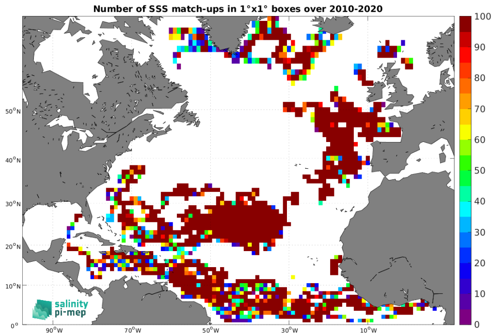
Figure 4: Number of SSS match-ups between Surface drifters SSS and the CCI SSS L4 Merged-OI v4.41 - 30-day running (ESA) SSS product for the North Atlantic Ocean Pi-MEP region over 1^\circ \times 1^\circ boxes and for the full satellite product period.
