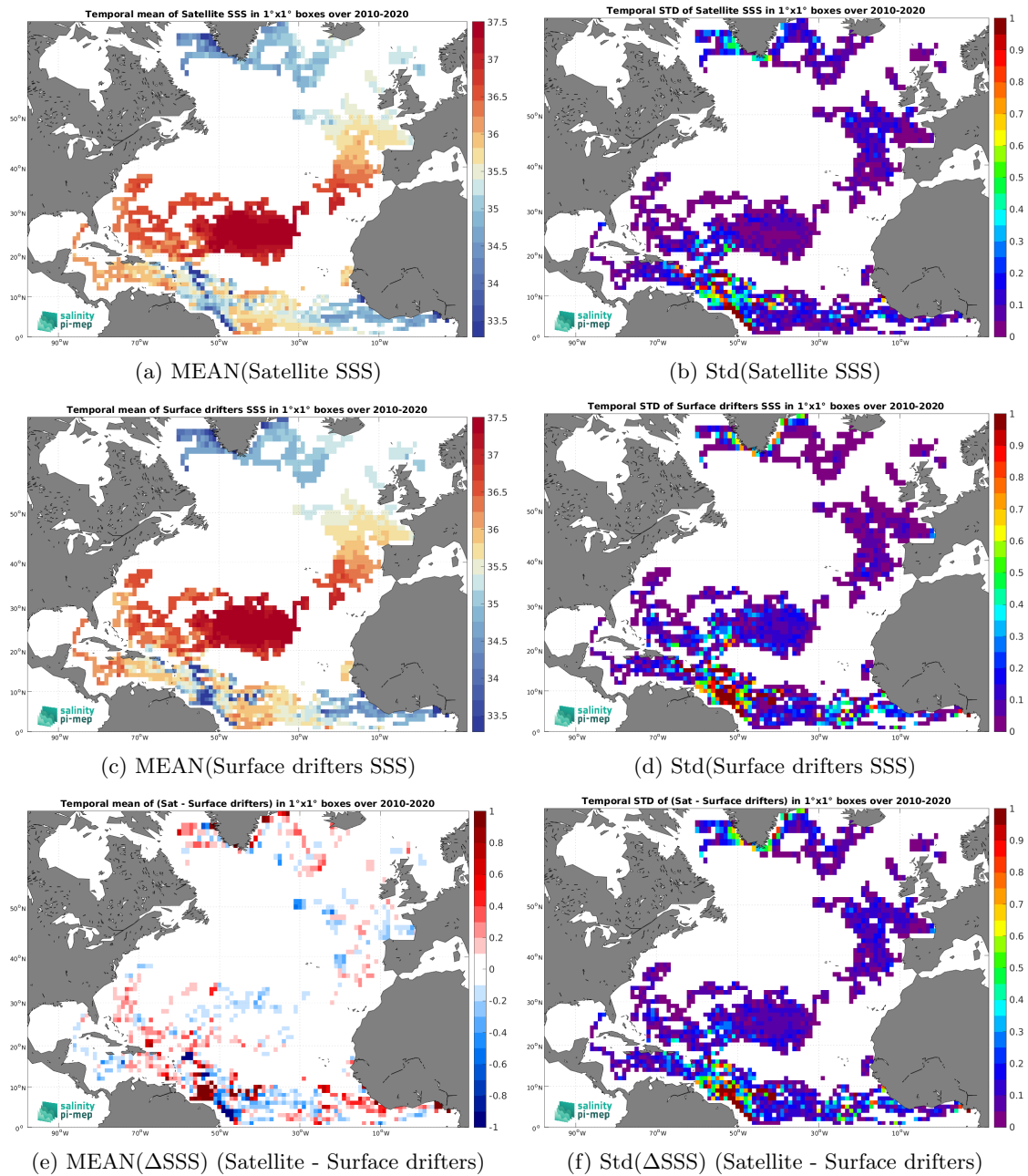
Figure 6: Temporal mean (left) and Std (right) of SSS from CCI SSS L4 Merged-OI v4.41 - 30-day running (ESA) (top), Surface drifters (middle), and of \Delta SSS (Satellite - Surface drifters). Only match-up pairs are used to generate these maps.
