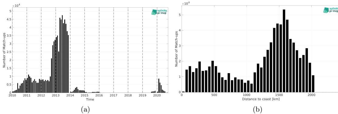
Figure 2: Number of match-ups between Surface drifters and CCI SSS L4 Merged-OI v4.41 - 30-day running (ESA) SSS as a function of time (a) and as function of the distance to coast (b) over the North Atlantic Ocean Pi-MEP region and for the full satellite product period.
