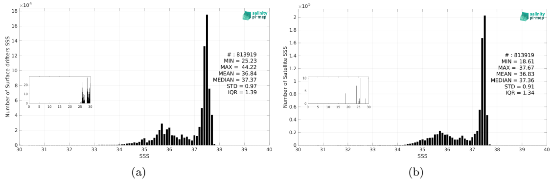
Figure 3: Histograms of SSS from Surface drifters (a) and CCI SSS L4 Merged-OI v4.41 - 30-day running (ESA) (b) considering all match-up pairs per bins of 0.1 over the North Atlantic Ocean Pi-MEP region and for the full satellite product period.
