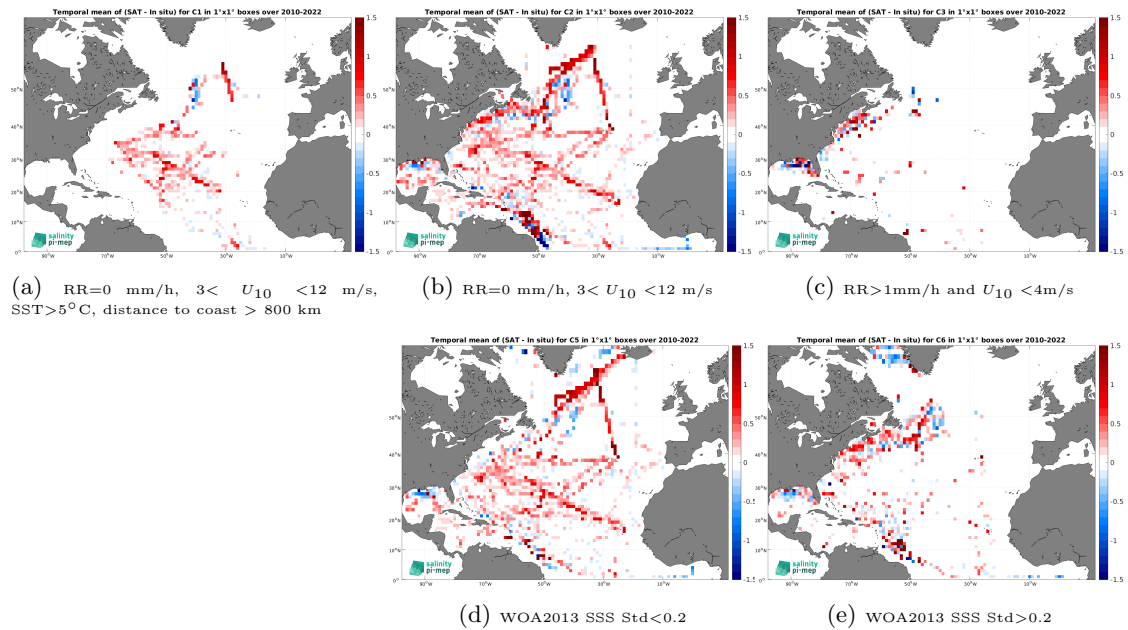
Figure 12: Temporal mean gridded over spatial boxes of size 1^\circ \times 1^\circ of \Delta\text{SSS} (CCI SSS L4 Merged-OI v4.4 - 7-day running (ESA) - TSG (SAMOS)) for 5 different subdatasets corresponding to:RR=0 mm/h, 3 < U_{10} < 12 m/s, SST >5^\circ\text{C} , distance to coast > 800 km (a), RR=0 mm/h, 3 < U_{10} < 12 m/s (b), RR >1 mm/h and U_{10} < 4 m/s (c), WOA2013 SSS Std <0.2 (d), WOA2013 SSS Std >0.2 (e).
