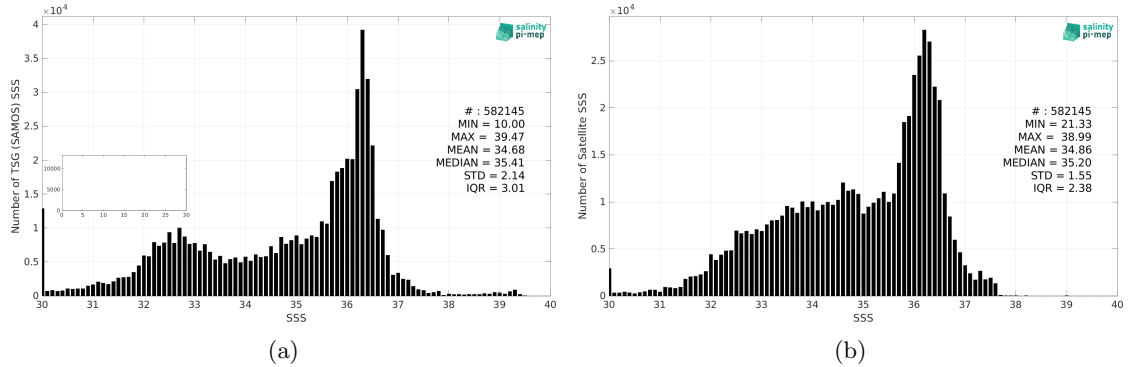
Figure 2: Histograms of SSS from TSG (SAMOS) (a) and CCI SSS L4 Merged-OI v4.4 - 7-day running (ESA) (b) considering all match-up pairs per bins of 0.1 over the North Atlantic Ocean Pi-MEP region and for the full satellite product period.
