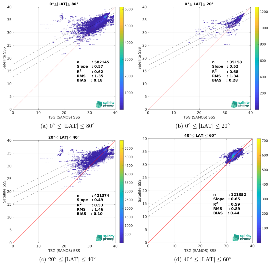
Figure 9: Contour maps of the concentration of CCI SSS L4 Merged-OI v4.4 - 7-day running (ESA) SSS (y-axis) versus TSG (SAMOS) SSS (x-axis) at match-up pairs for different latitude bands. For each plot, the red line shows x=y . The black thin and dashed lines indicate a linear fit through the data cloud and the \pm 95\% confidence levels, respectively. The number match-up pairs n , the slope and R^2 coefficient of the linear fit, the root mean square (RMS) and the mean bias between satellite and in situ data are indicated for each latitude band in each plots.
