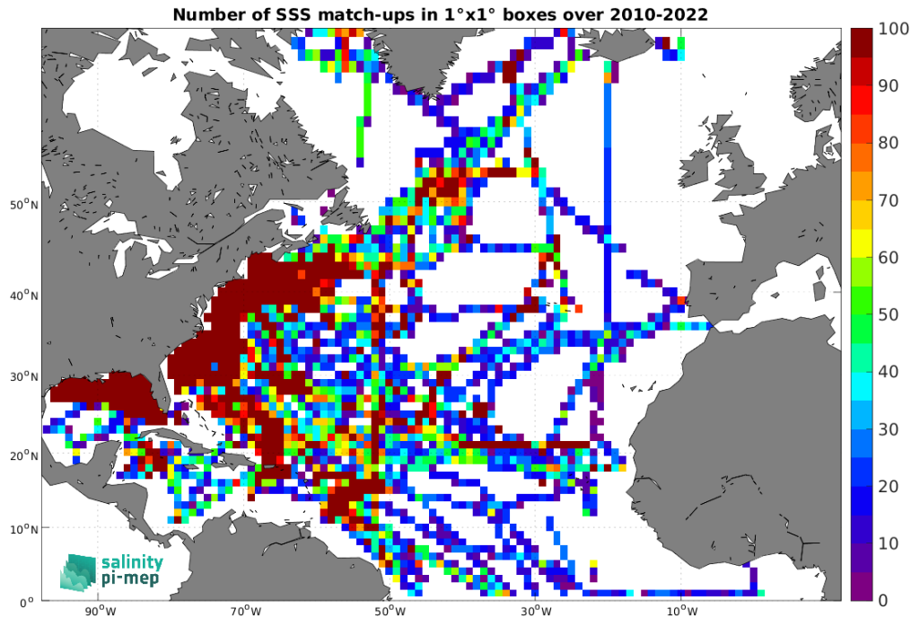
Figure 4: Number of SSS match-ups between TSG (SAMOS) SSS and the CCI SSS L4 Merged-OI v4.4 - 7-day running (ESA) SSS product for the North Atlantic Ocean Pi-MEP region over 1^\circ \times 1^\circ boxes and for the full satellite product period.
