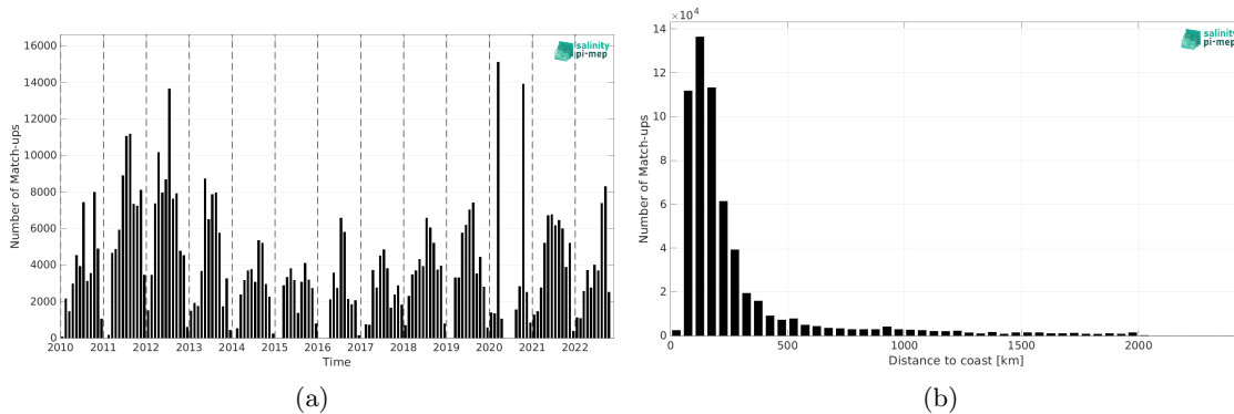
Figure 1: Number of match-ups between TSG (SAMOS) and CCI SSS L4 Merged-OI v4.4 - 7-day running (ESA) SSS as a function of time (a) and as function of the distance to coast (b) over the North Atlantic Ocean Pi-MEP region and for the full satellite product period.
