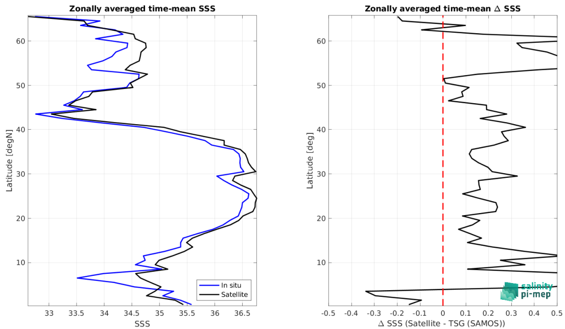
Figure 8: Left panel: Zonal mean SSS from CCI SSS L4 Merged-OI v4.4 - 7-day running (ESA) satellite product (black) and from TSG (SAMOS) (blue). Right panel: Zonal mean of \Delta SSS (Satellite - TSG (SAMOS)) for all the collected Pi-MEP match-up pairs estimated over the full satellite product period.
