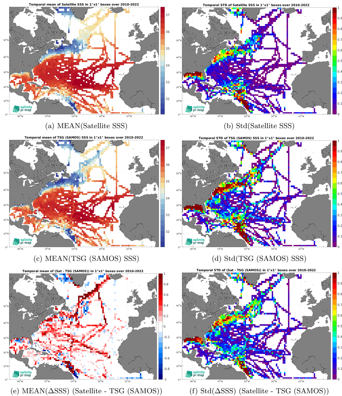
Figure 6: Temporal mean (left) and Std (right) of SSS from CCI SSS L4 Merged-OI v4.4 - 7-day running (ESA) (top), TSG (SAMOS) (middle), and of \Delta SSS (Satellite - TSG (SAMOS)). Only match-up pairs are used to generate these maps.
