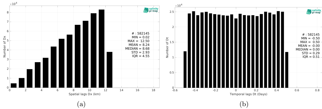
Figure 5: Histograms of the spatial (a) and temporal (b) lags between the location/time of the TSG (SAMOS) measurement and the date of the corresponding CCI SSS L4 Merged-OI v4.4 - 7-day running (ESA) SSS pixel.
