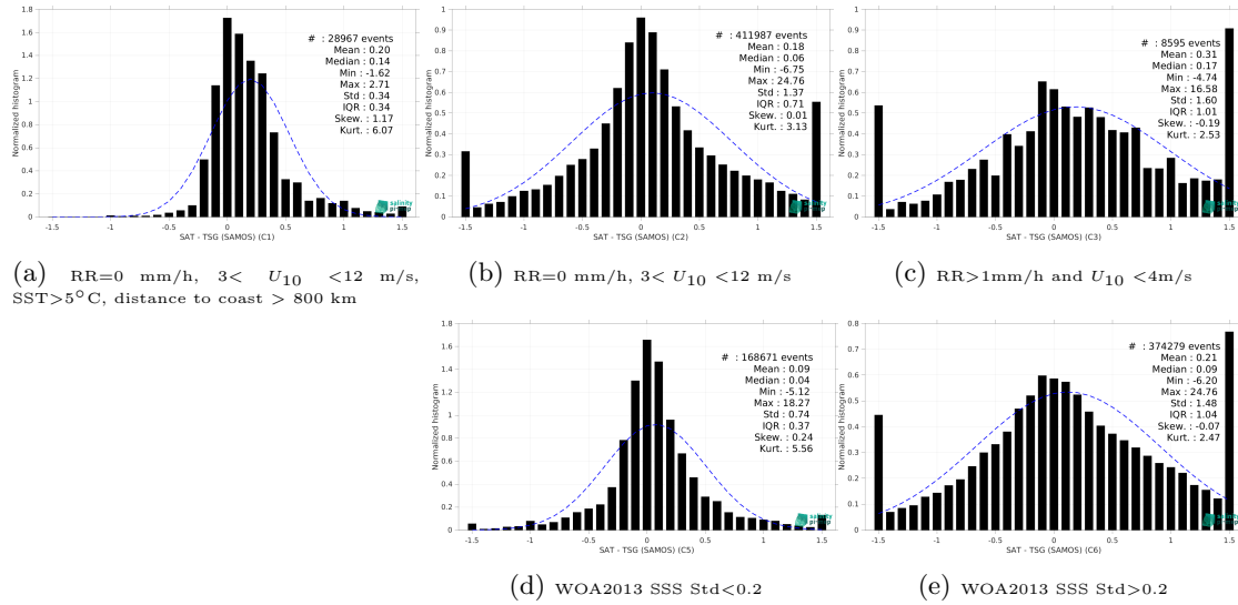
Figure 13: Normalized histogram of \Delta SSS (CCI SSS L4 Merged-OI v4.4 - 7-day running (ESA) - TSG (SAMOS)) for 5 different subdatasets corresponding to: RR=0 mm/h, 3 < U_{10} < 12 m/s, SST>5°C, distance to coast > 800 km (a), RR=0 mm/h, 3 < U_{10} < 12 m/s (b), RR>1mm/h and U_{10} < 4 m/s (c), WOA2013 SSS Std<0.2 (d), WOA2013 SSS Std>0.2 (e).
