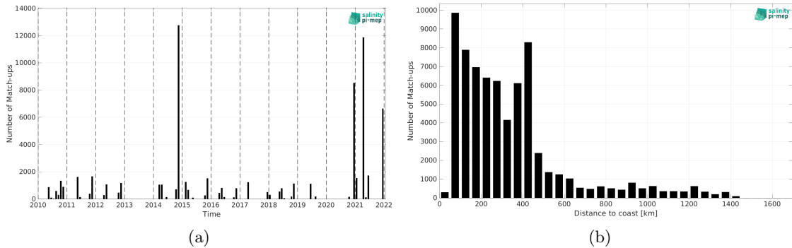
Figure 1: Number of match-ups between TSG (Polarstern) and CCI SSS L4 Merged-OI v4.4 - 7-day running (ESA) SSS as a function of time (a) and as function of the distance to coast (b) over the North Atlantic Ocean Pi-MEP region and for the full satellite product period.
