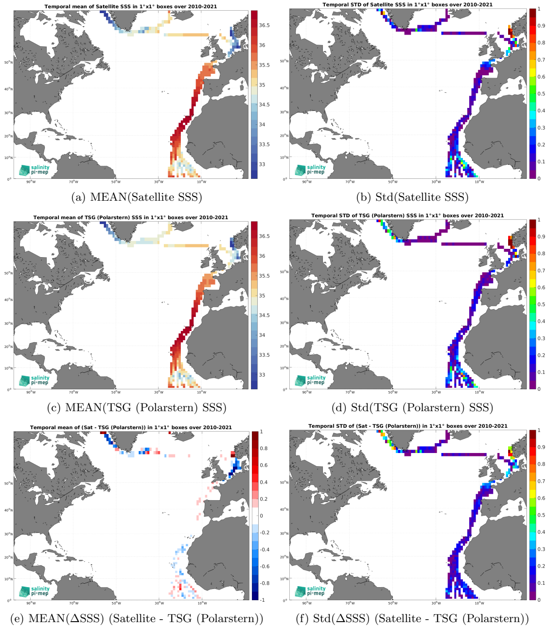
Figure 6: Temporal mean (left) and Std (right) of SSS from CCI SSS L4 Merged-OI v4.4 - 7-day running (ESA) (top), TSG (Polarstern) (middle), and of \Delta SSS (Satellite - TSG (Polarstern)). Only match-up pairs are used to generate these maps.
