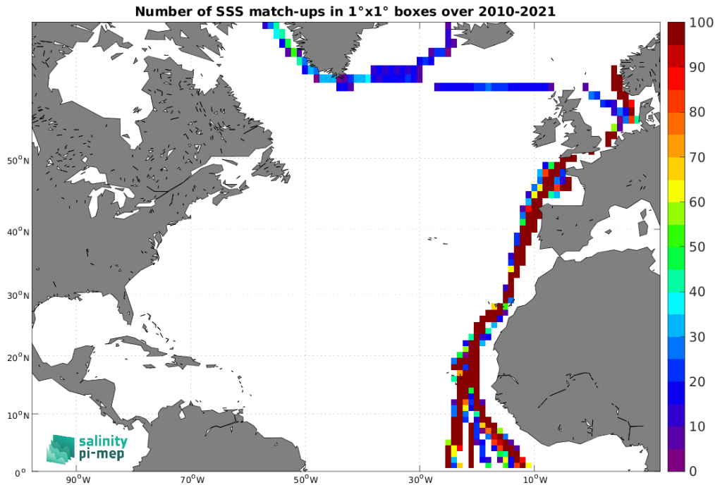
Figure 4: Number of SSS match-ups between TSG (Polarstern) SSS and the CCI SSS L4 Merged-OI v4.4 - 7-day running (ESA) SSS product for the North Atlantic Ocean Pi-MEP region over 1^\circ \times 1^\circ boxes and for the full satellite product period.
