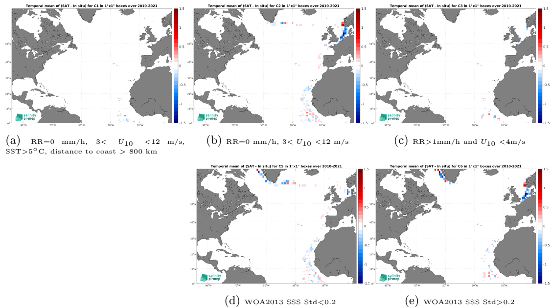
Figure 12: Temporal mean gridded over spatial boxes of size 1^\circ \times 1^\circ of \Delta\text{SSS} (CCI SSS L4 Merged-OI v4.4 - 7-day running (ESA) - TSG (Polarstern)) for 5 different subdatasets corresponding to:RR=0 mm/h, 3 < U_{10} < 12 m/s, SST >5^\circ\text{C} , distance to coast > 800 km (a), RR=0 mm/h, 3 < U_{10} < 12 m/s (b), RR >1 mm/h and U_{10} < 4 m/s (c), WOA2013 SSS Std <0.2 (d), WOA2013 SSS Std >0.2 (e).
