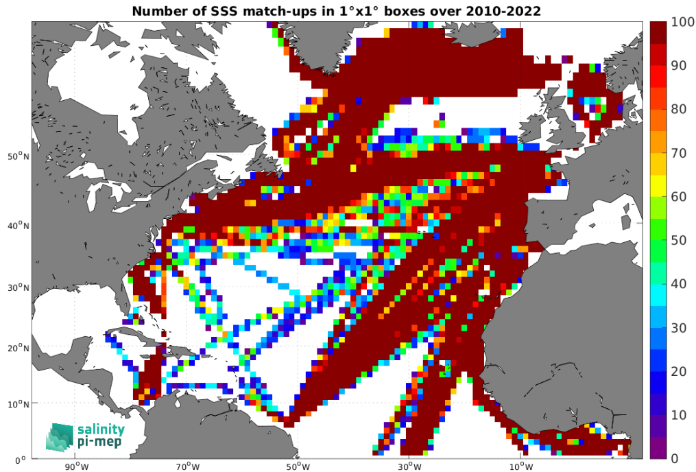
Figure 4: Number of SSS match-ups between TSG (LEGOS-DM) SSS and the CCI SSS L4 Merged-OI v4.4 - 7-day running (ESA) SSS product for the North Atlantic Ocean Pi-MEP region over 1^\circ \times 1^\circ boxes and for the full satellite product period.
