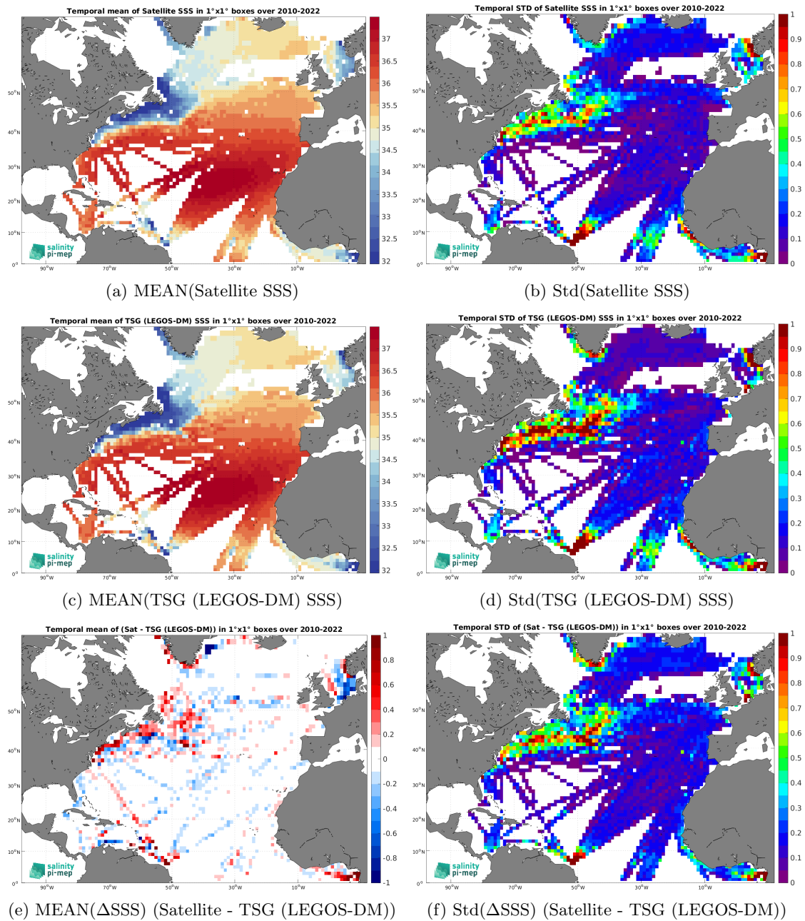
Figure 6: Temporal mean (left) and Std (right) of SSS from CCI SSS L4 Merged-OI v4.4 - 7-day running (ESA) (top), TSG (LEGOS-DM) (middle), and of \Delta SSS (Satellite - TSG (LEGOS-DM)). Only match-up pairs are used to generate these maps.
