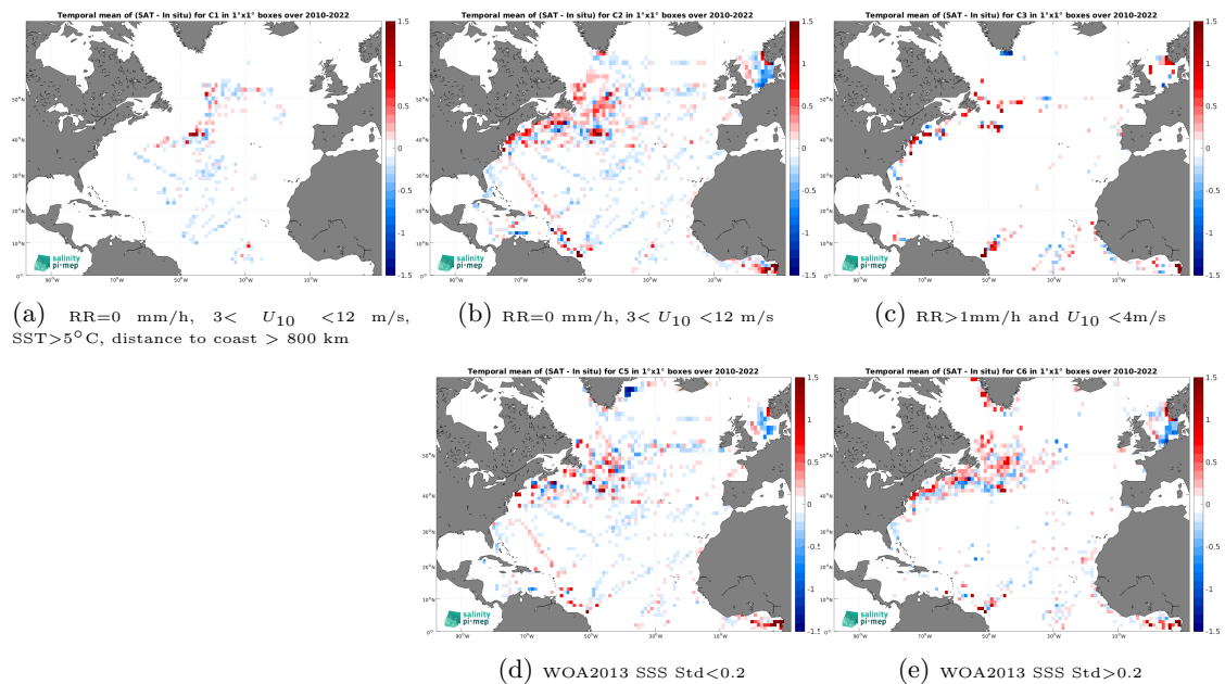
Figure 12: Temporal mean gridded over spatial boxes of size 1^\circ \times 1^\circ of \Delta\text{SSS} (CCI SSS L4 Merged-OI v4.4 - 7-day running (ESA) - TSG (LEGOS-DM)) for 5 different subdatasets corresponding to:RR=0 mm/h, 3 < U_{10} < 12 m/s, SST >5^\circ\text{C} , distance to coast > 800 km (a), RR=0 mm/h, 3 < U_{10} < 12 m/s (b), RR >1 mm/h and U_{10} < 4 m/s (c), WOA2013 SSS Std <0.2 (d), WOA2013 SSS Std >0.2 (e).
