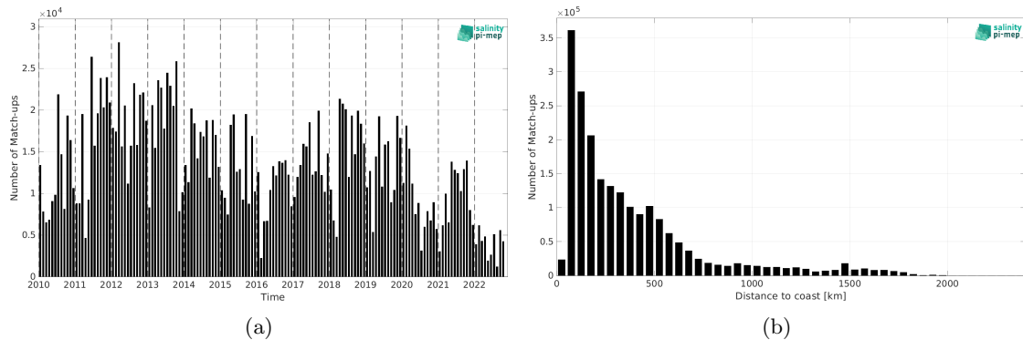
Figure 1: Number of match-ups between TSG (LEGOS-DM) and CCI SSS L4 Merged-OI v4.4 - 7-day running (ESA) SSS as a function of time (a) and as function of the distance to coast (b) over the North Atlantic Ocean Pi-MEP region and for the full satellite product period.
