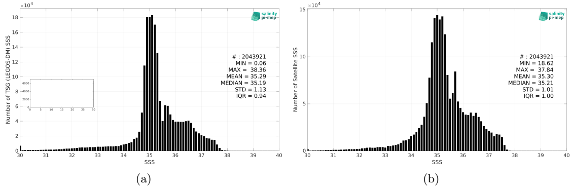
Figure 2: Histograms of SSS from TSG (LEGOS-DM) (a) and CCI SSS L4 Merged-OI v4.4 - 7-day running (ESA) (b) considering all match-up pairs per bins of 0.1 over the North Atlantic Ocean Pi-MEP region and for the full satellite product period.
