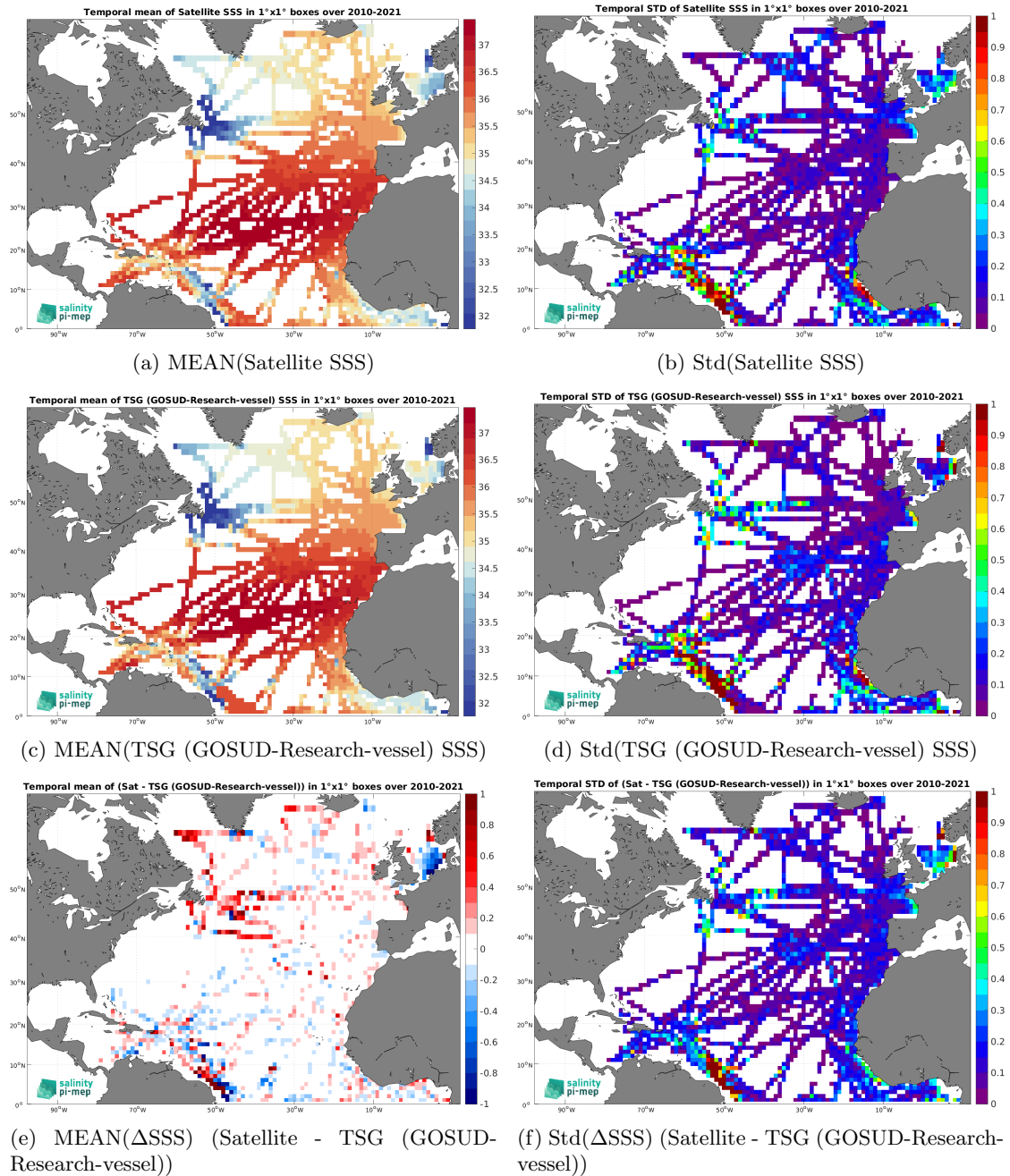
Figure 6: Temporal mean (left) and Std (right) of SSS from CCI SSS L4 Merged-OI v4.4 - 7-day running (ESA) (top), TSG (GOSUD-Research-vessel) (middle), and of \Delta SSS (Satellite - TSG (GOSUD-Research-vessel)). Only match-up pairs are used to generate these maps.
