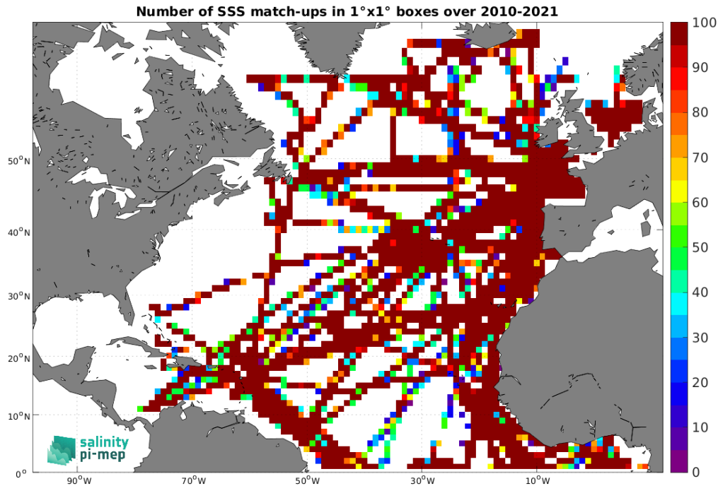
Figure 4: Number of SSS match-ups between TSG (GOSUD-Research-vessel) SSS and the CCI SSS L4 Merged-OI v4.4 - 7-day running (ESA) SSS product for the North Atlantic Ocean Pi-MEP region over 1^\circ \times 1^\circ boxes and for the full satellite product period.
