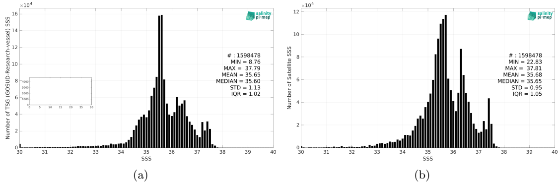
Figure 2: Histograms of SSS from TSG (GOSUD-Research-vessel) (a) and CCI SSS L4 Merged-OI v4.4 - 7-day running (ESA) (b) considering all match-up pairs per bins of 0.1 over the North Atlantic Ocean Pi-MEP region and for the full satellite product period.
