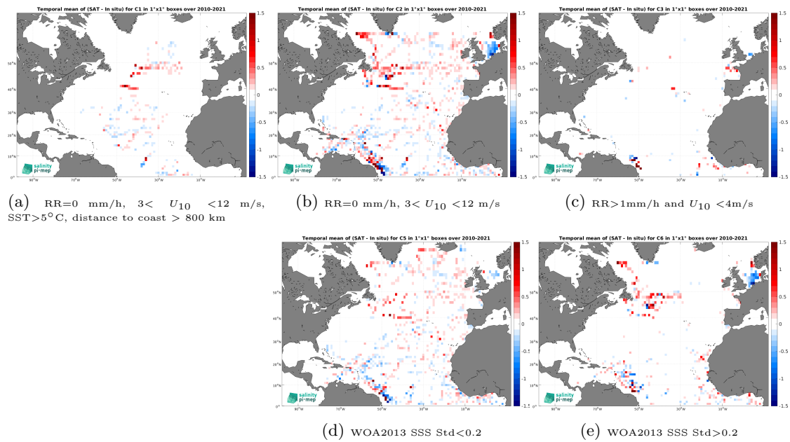
Figure 12: Temporal mean gridded over spatial boxes of size 1^\circ \times 1^\circ of \Delta\text{SSS} (CCI SSS L4 Merged-OI v4.4 - 7-day running (ESA) - TSG (GOSUD-Research-vessel)) for 5 different subdatasets corresponding to:RR=0 mm/h, 3 < U_{10} < 12 m/s, SST >5^\circ\text{C} , distance to coast > 800 km (a), RR=0 mm/h, 3 < U_{10} < 12 m/s (b), RR >1 mm/h and U_{10} < 4 m/s (c), WOA2013 SSS Std <0.2 (d), WOA2013 SSS Std >0.2 (e).
