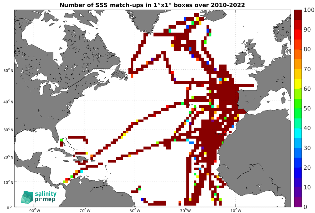
Figure 4: Number of SSS match-ups between TSG (CSIC-UTM) SSS and the CCI SSS L4 Merged-OI v4.4 - 7-day running (ESA) SSS product for the North Atlantic Ocean Pi-MEP region over 1^\circ \times 1^\circ boxes and for the full satellite product period.
