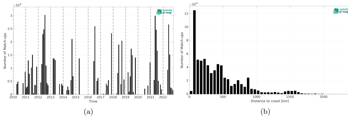
Figure 1: Number of match-ups between TSG (CSIC-UTM) and CCI SSS L4 Merged-OI v4.4 - 7-day running (ESA) SSS as a function of time (a) and as function of the distance to coast (b) over the North Atlantic Ocean Pi-MEP region and for the full satellite product period.
