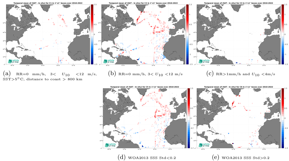
Figure 12: Temporal mean gridded over spatial boxes of size 1^\circ \times 1^\circ of \Delta\text{SSS} (CCI SSS L4 Merged-OI v4.4 - 7-day running (ESA) - TSG (CSIC-UTM)) for 5 different subdatasets corresponding to:RR=0 mm/h, 3 < U_{10} < 12 m/s, SST >5^\circ\text{C} , distance to coast > 800 km (a), RR=0 mm/h, 3 < U_{10} < 12 m/s (b), RR >1 mm/h and U_{10} < 4 m/s (c), WOA2013 SSS Std <0.2 (d), WOA2013 SSS Std >0.2 (e).
