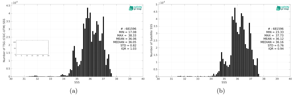
Figure 2: Histograms of SSS from TSG (CSIC-UTM) (a) and CCI SSS L4 Merged-OI v4.4 - 7-day running (ESA) (b) considering all match-up pairs per bins of 0.1 over the North Atlantic Ocean Pi-MEP region and for the full satellite product period.
