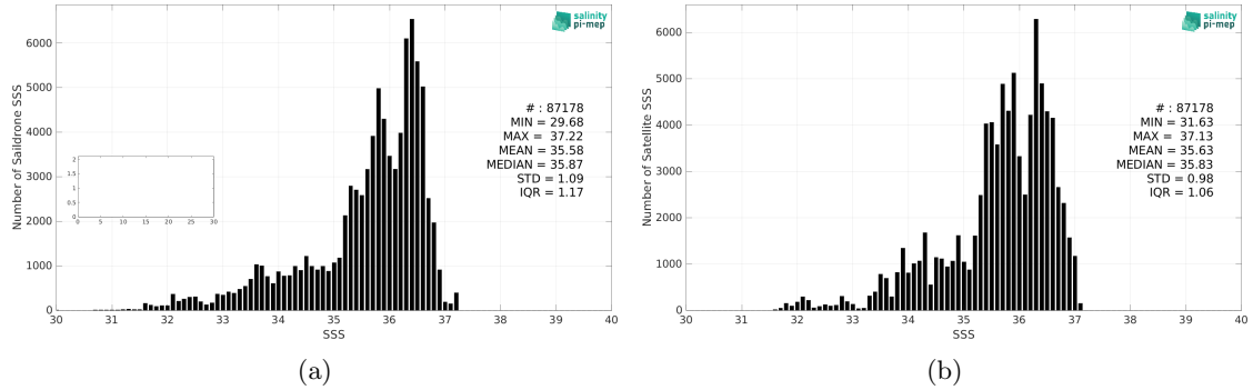
Figure 2: Histograms of SSS from Saildrone (a) and CCI SSS L4 Merged-OI v4.4 - 7-day running (ESA) (b) considering all match-up pairs per bins of 0.1 over the North Atlantic Ocean Pi-MEP region and for the full satellite product period.
