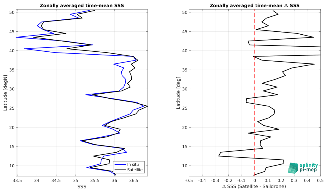
Figure 8: Left panel: Zonal mean SSS from CCI SSS L4 Merged-OI v4.4 - 7-day running (ESA) satellite product (black) and from Saildrone (blue). Right panel: Zonal mean of \Delta SSS (Satellite - Saildrone) for all the collected Pi-MEP match-up pairs estimated over the full satellite product period.
