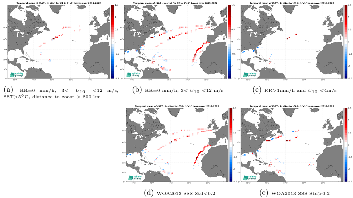
Figure 12: Temporal mean gridded over spatial boxes of size 1^\circ \times 1^\circ of \Delta\text{SSS} (CCI SSS L4 Merged-OI v4.4 - 7-day running (ESA) - Saildrone) for 5 different subdatasets corresponding to:RR=0 mm/h, 3 < U_{10} < 12 m/s, SST >5^\circ\text{C} , distance to coast > 800 km (a), RR=0 mm/h, 3 < U_{10} < 12 m/s (b), RR >1 mm/h and U_{10} < 4 m/s (c), WOA2013 SSS Std <0.2 (d), WOA2013 SSS Std >0.2 (e).
