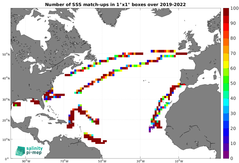
Figure 4: Number of SSS match-ups between Saildrone SSS and the CCI SSS L4 Merged-OI v4.4 - 7-day running (ESA) SSS product for the North Atlantic Ocean Pi-MEP region over 1^\circ \times 1^\circ boxes and for the full satellite product period.
