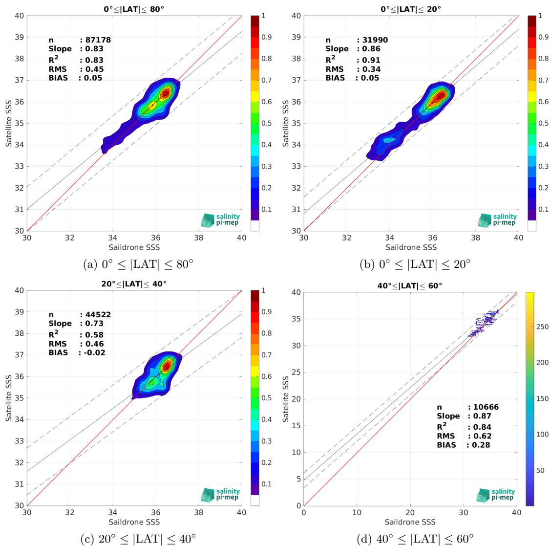
Figure 9: Contour maps of the concentration of CCI SSS L4 Merged-OI v4.4 - 7-day running (ESA) SSS (y-axis) versus Saldrone SSS (x-axis) at match-up pairs for different latitude bands. For each plot, the red line shows x=y . The black thin and dashed lines indicate a linear fit through the data cloud and the \pm 95\% confidence levels, respectively. The number match-up pairs n , the slope and R^2 coefficient of the linear fit, the root mean square (RMS) and the mean bias between satellite and in situ data are indicated for each latitude band in each plots.
