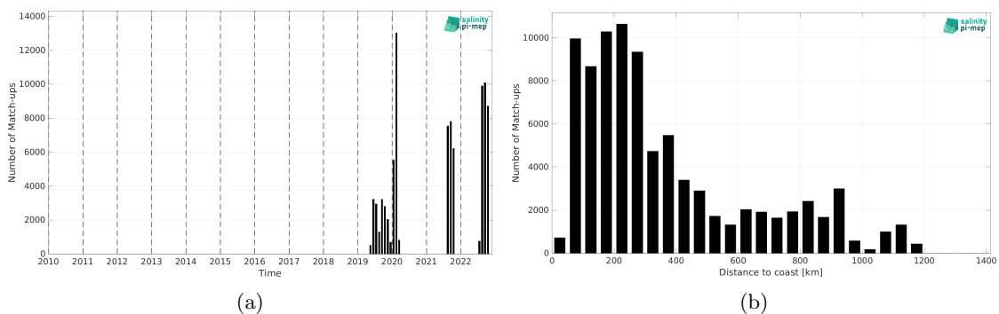
Figure 1: Number of match-ups between Saildrone and CCI SSS L4 Merged-OI v4.4 - 7-day running (ESA) SSS as a function of time (a) and as function of the distance to coast (b) over the North Atlantic Ocean Pi-MEP region and for the full satellite product period.
