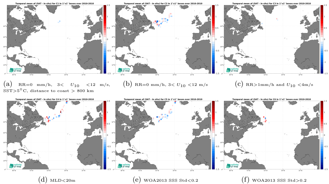
Figure 12: Temporal mean gridded over spatial boxes of size 1^{\circ}\times 1^{\circ} of \Delta\text{SSS} (CCI SSS L4 Merged-OI v4.4 - 7-day running (ESA) - Marine mammals) for 6 different subdatasets corresponding to:RR=0 mm/h, 3 < U_{10} < 12 m/s, SST >5^{\circ}\text{C} , distance to coast > 800 km (a), RR=0 mm/h, 3 < U_{10} < 12 m/s (b), RR >1\text{mm/h} and U_{10} < 4\text{m/s} (c),MLD <20\text{m} (d),WOA2013 SSS Std <0.2 (e),WOA2013 SSS Std >0.2 (f).
