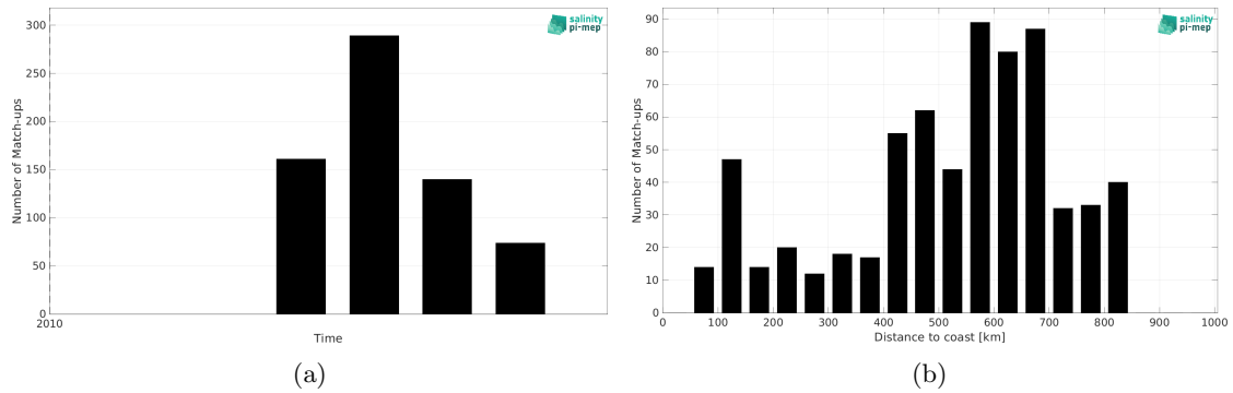
Figure 1: Number of match-ups between Marine mammals and CCI SSS L4 Merged-OI v4.4 - 7-day running (ESA) SSS as a function of time (a) and as function of the distance to coast (b) over the North Atlantic Ocean Pi-MEP region and for the full satellite product period.
