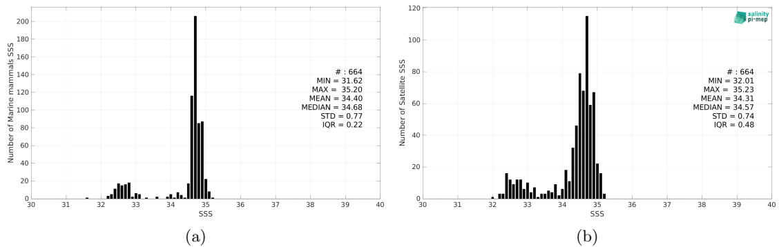
Figure 2: Histograms of SSS from Marine mammals (a) and CCI SSS L4 Merged-OI v4.4 - 7-day running (ESA) (b) considering all match-up pairs per bins of 0.1 over the North Atlantic Ocean Pi-MEP region and for the full satellite product period.
