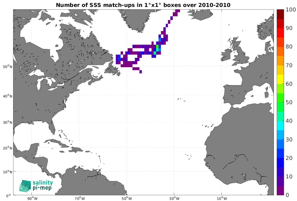
Figure 4: Number of SSS match-ups between Marine mammals SSS and the CCI SSS L4 Merged-OI v4.4 - 7-day running (ESA) SSS product for the North Atlantic Ocean Pi-MEP region over 1^\circ \times 1^\circ boxes and for the full satellite product period.
