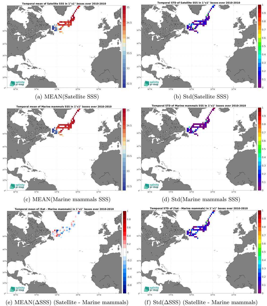
Figure 6: Temporal mean (left) and Std (right) of SSS from CCI SSS L4 Merged-OI v4.4 - 7-day running (ESA) (top), Marine mammals (middle), and of \Delta SSS (Satellite - Marine mammals). Only match-up pairs are used to generate these maps.
