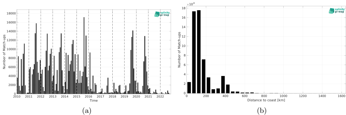
Figure 1: Number of match-ups between ICES and CCI SSS L4 Merged-OI v4.4 - 7-day running (ESA) SSS as a function of time (a) and as function of the distance to coast (b) over the North Atlantic Ocean Pi-MEP region and for the full satellite product period.
