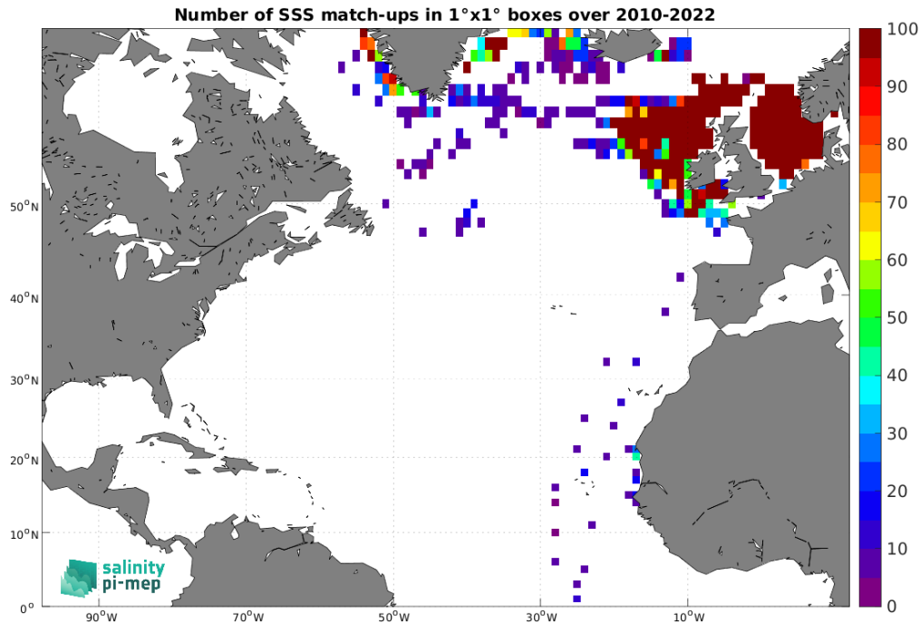
Figure 4: Number of SSS match-ups between ICES SSS and the CCI SSS L4 Merged-OI v4.4 - 7-day running (ESA) SSS product for the North Atlantic Ocean Pi-MEP region over 1^\circ \times 1^\circ boxes and for the full satellite product period.
