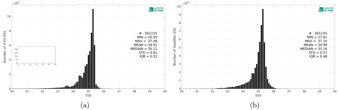
Figure 2: Histograms of SSS from ICES (a) and CCI SSS L4 Merged-OI v4.4 - 7-day running (ESA) (b) considering all match-up pairs per bins of 0.1 over the North Atlantic Ocean Pi-MEP region and for the full satellite product period.
