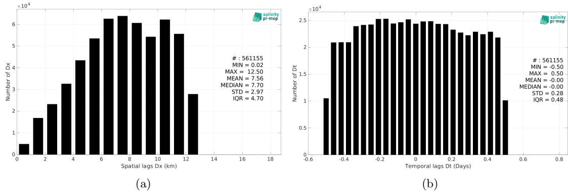
Figure 5: Histograms of the spatial (a) and temporal (b) lags between the location/time of the ICES measurement and the date of the corresponding CCI SSS L4 Merged-OI v4.4 - 7-day running (ESA) SSS pixel.
