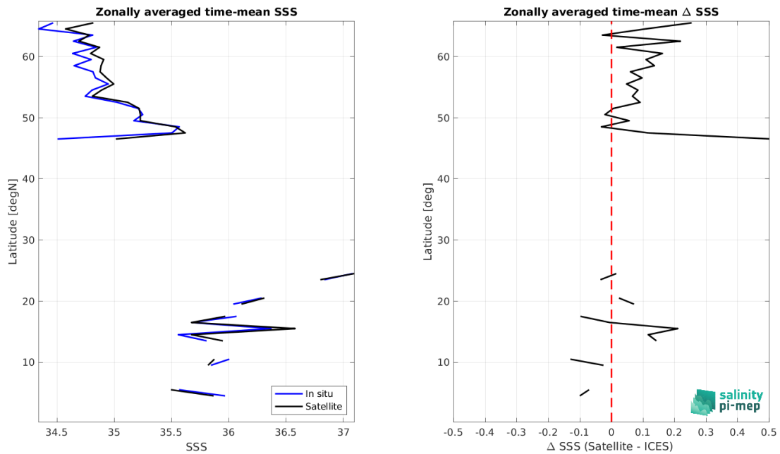
Figure 8: Left panel: Zonal mean SSS from CCI SSS L4 Merged-OI v4.4 - 7-day running (ESA) satellite product (black) and from ICES (blue). Right panel: Zonal mean of \Delta SSS (Satellite - ICES) for all the collected Pi-MEP match-up pairs estimated over the full satellite product period.
