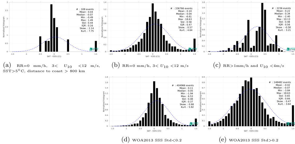
Figure 13: Normalized histogram of \Delta SSS (CCI SSS L4 Merged-OI v4.4 - 7-day running (ESA) - ICES) for 5 different subdatasets corresponding to: RR=0 mm/h, 3 < U_{10} < 12 m/s, SST > 5°C, distance to coast > 800 km (a), RR=0 mm/h, 3 < U_{10} < 12 m/s (b), RR > 1mm/h and U_{10} < 4 m/s (c), WOA2013 SSS Std < 0.2 (d), WOA2013 SSS Std > 0.2 (e).
