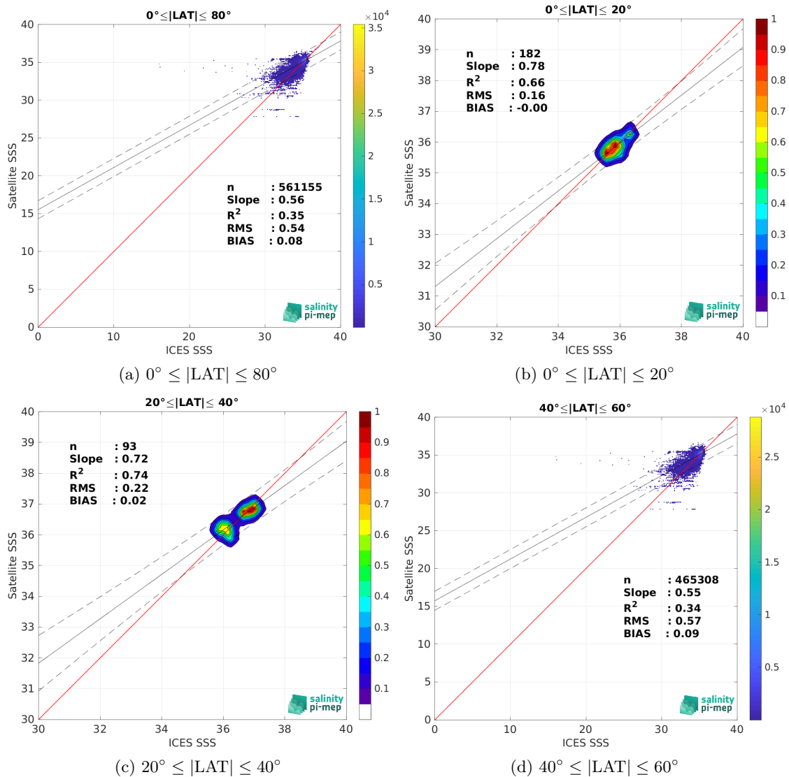
Figure 9: Contour maps of the concentration of CCI SSS L4 Merged-OI v4.4 - 7-day running (ESA) SSS (y-axis) versus ICES SSS (x-axis) at match-up pairs for different latitude bands. For each plot, the red line shows x=y . The black thin and dashed lines indicate a linear fit through the data cloud and the \pm 95\% confidence levels, respectively. The number match-up pairs n , the slope and R^2 coefficient of the linear fit, the root mean square (RMS) and the mean bias between satellite and in situ data are indicated for each latitude band in each plots.
