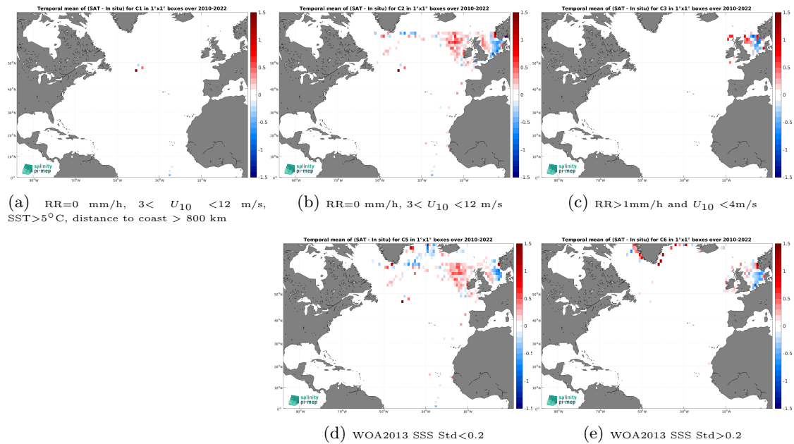
Figure 12: Temporal mean gridded over spatial boxes of size 1^\circ \times 1^\circ of \Delta\text{SSS} (CCI SSS L4 Merged-OI v4.4 - 7-day running (ESA) - ICES) for 5 different subdatasets corresponding to:RR=0 mm/h, 3 < U_{10} < 12 m/s, SST >5^\circ\text{C} , distance to coast > 800 km (a), RR=0 mm/h, 3 < U_{10} < 12 m/s (b), RR >1 mm/h and U_{10} < 4 m/s (c), WOA2013 SSS Std <0.2 (d), WOA2013 SSS Std >0.2 (e).
