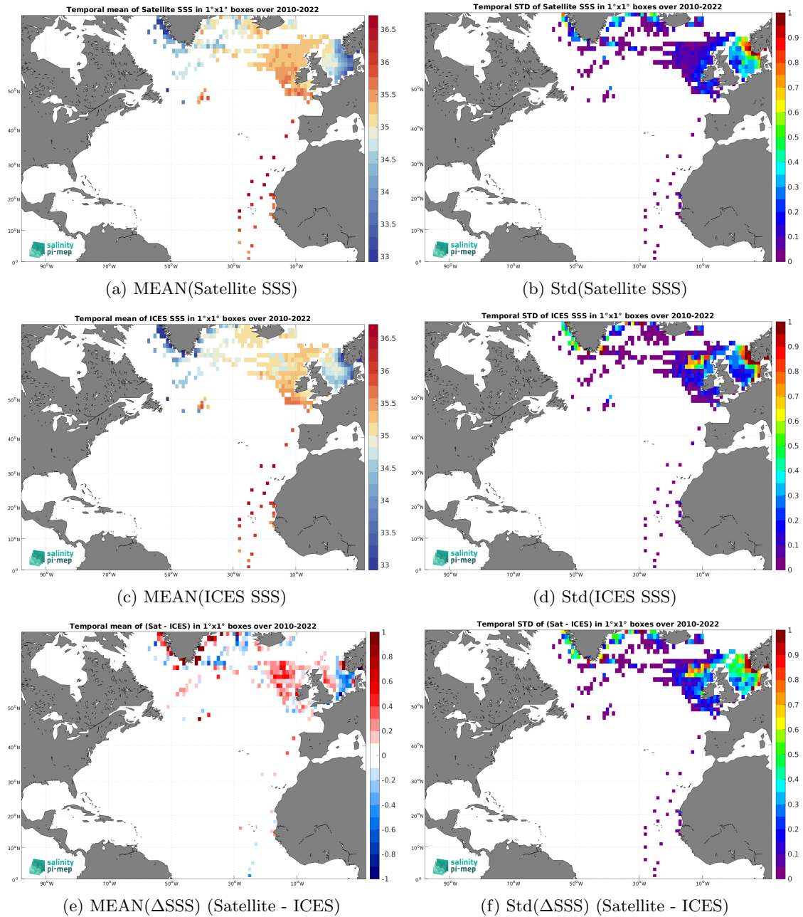
Figure 6: Temporal mean (left) and Std (right) of SSS from CCI SSS L4 Merged-OI v4.4 - 7-day running (ESA) (top), ICES (middle), and of \Delta SSS (Satellite - ICES). Only match-up pairs are used to generate these maps.
