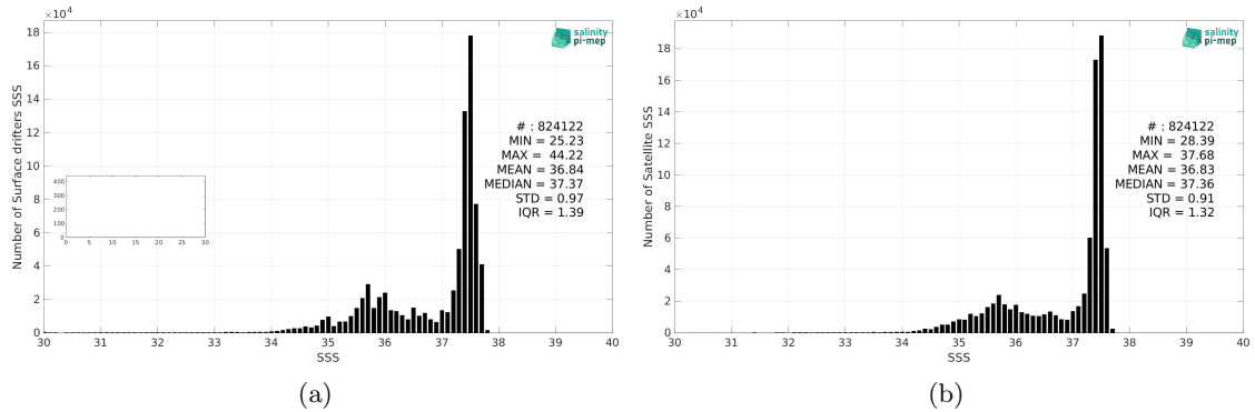
Figure 2: Histograms of SSS from Surface drifters (a) and CCI SSS L4 Merged-OI v4.4 - 7-day running (ESA) (b) considering all match-up pairs per bins of 0.1 over the North Atlantic Ocean Pi-MEP region and for the full satellite product period.
