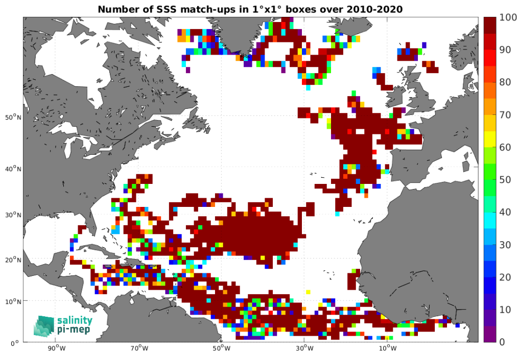
Figure 3: Number of SSS match-ups between Surface drifters SSS and the CCI SSS L4 Merged-OI v4.4 - 7-day running (ESA) SSS product for the North Atlantic Ocean Pi-MEP region over 1^\circ \times 1^\circ boxes and for the full satellite product period.
