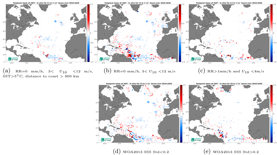
Figure 11: Temporal mean gridded over spatial boxes of size 1^\circ \times 1^\circ of \Delta\text{SSS} (CCI SSS L4 Merged-OI v4.4 - 7-day running (ESA) - Surface drifters) for 5 different subdatasets corresponding to:RR=0 mm/h, 3 < U_{10} < 12 m/s, SST >5^\circ\text{C} , distance to coast > 800 km (a), RR=0 mm/h, 3 < U_{10} < 12 m/s (b), RR >1 mm/h and U_{10} < 4 m/s (c), WOA2013 SSS Std <0.2 (d), WOA2013 SSS Std >0.2 (e).
